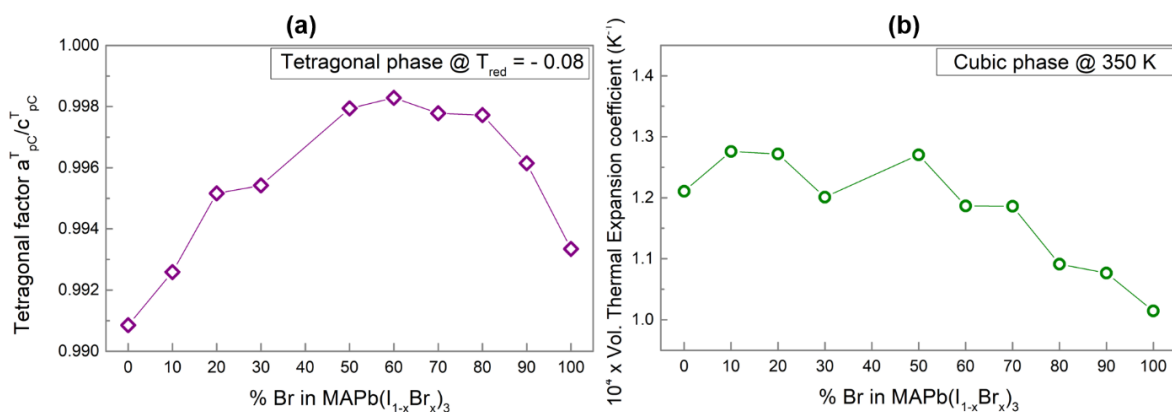
Figure 5.10: (a) Tetragonal factor of \text{MAPb}(\text{I}_{1-x}\text{Br}_x)_3 ( x = 0 to 100 % Br) compounds in the I4/mcm symmetry, calculated at T_{\text{red}} = - 0.08 . (b) Evolution of the volumetric thermal expansion coefficient of the cubic phase of \text{MAPb}(\text{I}_{1-x}\text{Br}_x)_3 ( x = 0 to 100 % Br) at 350 K.
