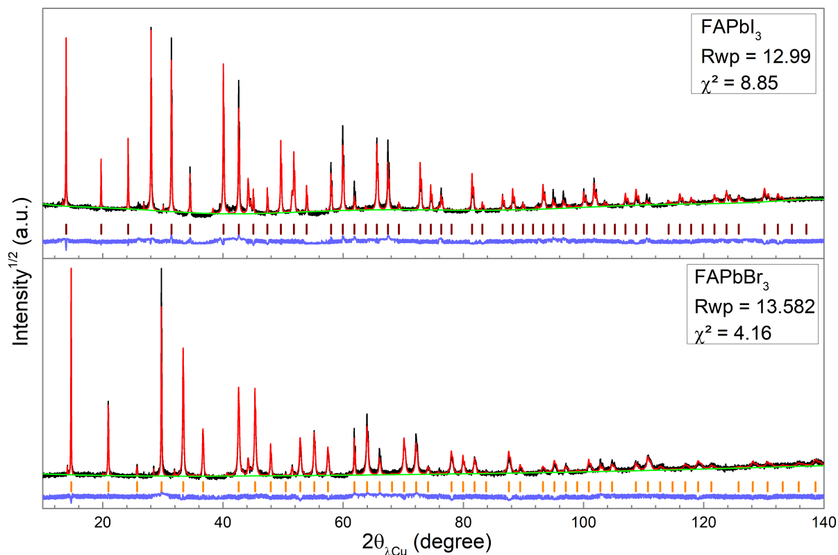
Figure 4.12: Example of Rietveld refinements for \text{FAPbI}_3 (top panel) and \text{FAPbBr}_3 (bottom panel), showing the poor quality of the refinement for both samples. In both panels, the black line is the measured pattern Y_{\text{obs}} , the red line is the refined pattern Y_{\text{calc}} , the green line is the refined background and the blue one is the difference Y_{\text{obs}} - Y_{\text{calc}} . The colored dashes represent the expected diffraction lines of the cubic \text{Pm-3m} phase.
