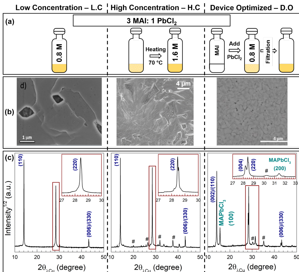
Figure I.15: Presentation of the three different layers used in this study: Low Concentration (L.C.), High Concentration (H.C) and Device optimized (D.O.). (a) Protocol of preparation of the precursor's solution. (b) SEM images of the three different layers. (c) Typical \theta - 2\theta diffractogram of the three types of layers, with, in red, an enlarged view of the region identified by in the red square in the main pattern. # sign indicated the peaks of the substrate, FTO/ \text{TiO}_2 or ITO/ \text{TiO}_2 .
