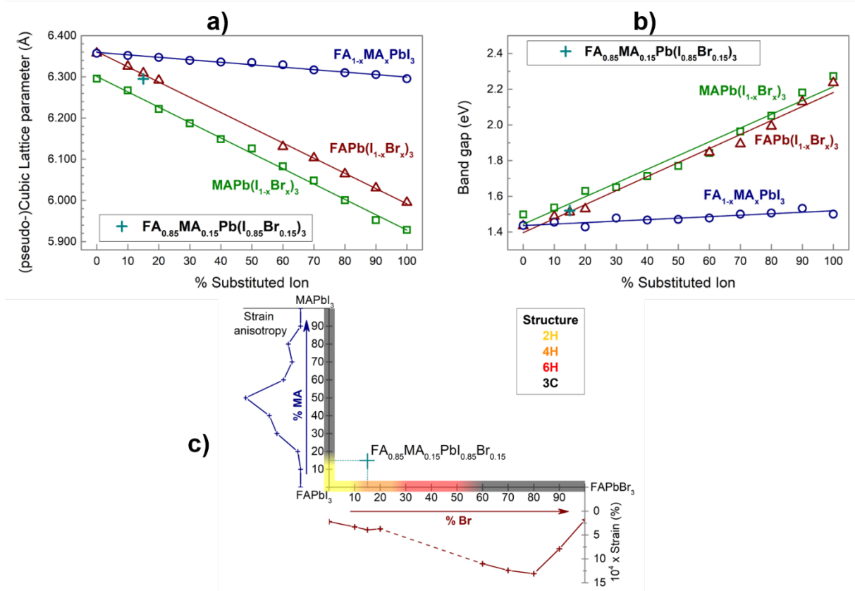
Figure 4.37: Evolution of (a) (pseudo-)cubic lattice parameter and (b) band gap upon ion substitution in the three solid solution families investigated here: \text{MAPb}(\text{I}_{1-x}\text{Br}_x)_3 , \text{FAPb}(\text{I}_{1-x}\text{Br}_x)_3 and \text{FA}_{1-x}\text{MA}_x\text{PbI}_3 . The blue cross in both panels represent the parameters evaluated for the quinary mixed organic cation/mixed halide compound studied. (c) schematic representation of the polymorphic behavior of FA-based compounds, as extracted from the previous sections, and the mixed cation mixed halide compound is positioned on this map.
