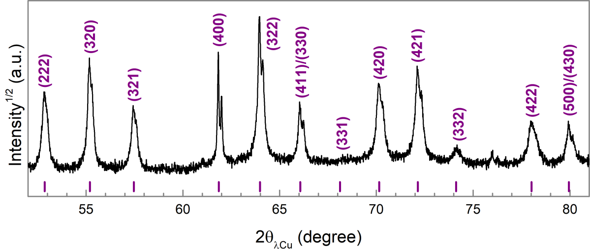
Figure 4.9: Raw DRX pattern of \text{FAPbBr}_3 powder. The purple sticks indicate the expected cubic Pm-3m perovskite peaks for a lattice parameter of a = 5.995(2) \text{ \AA} , matching the observed lines.
