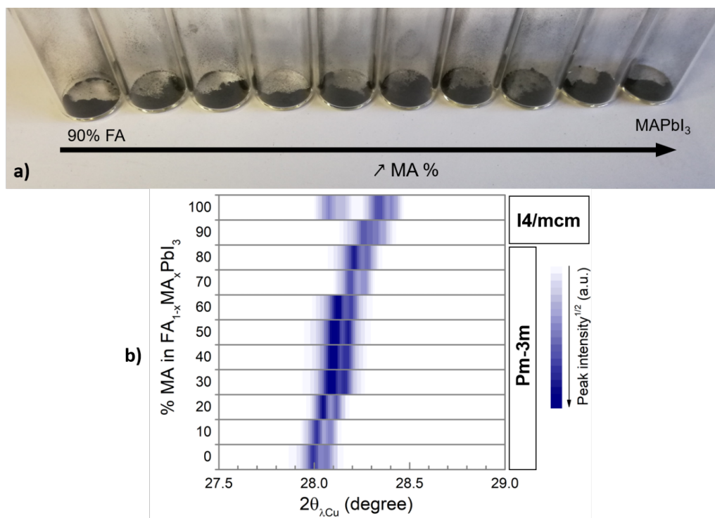
Figure 4.31: (a) Picture of the FA 1-x MA x PbI 3 solid solutions family. The sample remain black over the whole compositional range. (b) Evolution of the (200) cubic Pm-3m Bragg peak, showing a gradual shift of the peak position to higher angles, indicated a shirking in the lattice parameters. Note the small range of variation of the peak position (1.5 °) in comparison with the two previous families (3°). Furthermore, note that both 90 and 100 % MA + containing samples exhibit a tetragonal symmetry at RT
