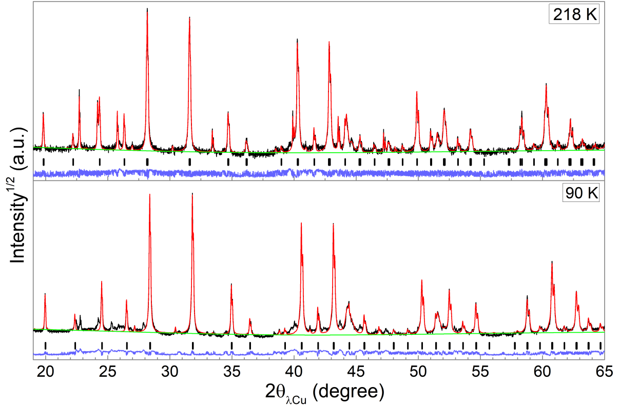
Figure 5.13: LeBail refinement of XRD pattern of \text{FAPbI}_3 measured at 218 (top panel) and 90 K (bottom panel), using, for both, \text{P4}/\text{mbm} space group. While the refinement matched all observed lines at 218 K, additional peaks at 90 K are not met by the \text{P4}/\text{mbm} space group.
