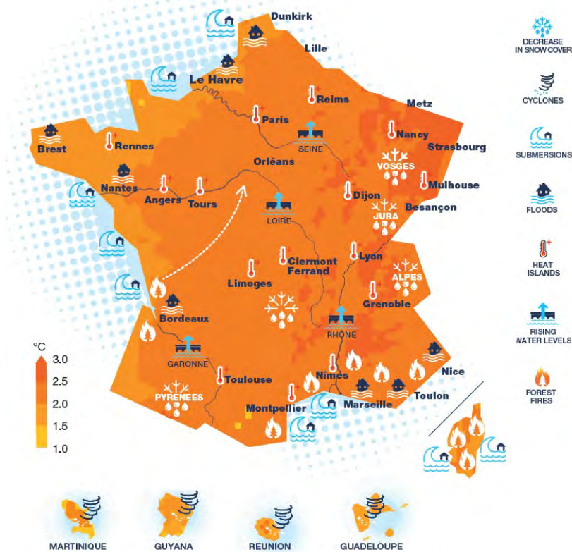
Fig. 1.2 Actual or expected by 2050 impacts of climate change in the case of France.
