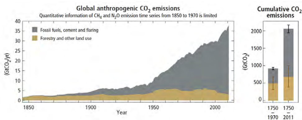
Fig. 1.1 Trend of annual global anthropogenic CO 2 emissions. Cumulative CO 2 emissions are presented on the right-hand side (uncertainties are shown as whiskers).
