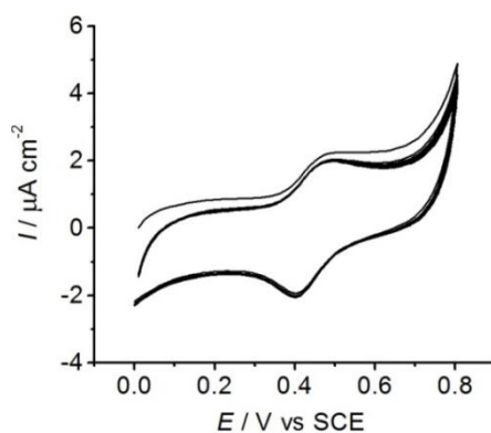
Figure 5.7 Ten consecutive CVs recorded of as-prepared aqueous PSCD-P2ABTS NP solution at GCE (pH = 5.6) at 100 \text{ mV s}^{-1} .
