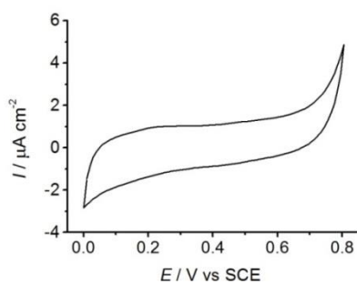
Figure 5.6 CV recorded at a GCE in 0.1 \text{ mol L}^{-1} PB pH 7 at 100 \text{ mV s}^{-1} to test for the presence of adsorbed species after performing a scan rate study in as-prepared aqueous PSCD-P2ABTS NP solution (ca. 15 potential cycles from 0 V to 0.8 V) then rinsing the electrode with 0.1 \text{ mol L}^{-1} PB pH 7.
