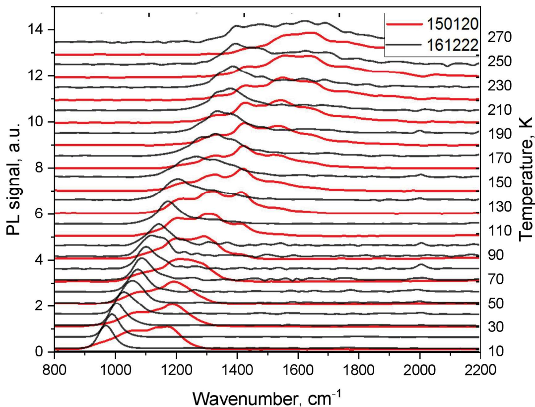
Fig. 43. Temperature dependence of the PL spectra of structures 150120 and 161222. The spectra were measured under continuous wave 800 nm pumping. The right
