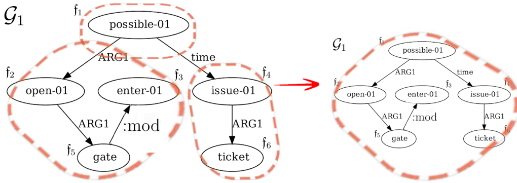
FIGURE 4.14 – Application du schéma s_2 = (req_2, tr_2)
