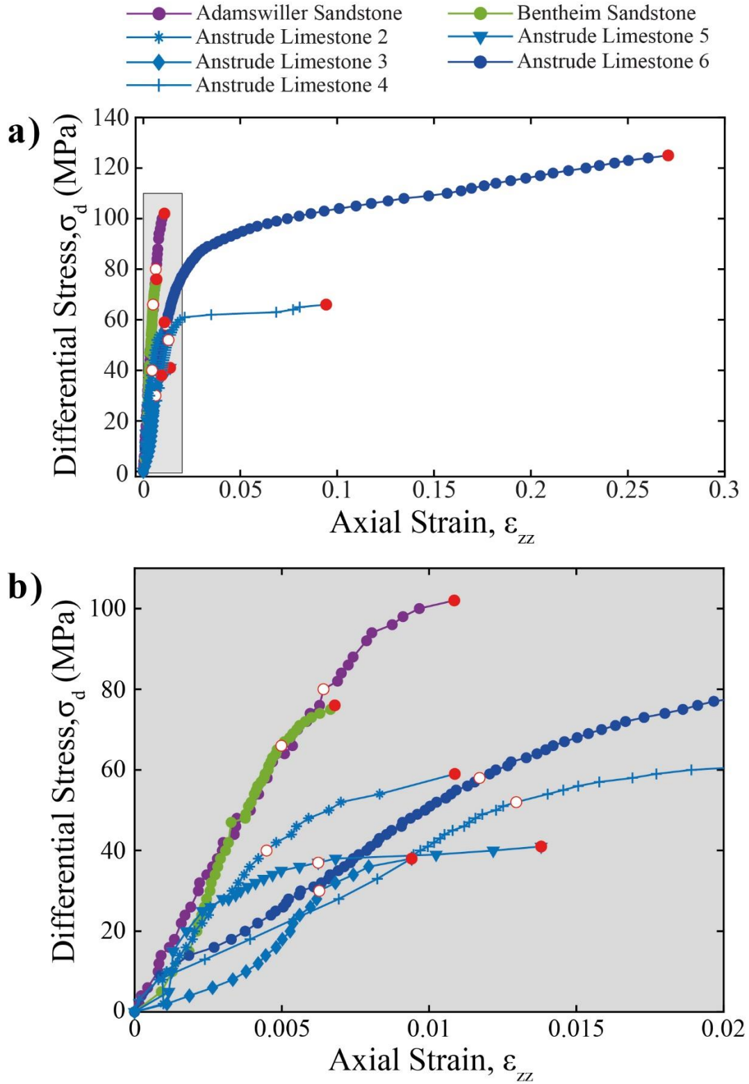
Figure 1. Relationships between differential stress and axial strain in seven experiments on porous rocks: Adamswiller sandstone, Bentheim sandstone, and Anstrude limestone (2, 3, 4, 5, 6). Table 2 shows the
