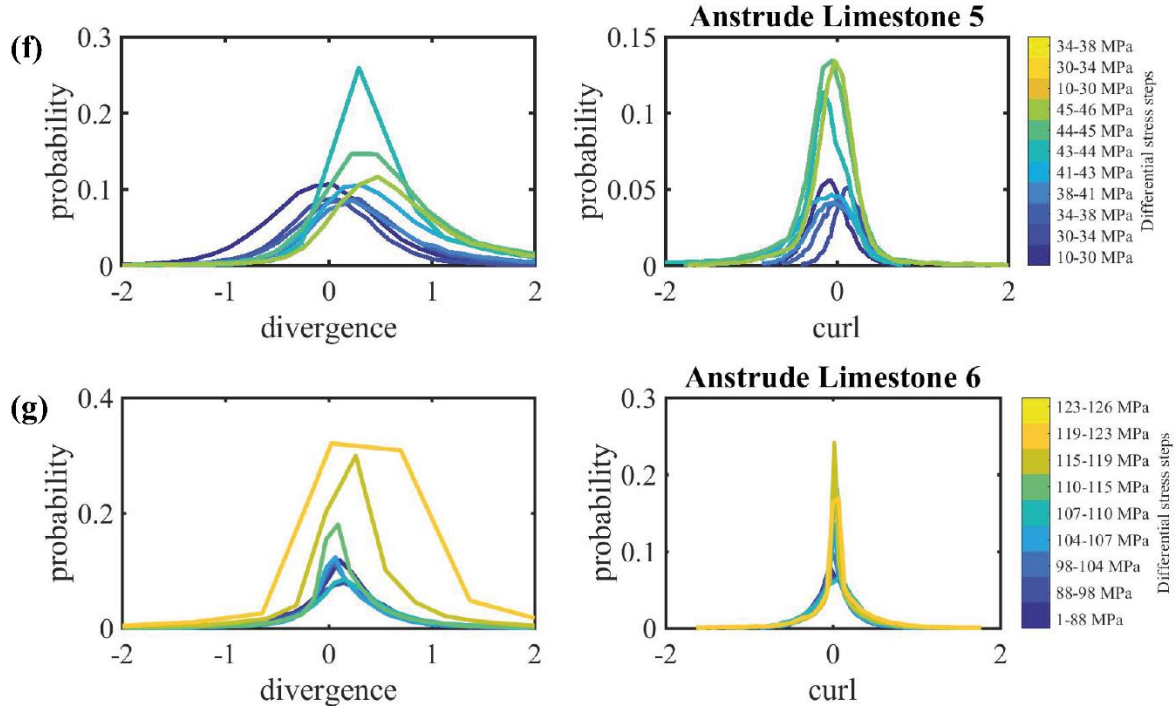
Figure S3. Histograms of divergence and curl of the incremental displacement fields ( \vec{u} ) computed from DVC analysis with 20 voxel node spacing for the Adamswiller sandstone (a), Bentheim sandstone (b), Anstrude limestone 2 (c), Anstrude limestone 3 (d), Anstrude limestone 4 (e), Anstrude limestone 5 (f) and Anstrude limestone 6 (g). Color scale from blue to yellow for each experiment represents the successive experimental increments and corresponds to the differential stress for the pair of tomograms chosen for DVC analysis. Tomograms at nearly equal strain increments are chosen for DVC analysis as given in supplementary Figure S2.
