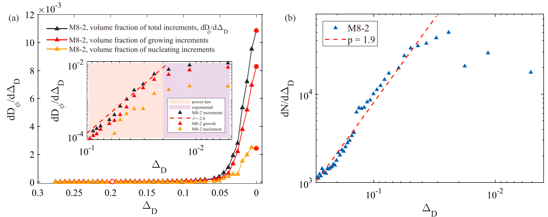
Figure 7. (a) Evolution of incremental damage, dD_\phi/d\Delta_D as a function of control parameter, \Delta_D in sample M8-2. Damage increments are tracked as incremental events of growth and nucleation (see Figure 1), and the respective volume fractions are plotted as a function of \Delta_D . Inset: Rate of damage growth and nucleation plotted against control parameter for sample M8-2, showing a scaling dD_\phi/d\Delta_D \sim \Delta_D^{-\beta} with an exponent \beta = 2.6 for 0.02 < \Delta_D < 0.1 (red dashed straight line). For \Delta_D < 0.02 , an exponential evolution is observed. Open red circle shows the yield point; full red circle shows the last scan acquired before failure. (b) Number of damage increments (damage event rate), dN/d\Delta_D plotted as a function of control parameter, \Delta_D , shows a power law scaling, dN/d\Delta_D \sim \Delta_D^{-p} with exponent p = 1.9 \pm 0.06 for \Delta_D > 0.02 and a fluctuating decrease for \Delta_D < 0.02 .
