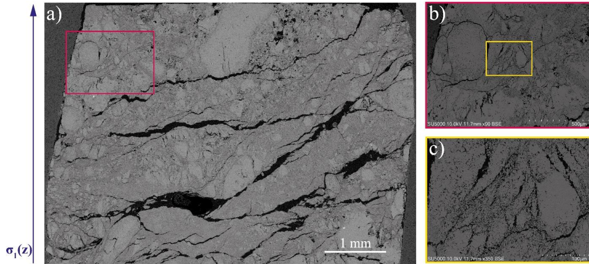
Figure S5. Scanning electron micrograph of the Anstrude limestone 2 showing the microstructure after a brittle compressive failure. a) Whole width of the sample. b-c) Magnified images of highlighted areas in a) and b) respectively. All images show grain crushing and in a-b) transgranular fractures are observed.
