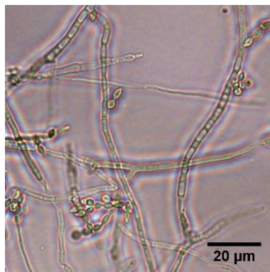
Fig. IV.7 : Mycelium of T. helicus incubated in mineral medium, after 30 min to 48 h of contact with BaP. Observations in bright field (top row) and epi-fluorescence microscopy with a DAPI excitation filter (bottom row)
