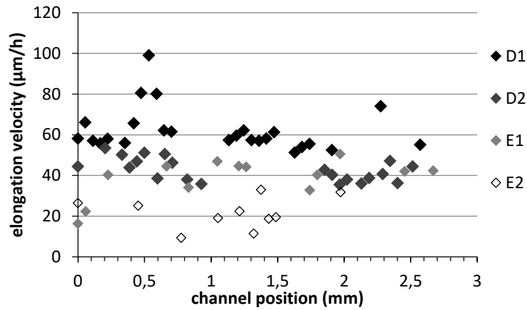
Fig. III.12: hyphal elongation velocity in individual channels depending on their relative position, in dynamic conditions (with x=0 corresponding to the position of the channel closest to the perfusion inlet)
