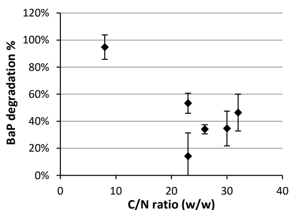
Fig. I.4: BaP degradation by T. helicus in exp. A and B expressed as a percentage of the quantity recovered in control flasks, depending on the C/N ratio of the medium
