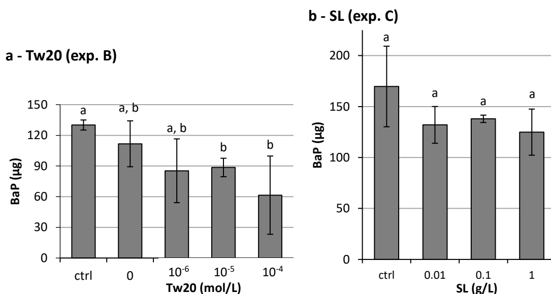
Fig. I.6 : Residual BaP mass after 9 days of incubation in control flasks vs flasks inoculated with T. helicus in 10 mL of mineral medium supplemented with surfactants : Tween 20 (Tw20) from 10 -6 to 10 -4 mol/L or Sophoclean (SL) from 10 -2 to 1 g/L. Groups of values that are not significantly different are indicated with the same letter.
