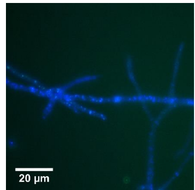
Fig. IV.7 : Mycelium of T. helicus incubated in mineral medium, after 30 min to 48 h of contact with BaP. Observations in bright field (top row) and epi-fluorescence microscopy with a DAPI excitation filter (bottom row)
