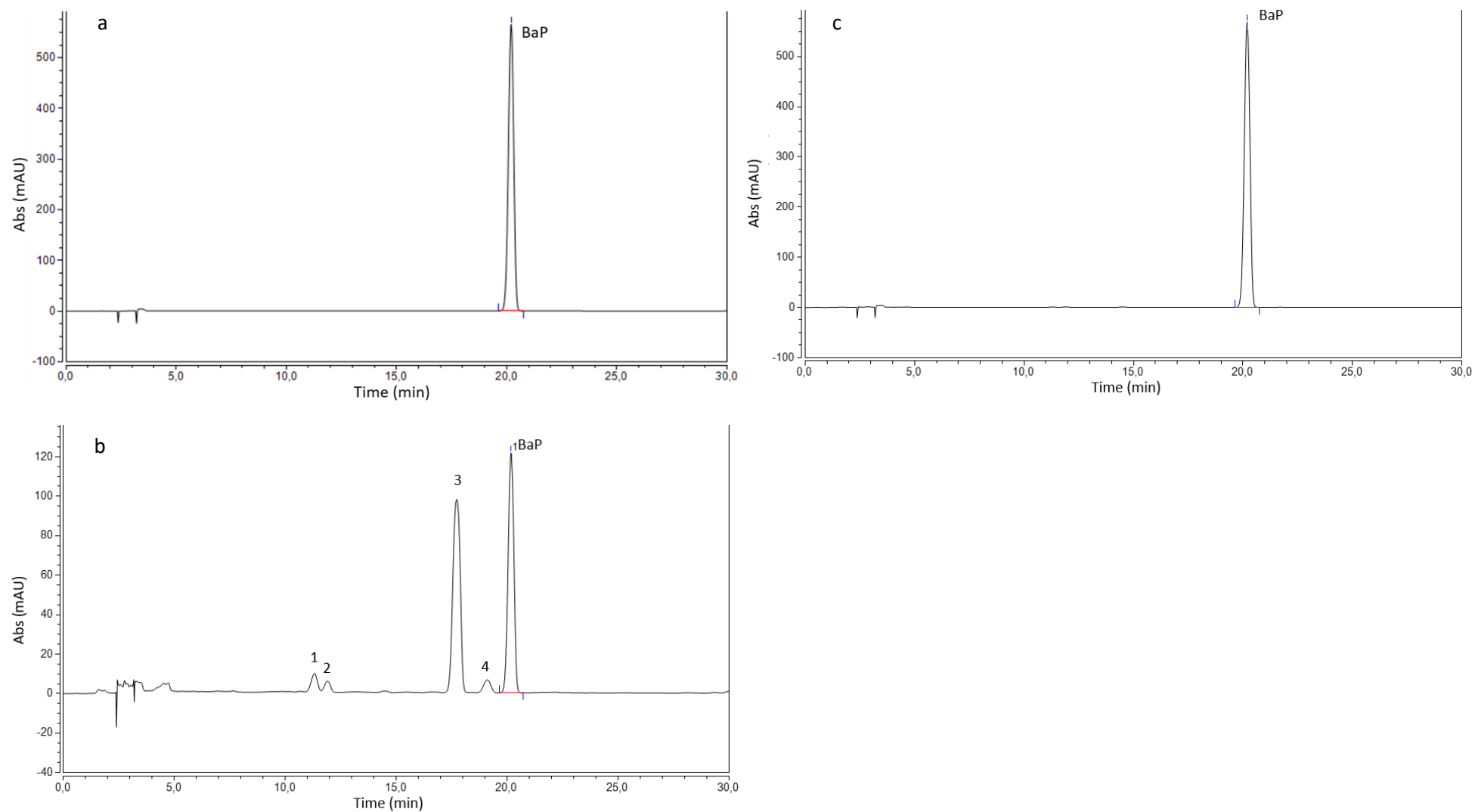
Fig. I.7: Chromatograms obtained after biodegradation in standard MM1 C/N=23 (a), in N-enriched MM1 C/N=8 (b), and for a pure BaP standard (c). BaP is detected as a peak at ~20.2 min.
