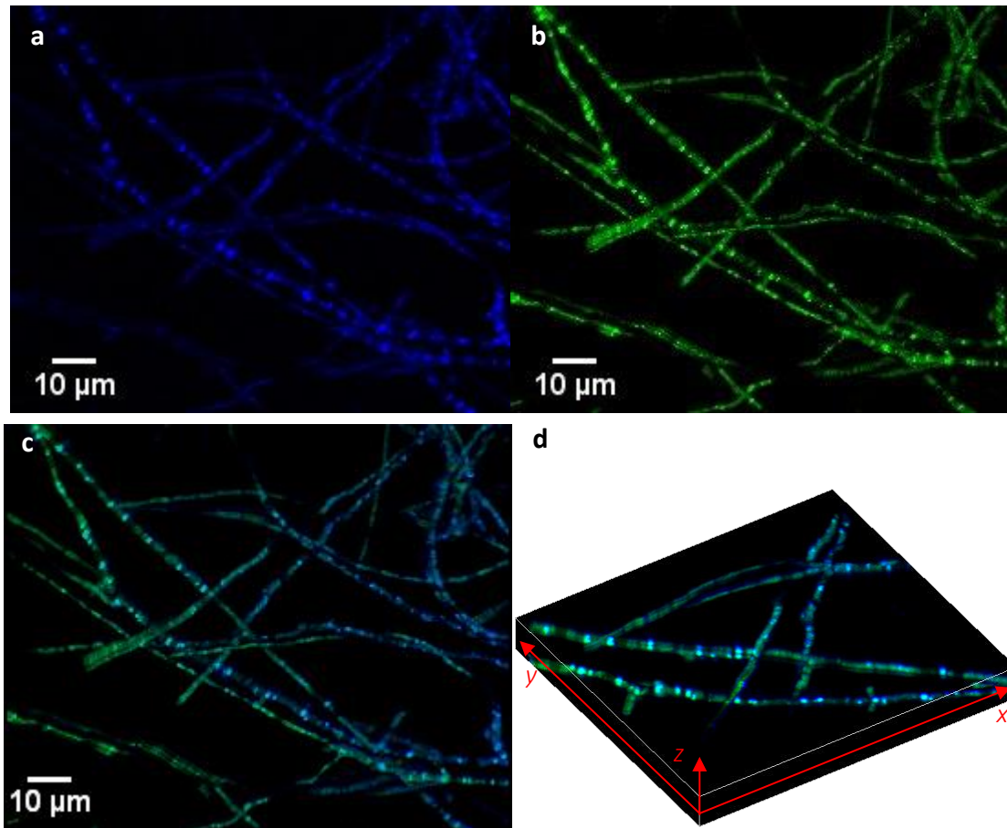
Fig. IV.5 : Mycelium of T. helicus incubated with BaP and stained with BODIPY, observed in confocal microscopy at 40 x magnification (maximum intensity projection of a 41 images stack with a 0.38 µm increment). BaP appears in blue and BODIPY in green. Structures stained with both fluorescent molecules appear in cyan shades. – a : DAPI filter – b: FITC filter – c: merged DAPI and FITC channels – d: 3D view of stained hyphae, dimensions 70 x 63 x 7 µm (x:y:z)
