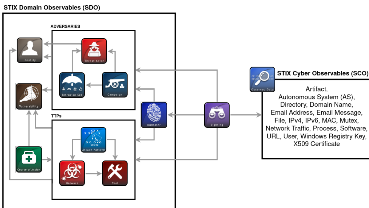
Figure 2.1 – STIXv2.0 Model
