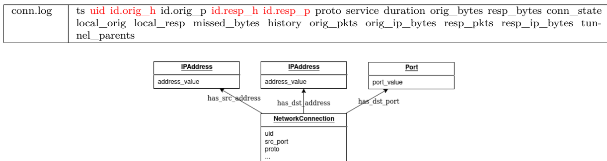
Figure 3.2 – Building a graph from one network connection as shown in the conn.log file
