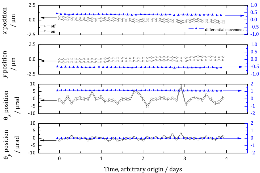
Figure 6. Linear and angular displacements of the coil between the two steps of the weighing mode during four typical days of h measurement. Four degrees of freedom of the coil are shown ( x , y , \theta_x , \theta_y ). The black open symbols describe the absolute position of the coil (mass on and mass off): the drift of the measured linear position is well below 1 \mu\text{m d}^{-1} , whereas drift of the measured angular position is not noticeable. The blue solid triangles represent the displacements of the coil from ‘mass off’ to ‘mass on’ (differential movement) during the same period. These displacements are 0.5 \mu\text{m} for x -axis, -0.5 \mu\text{m} for y -axis, 1.0 \mu\text{m} for the \theta_x -axis and 0.0 \mu\text{m} for the \theta_y -axis; these values exhibit negligible variation on this time scale.
