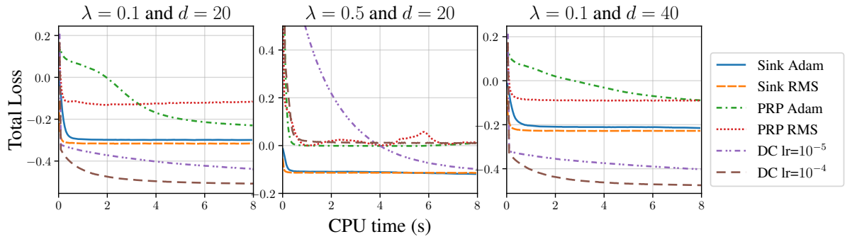
Figure 8.4: Comparison of optimization schemes. lr is the learning rate used for DC.
