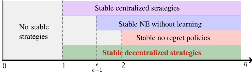
Figure 7.1: Existing results depending on the slack \eta . Our result is highlighted in red.
