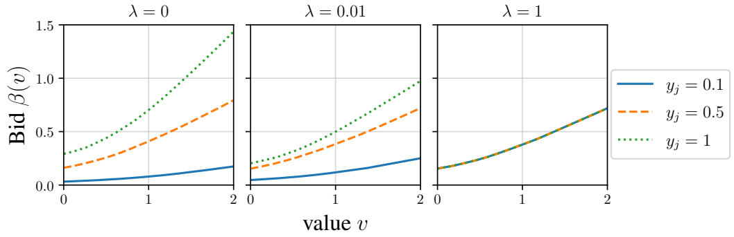
Figure 8.6: Evolution of the bidding strategy with the type and the regularization constant.
