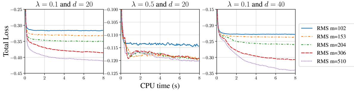
Figure 8.3: Influence of number of actions m .
