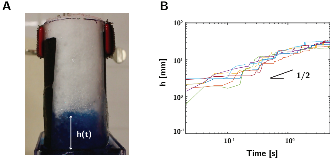
Figure 5.2: (A) Snapshot of the experimental set up: a solution of methylene blue is put in contact with a block of snow, leading to a capillary rise. (B) Liquid thickness evolution as a function of time at T=0^{\circ}\text{C} .
