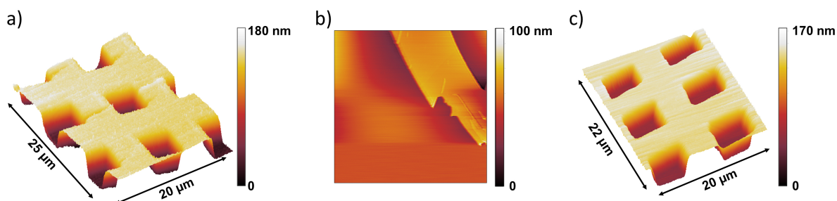
Figure 2.13: (A) AFM image of a standard nanoletric calibration grating (B) AFM image of a mica substrate. (C) AFM image of the same grating immersed in a very viscous silicone oil.
