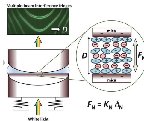
Figure 2.2: Schematic of a surface force apparatus taken from [66].
