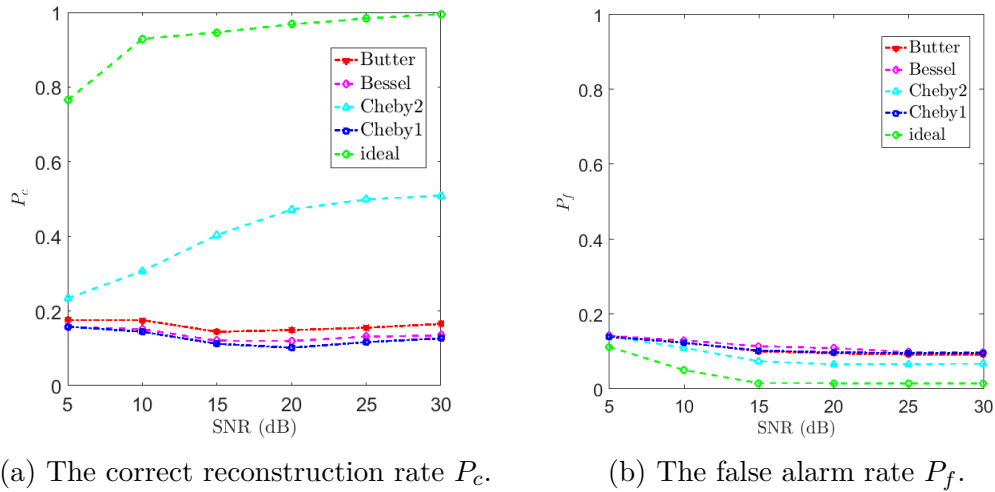
Figure 3.10 – The P_c and P_f for different SNRs without compensation when M = 4 , q = 5 , L = 96 , B = 7 MHz and F_{nyq} = 1 GHz.
