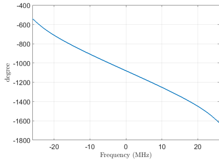
(a) Butterworth filter phase response.
