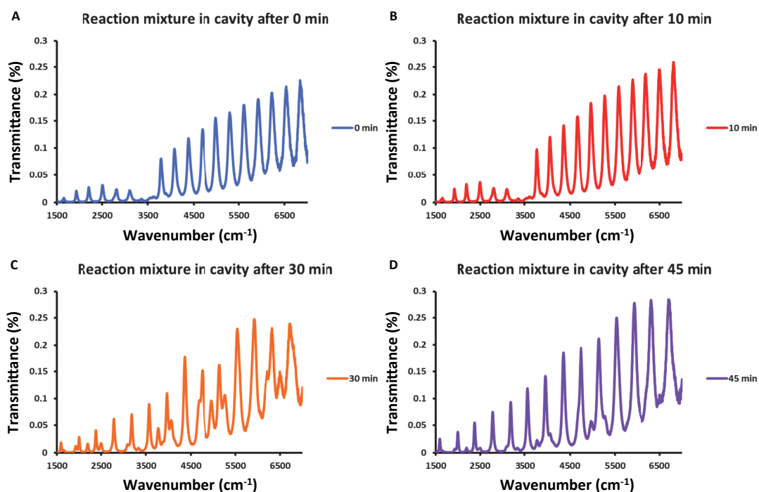
Figure 69. Evolution of the IR transmission spectrum of an on-resonance cavity in function of time. In this particular example, the cavity was tuned at 3386\text{ cm}^{-1} . The spectra shown here have been recorded immediately (A), 10 min (B), 30 min (C) and 45 min (D) after injection of the reaction mixture inside the cavity.
