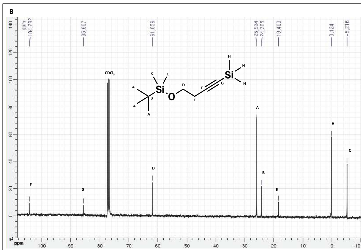
Figure 72. 1 H NMR spectrum of the reactant ( R ) with its various 1 H signals labeled from 1 to 5 on the schematic structure of ( R ) given in the inset. B. 13 C NMR spectrum with its various 13 C signals marked from A to H.
