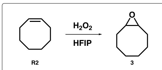
Figure 61. Epoxidation of cis -cyclooctene (R2) by \text{H}_2\text{O}_2 in HFIP
