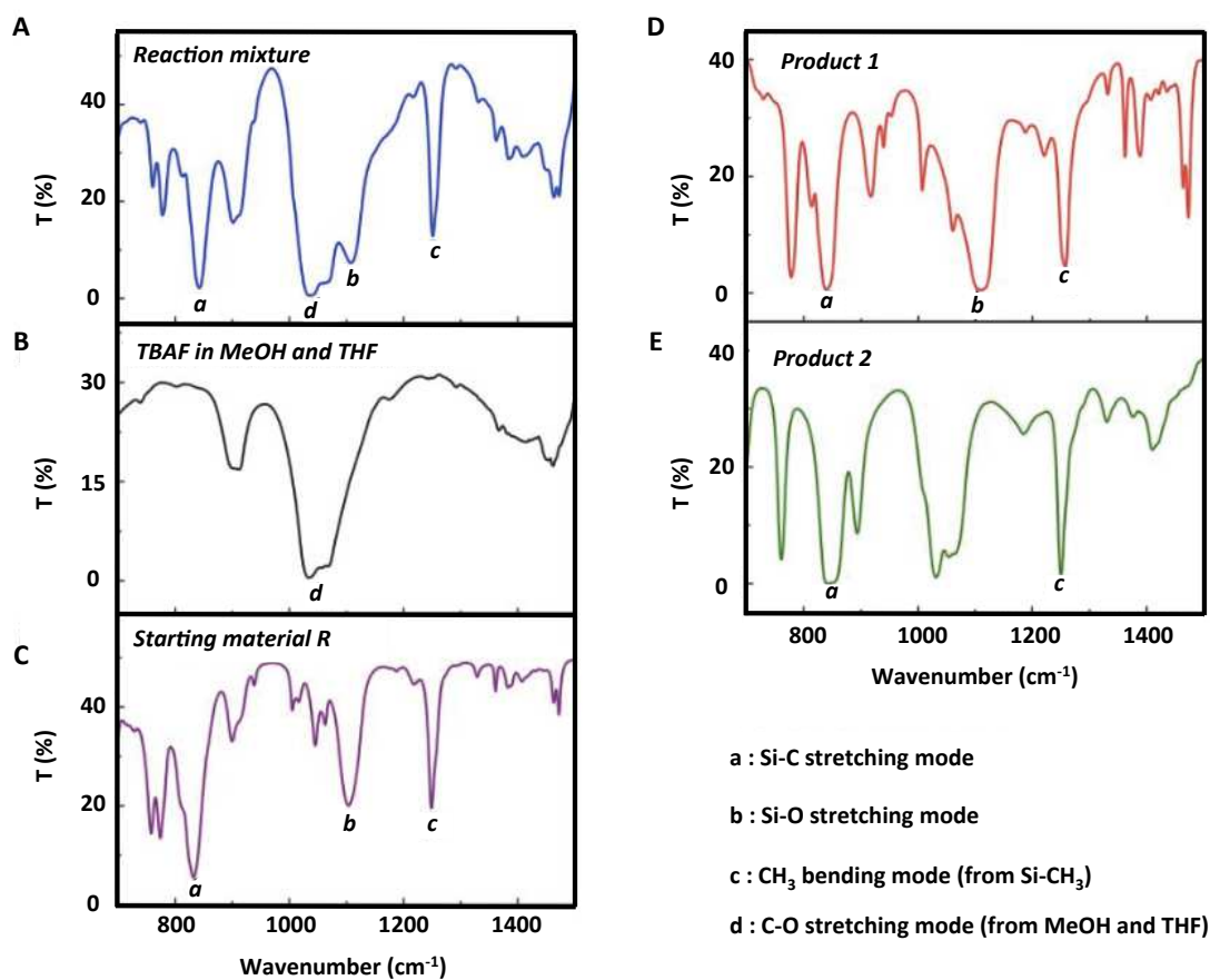
Figure 73. FT-IR transmission spectrum of: A. The reaction mixture containing the starting material (R) B. A solution of TBAF in methanol (MeOH) and THF C. Neat starting material (R) D. Neat product (1) E. Neat product (2) . The spectral window is limited to the region of interest of the present study. The vibrational modes of interest in the present study are marked from a-d. Neat products (1) and (2) were obtained from commercial sources.
