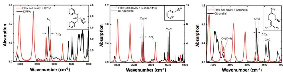
Figure 40. IR absorption spectra of three molecules (black curves, in absorption) that have been strongly coupled with the Fabry-Perot cavity modes (red curves). From left to right: diphenyl phosphoryl azide (DPPA), benzonitrile and citronellal.
