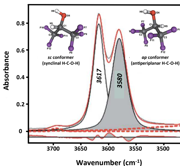
Figure 64. High frequency region of the IR spectrum of a 0.1M solution of HFIP in \text{CCl}_4 , showing the (\text{OH})_{\text{str.}} of HFIP. The band assigned to the ap conformer is shadowed in grey. The optimized structures of the ap and sc conformers of HFIP are illustrated in the inset. Adapted from reference 25.
