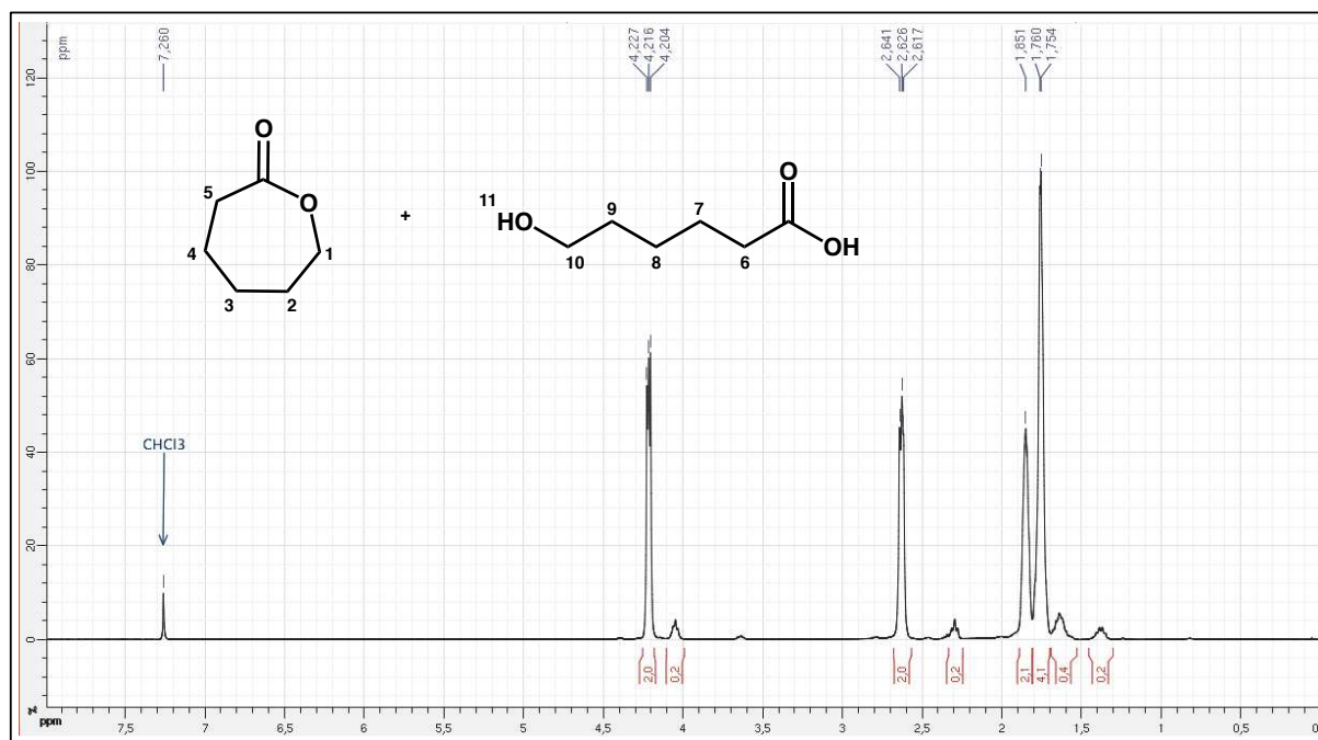
Figure 86. ^1\text{H NMR} spectrum of the product ( 4 ) with its various ^1\text{H} signals labeled from 1 to 5 on the schematic structure of ( 4 ) given in the inset (molecule on the left). The hydrolyzed form of product ( 4 ) is also visible on the spectrum, with its various ^1\text{H} signals labeled from 6 to 11 on the schematic structure given in the inset (molecule on the right).
