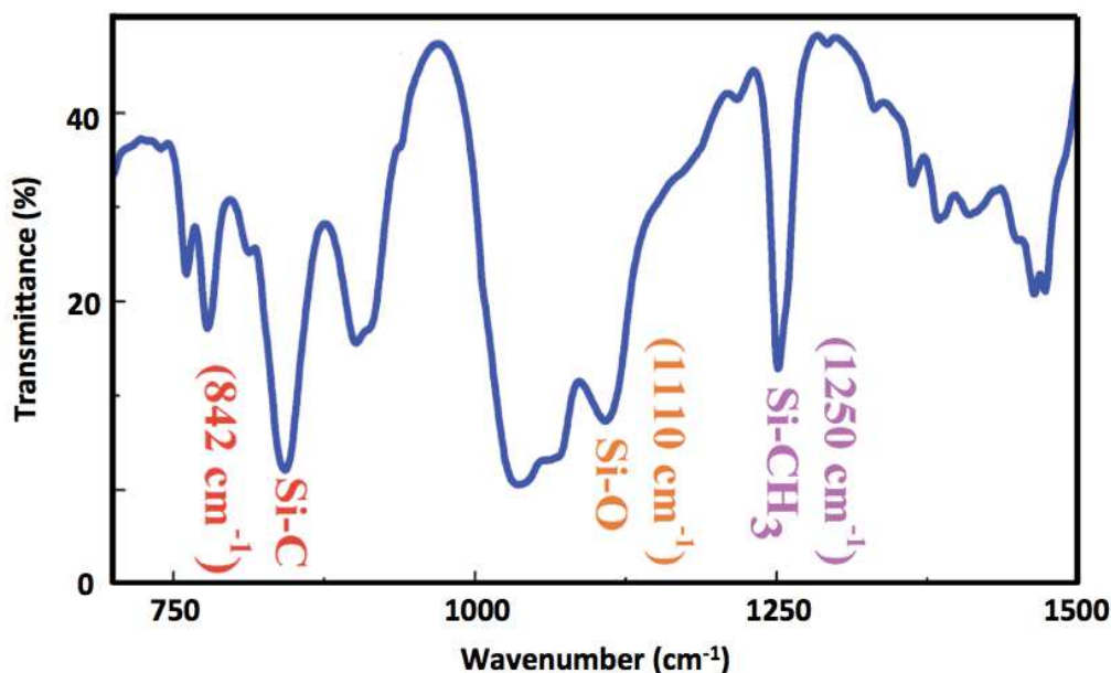
Figure 48. FT-IR transmission spectrum of the starting material ( R ) in the reaction mixture recorded in a flow-cell, with glass-coated ZnSe windows separated by the same spacer thickness as of the FP cavity.
