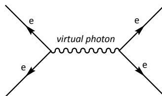
Figure 21. An example of one very simple Feynman diagram. Virtual photons (represented as wavy line) serve as force carriers for the interacting particles (here, electrons are represented as straight lines) that undergo changes in their velocity and direction of motion when they release or absorb the energy of a photon.
