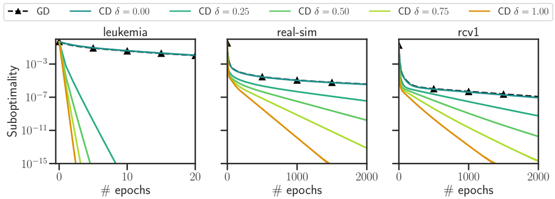
Figure 1.8 – Influence of stepsizes for cyclic coordinate descent, OLS. Suboptimality f(\beta^{(k)}) - f(\hat{\beta}) as a function of the number of epochs to solve a least squares problem on multiple datasets from libsvm : leukemia , real-sim and rcv1 . Gradient descent is compared against coordinate descent with step sizes \gamma_j = \delta/L_j + (1 - \delta)/L , for multiple values of \delta .
