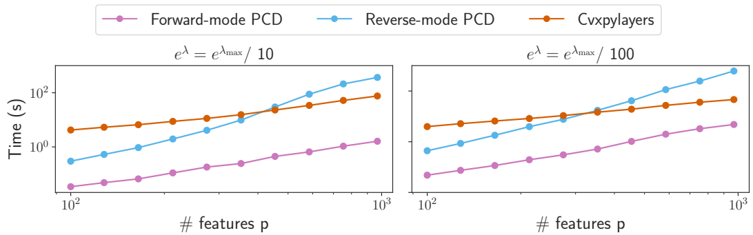
Figure 6.1 – Lasso with hold-out criterion : time comparison on the gina dataset to compute a single hypergradient as a function of the number of features, for two values of \lambda , e^\lambda = e^{\lambda_{\max}}/10 (left) and e^\lambda = e^{\lambda_{\max}}/100 (right).
