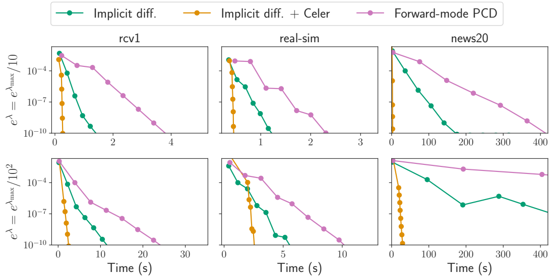
Figure 6.2 – Lasso with hold-out criterion : absolute difference between the exact hypergradient (using \hat{\beta} ) and the iterate hypergradient (using \beta^{(k)} ) of the Lasso as a function of time. Results are for three datasets and two different regularization parameters. “Implicit diff. + Celer” uses Celer (Massias et al., 2020b) instead of our proximal coordinate descent implementation.
