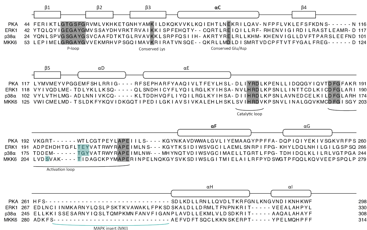
Figure 5: Structure-based sequence alignment of the kinases of interest in this work (ERK1, p38 \alpha and MKK6) relative to the reference kinase PKA. The alignment was published in Modi and Dunbrack, 2019a. Common kinase secondary structure with the kinase nomenclature are shown. Key conserved motifs and residues are highlighted in grey. Specific features of MAP2K and MAPK are indicated in teal.
