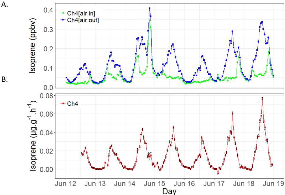
Figure II. (a) Temporal variation of the inlet and outlet isoprene mixing ratios (ppbv) from the wheat chamber and (b) the corresponding isoprene fluxes ( \mu\text{g.g}^{-1}.\text{h}^{-1} ) calculated.
