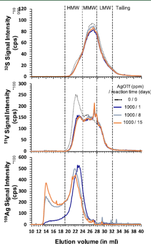
Figure 3. ^{109}\text{Ag} , ^{32}\text{S} , and ^{51}\text{V} GPC ICP-HR-MS chromatograms with 1000 ppm AgOTf mixed with AT-1 samples at different times.
