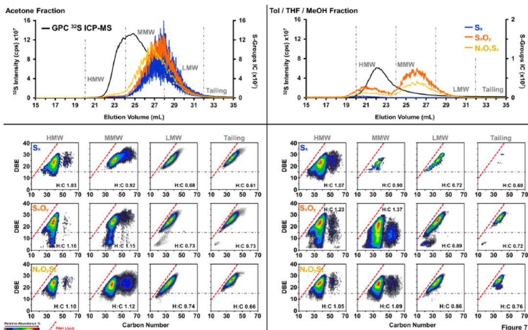
Figure 7. Upper row: GPC ^{32}\text{S} ICP-MS and ICs for S-containing groups for acetone (left) and Tol/THF/MeOH (right). Lower row: DBE vs carbon number plots for \text{S}_x , \text{S}_x\text{O}_y , and \text{N}_x\text{O}_y\text{S}_z groups. Abundance-weighted H/C ratios facilitate subfraction comparison.
