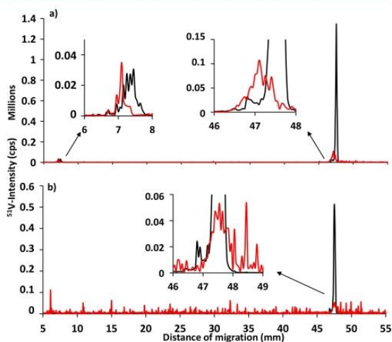
Figure 1. (a) 51 V signal and (b) 58 Ni signal from LA-ICP-MS of a one-step (40 mm) development with silica (red line) and cellulose (black line) HPTLC plates with DCM/MeOH 99.5/0.5 v/v of 1 µg of the reference porphyrin mixture.
