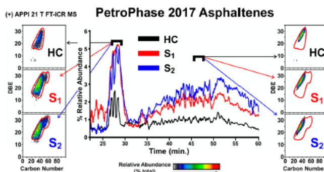
Figure 4. GPC FT-ICR MS extracted ion chromatograms for the hydrocarbon and sulfur heteroatom classes (center). Positive APPI-derived isobundance contour plots of DBE vs carbon number for the HC class (top), S 1 class (middle), and S 2 class (bottom) with short retention times (left) and long retention times (right). As aggregation decreases, the compositional range for each class moves from more aliphatic species on the left toward condensed polycyclic aromatics on the right.
