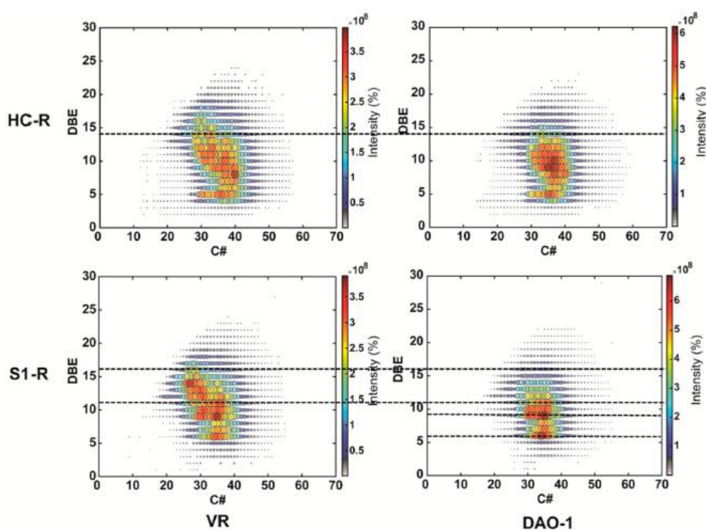
Figure 7. Double bond equivalent (DBE)/C# maps of the HC and S 1 chemical classes showing the cation radical species detected by the atmospheric pressure photo ionization (APPI) ± Fourier transformation ion cyclotron resonance (FT-ICR) mass spectra of VR (feed) and deasphalted oil (DAO) obtained from the SDA unit.
