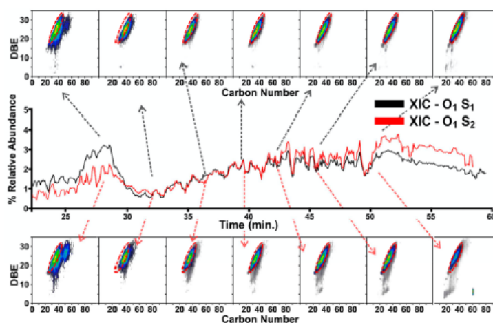
Figure 6. Extracted ion chromatograms and plots of DBE vs carbon number shown in order of elution from left to right for the O_1S_1 (top) and O_1S_2 (bottom) heteroatom classes from the PetroPhase 2017 asphaltenes.
