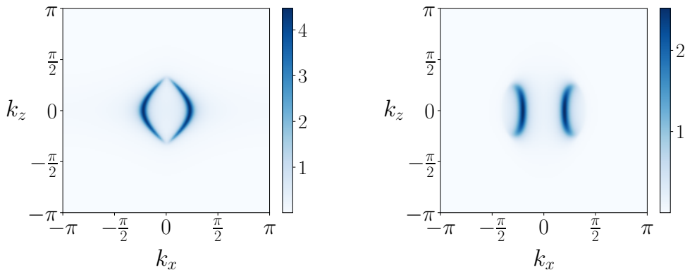
Figure 4.12 Surface spectral function at E = 0, y = -1 , for the Hamiltonian (4.8) with a surface impurity at y = 0 . The plots are obtained with the same set of parameters as in Fig. 4.11. We set U = 100 .
