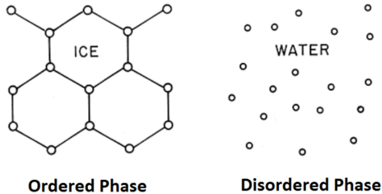
Figure 1.1 Illustration of two different phases: an ordered phase (crystal) where the position of the atoms is fixed, and a disordered phase (liquid) for which the atoms only have a certain probability of existing at a given point in space. Credit to Trung Van Phan .
