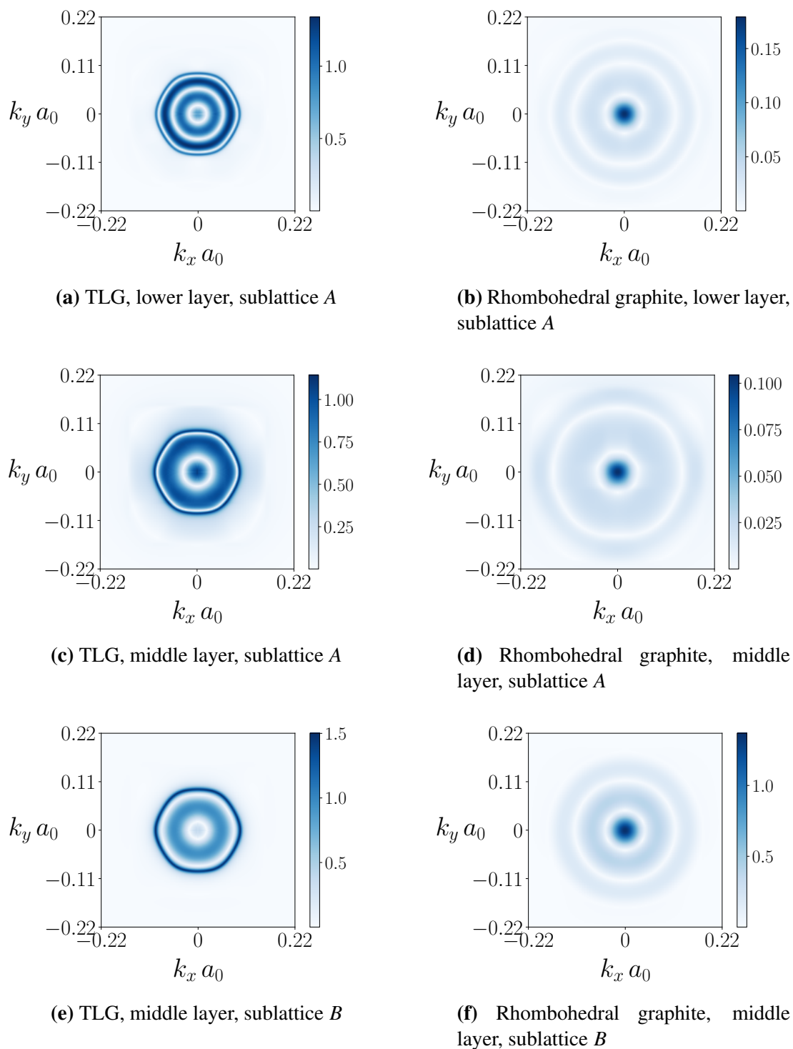
Figure 7.B.2 Quasiparticle interference pattern computed for TLG and rhombohedral graphite, for an impurity situated on different layers and sublattices.
