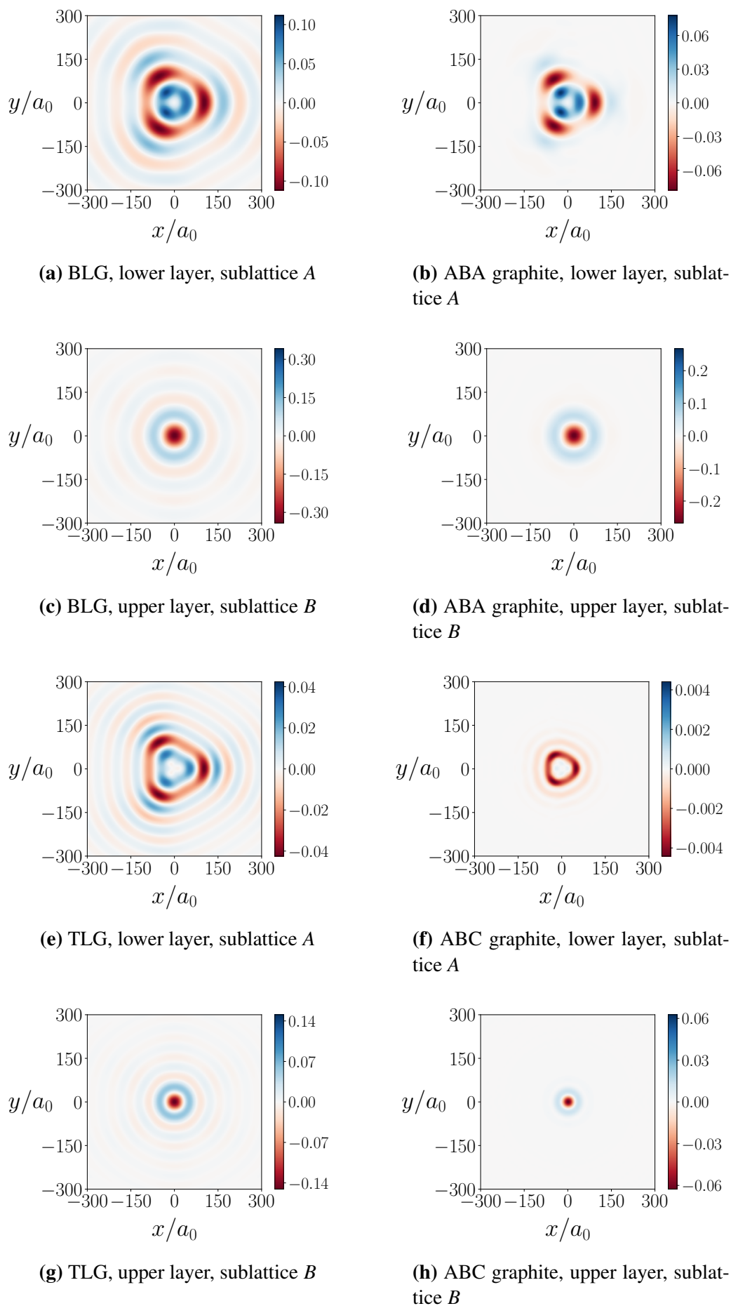
Figure 7.3.3 Real space QPI for the different systems around two distinct impurities: one on the sublattice A of the lower layer, the other on the sublattice B of the upper layer.
