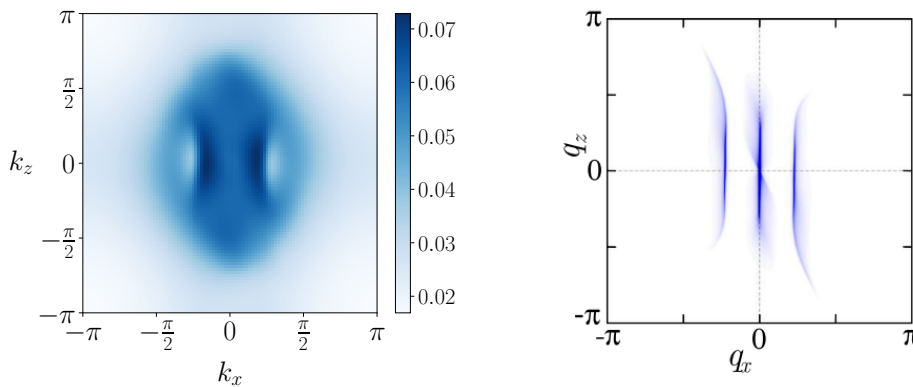
Figure 6.2.5 Left: Quasiparticle interference pattern corresponding to the surface spectral function of Fig. 6.2.4 , with V = \mathbb{I} . Right: JDOS obtained in Lau et al. 2017 for the same model and parameters.
