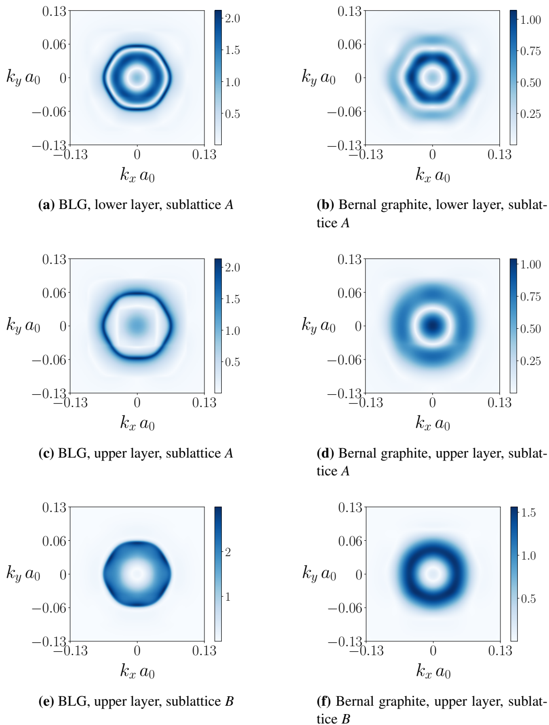
Figure 7.B.1 Quasiparticle interference pattern computed for BLG and Bernal graphite, for an impurity situated on different layers and sublattices.
