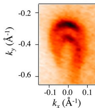
Figure 4.10 High-resolution ARPES Fermi surface map of crescent-shaped Fermi arcs on the surface of tantalum arsenide (TaAs), modified from Xu et al. 2015 )
