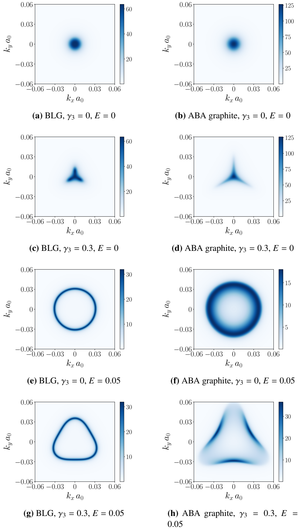
Figure 7.2.1 Surface spectral function of BLG and ABA graphite around the K point (corresponding to k_x = 0, k_y = 0 ), with and without trigonal warping.
