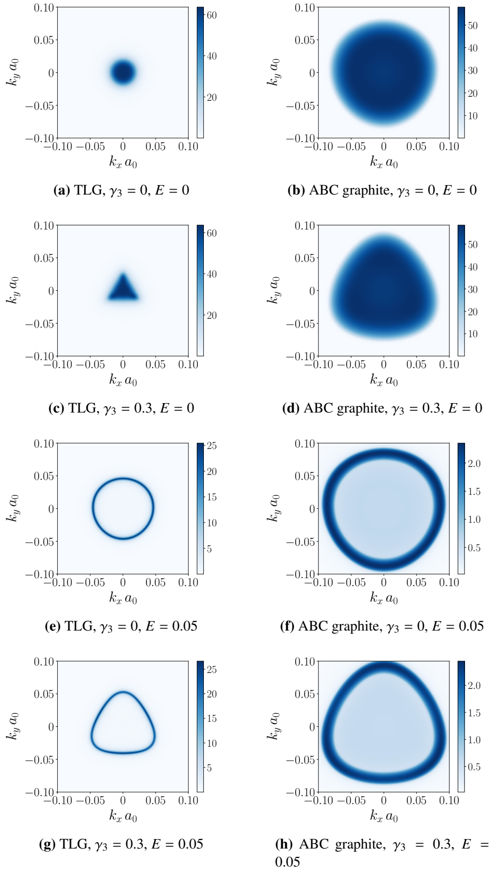
Figure 7.2.2 Surface spectral function of TLG and ABC graphite around the K point (corresponding to k_x = 0, k_y = 0 ), with and without trigonal warping.
