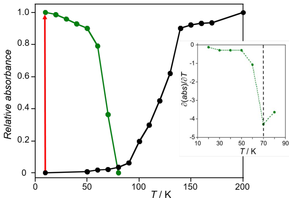
Figure 10. Temperature dependences of the the relative absorbance of the \nu_{\text{C}\equiv\text{N}(\text{HS})} (ABS vs. T ) vibration band observed at 2069 \text{cm}^{-1} from 200 to 10 K in the dark ( \bullet ); temperature dependences of the relative absorbance of the \nu_{\text{C}\equiv\text{N}(\text{LS})} (1-ABS vs. T ) band observed at 2105 \text{cm}^{-1} under 505 nm ( \text{---} ), with a power intensity of 40 mW, light irradiation at 10 K, for the crushed single crystals of 1 . Green dots are the subsequent thermal relaxation in the dark. Inset: Plot of \partial(\text{abs})/\partial T versus temperature indicating T(LIESST) value of 70 K.
