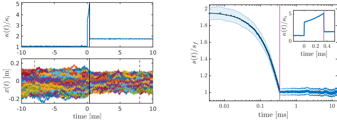
FIGURE 5.6: Experimental results of the optimal protocol. Left panel displays the ensemble of trajectories undergoing one cycle of the the optimal protocol \kappa_{\text{opt}}(t) shown on top. The black vertical lines indicate t_f . Right panel shows the temporal evolution of the corresponding ensemble variance s(t) with a 95% confidence interval.
