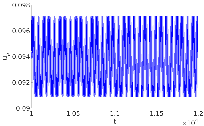
Figure VI.28 – Long time scale simulation for Re=1950 , and G=2 . The probe is located at (0.5,0,0.5G) . The displayed time span is equivalent to a bit more than 318 rotation of the disc.
