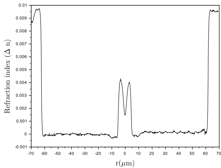
Figure 2.20: Example of refraction index profile measured on a P-doped silica fiber (4 at.% P).
