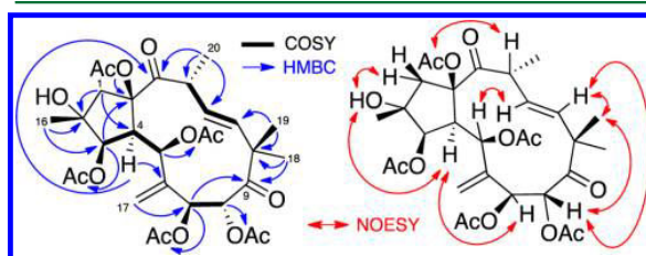
Figure 1. Key COSY (bold, left), HMBC (blue arrows, left), and NOESY (red arrows, right) correlations for the structure elucidation of 1 .
