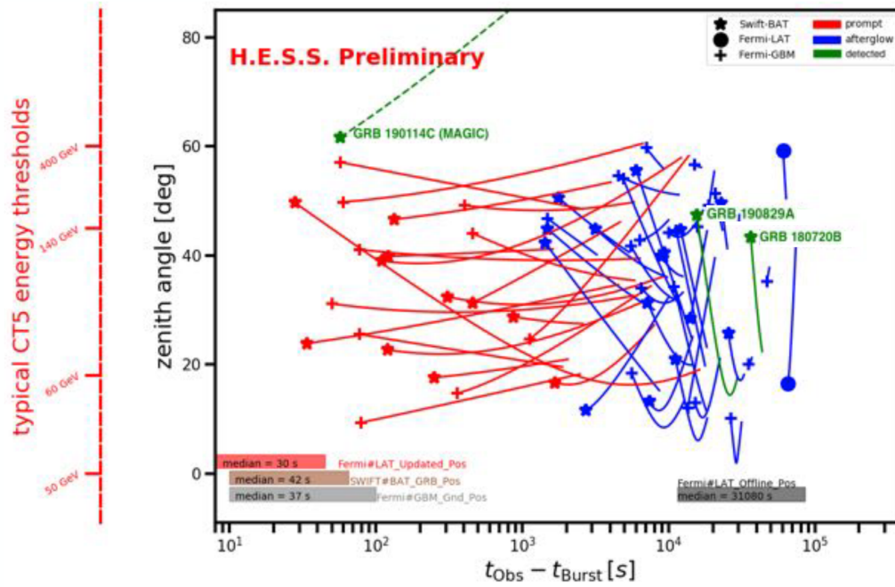
Figure 4.3: H.E.S.S. successful observation of GRBs detected by the Fermi-GBM, Fermi-LAT and Swift observatories. The plot shows the evolution of the zenith angle (y-axis) of the HR observations and therefore the variation of the energy threshold of the 28-m telescope with the observation time since the detection of the burst. Updated from [167].
