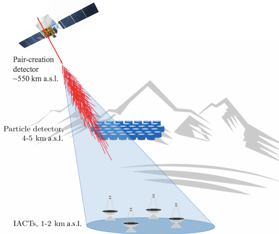
Figure 1.10: Illustration of an electromagnetic shower with space-based and ground based (water Cherenkov tanks and IACTs) VHE detectors at their preferred site altitudes. Adapted from [32].
