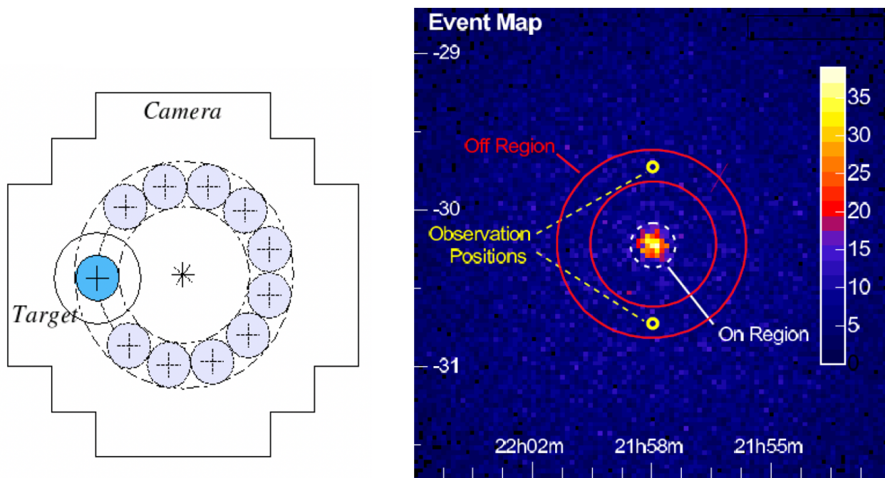
Figure 1.24: An example of the "Multiple off" (left) and "Ring background" (right) techniques for background subtraction on an event map. The color bar indicates the number of gamma ray like events. From [63].
