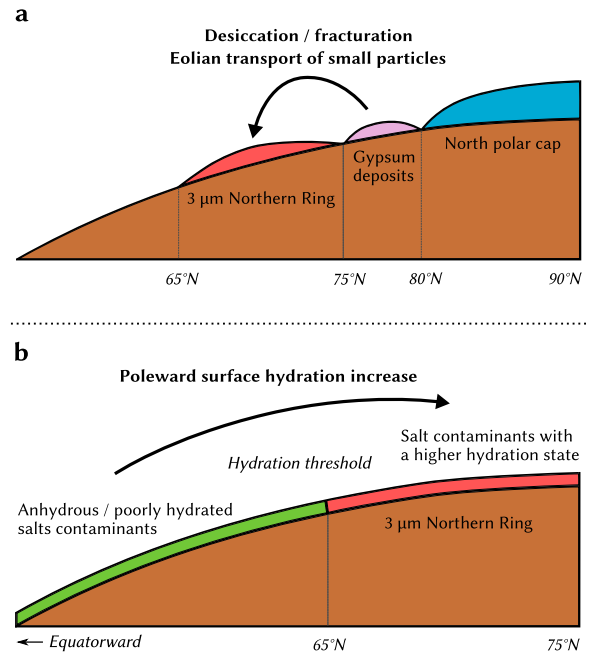
Fig. 16. Schematic drawings of two possible scenarios for the formation of the 3 μm northern ring. (a) Hydrated salts from the northern regions are transported to lower latitudes through eolian processes with a possible contribution of fracturation and desiccation either at source or arrival site. (b) A ~ 65° N latitude threshold separates two hydration states of salts (sulfates and/or perchlorates) contaminants within soils, with more hydration over the 3 μm northern ring.
