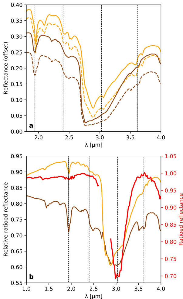
Fig. 15. (a) RELAB spectra of natural perchlorate salts from the Atacama desert in Chile. In orange, two different samples with particles sizes lower than 125 μm (dashed line JBE47, solid line JBE48). In brown, a third sample (JBE49) for two ranges of particle sizes: lower than 125 μm (solid line), and between 125 and 250 μm (dashed line). (b) Comparison between the typical spectral ratio associated with the 3 μm northern ring band (red, see Fig. 6 for details) and perchlorate salts ratios calculated using the laboratory spectra shown in panel (a). Orange: ratio of two natural samples with particles sizes lower than 125 μm (JBE47/JBE48); the presence of the 1.9 μm band in the ratio may indicate an hydration level difference between both. Brown: ratio of the 125–250 μm over the < 125 μm size for the JBE49 sample. Black dotted lines correspond to wavenumbers of 1.94, 2.9, 3.03, and 3.62 μm. RELAB spectra downloaded from the PDS spectral library (Milliken, 2020). (For interpretation of the references to color in this figure legend, the reader is referred to the web version of this article.)
