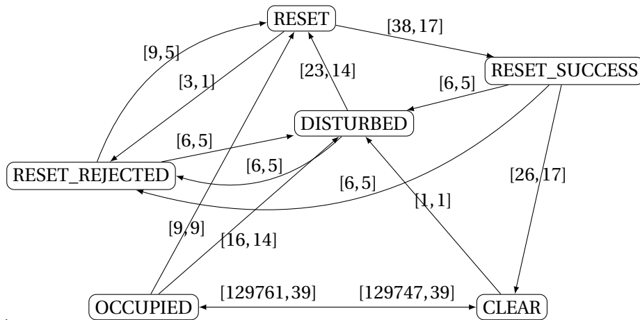
Figure 4.3: State transition graph automatically extracted from MoTRicS2015. Edge labels: [number of occurrences in all sections, number of sections it occurs in], all sections = 39.
