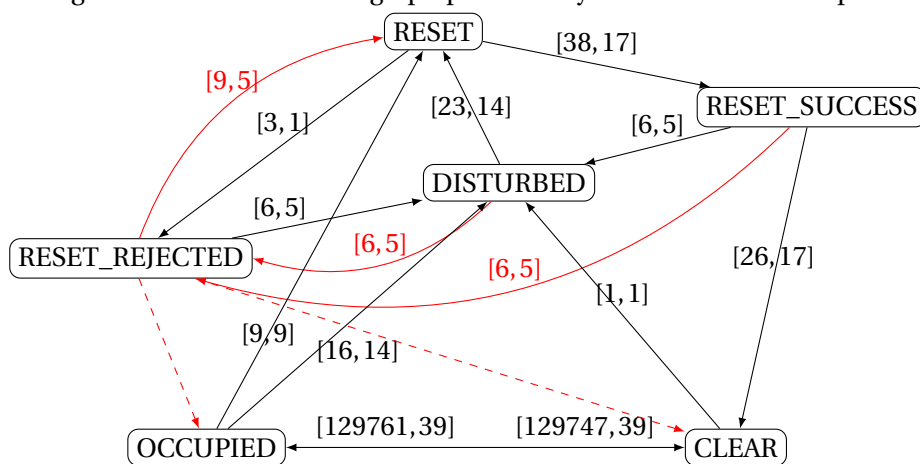
Figure 4.5: Comparison between graphs of Figures 4.3 and 4.4. Edge labels are taken from the data graph. Solid red edged are present in Figure 4.3 but not Figure 4.4, dashed red edges, on the contrary, are present on Figure 4.4 but not Figure 4.3.
