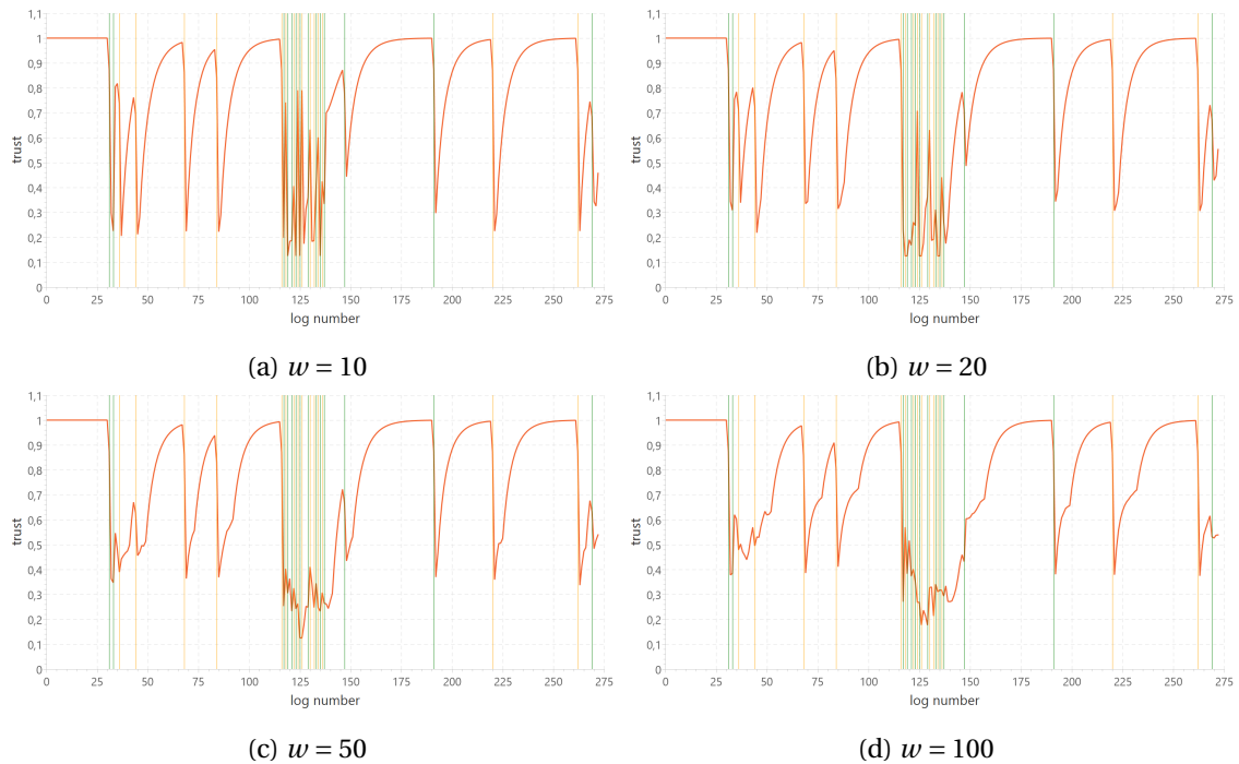
Figure 5.10: Trust evolution for different time windows
