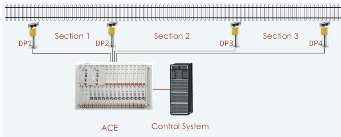
Figure 4.2: Illustration of the axle counter principle which consists in one ACE and multiple DPs. Provided by Thales: https://myproducts-thales.com/brochures-documents/1-brochure-fieldtrac-6315-az-lm/file
