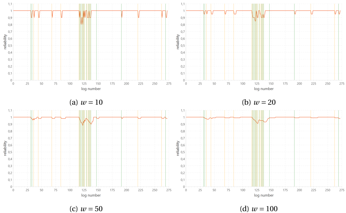
Figure 5.8: Reliability evolution for different time windows
