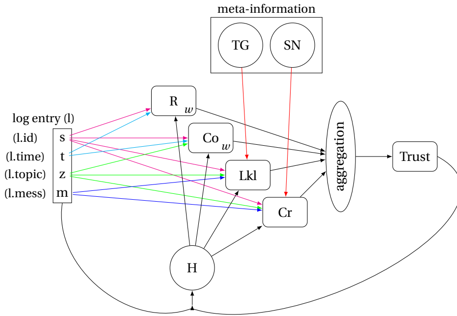
Figure 3.2: The general ReCLiC model.
