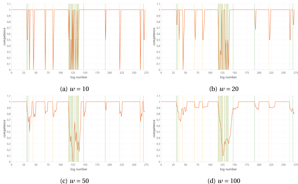
Figure 5.9: Competence evolution for different time windows
