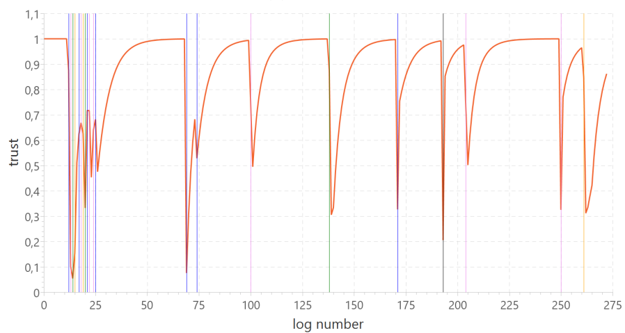
Figure 5.7: Trust evolution for different \alpha values
