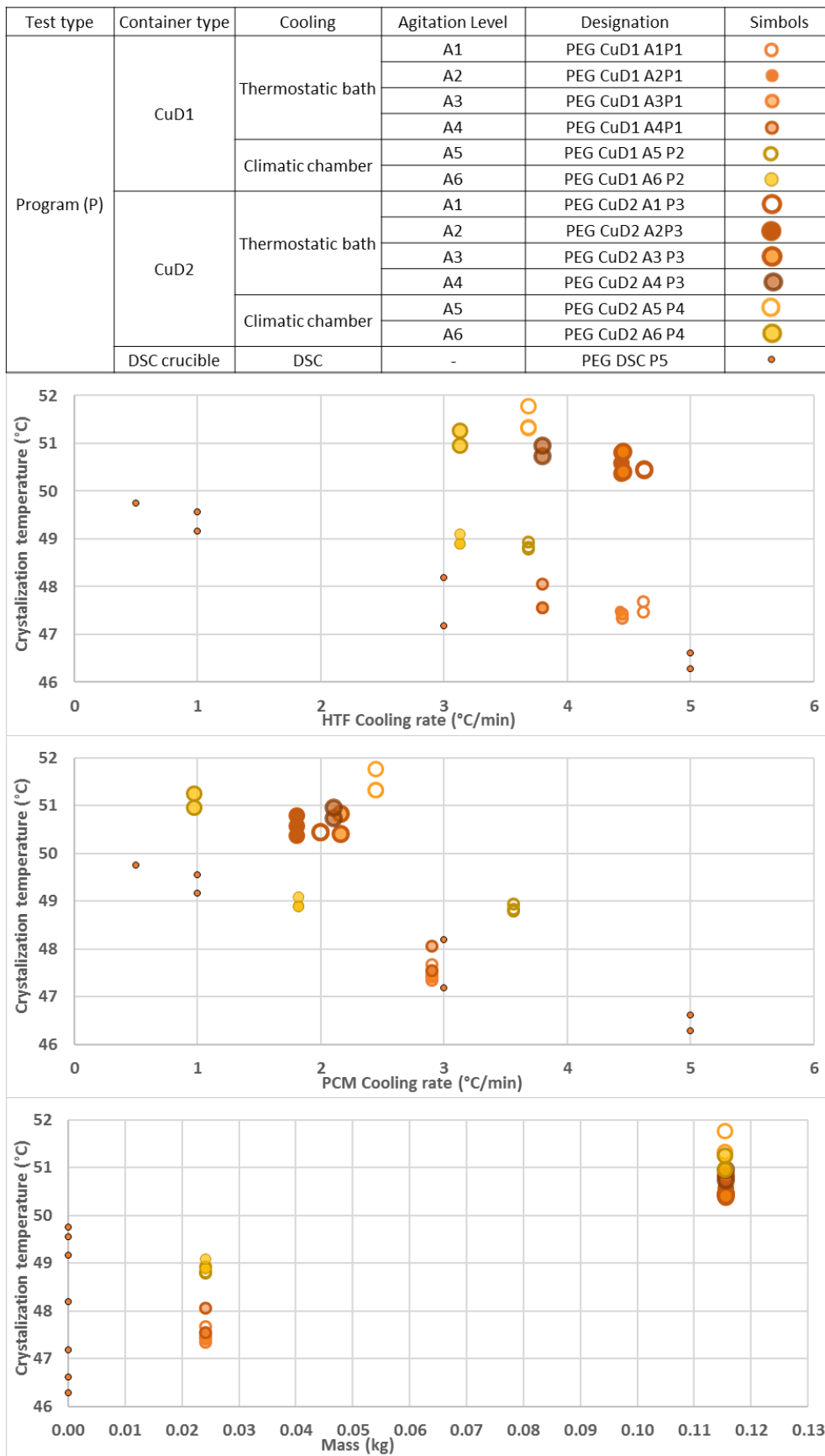
Figure 5. 6 Crystallization temperatures of PEG 10000 depending on the HTF and, PCM cooling rates and mass
