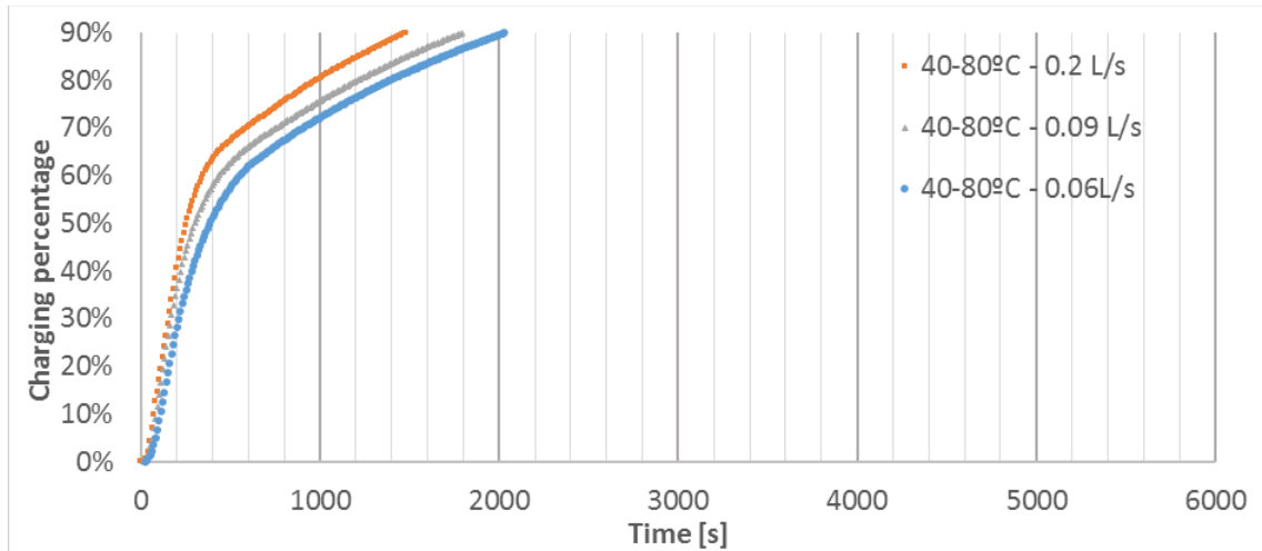
Figure 6. 11 Charging percentage of different flow rates with time
