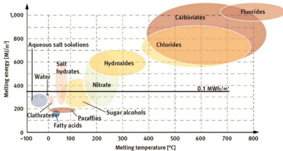
Figure 1. 5 PCM groups in function of their melting temperatures and melting energy [47]
