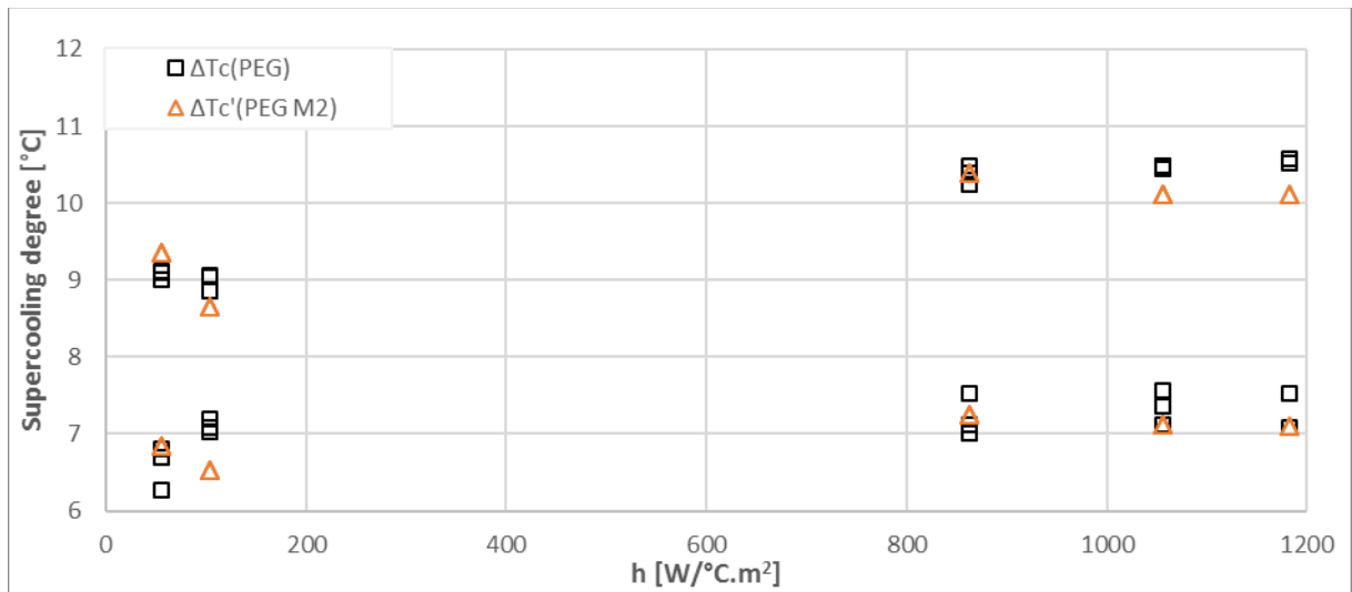
Figure 5. 19 Experimentally determined and modelled supercooling degree versus heat transfer coefficient values for PEG 10000
