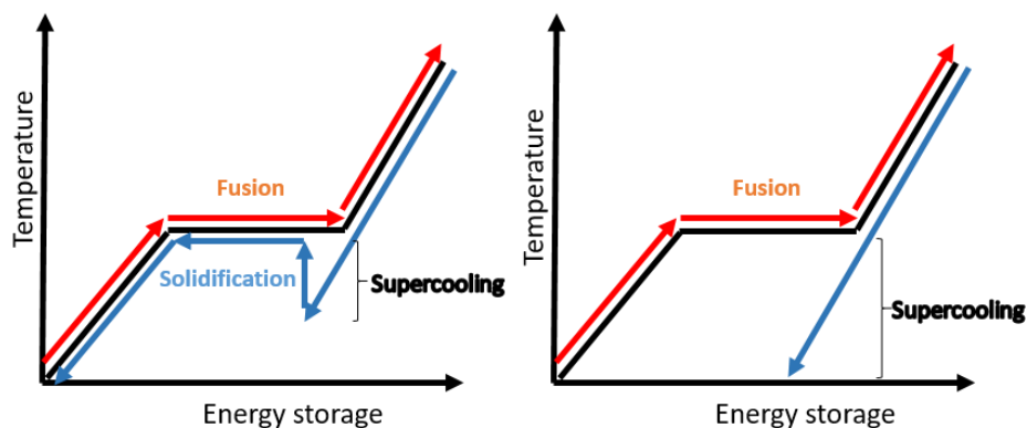
Figure 1. 6 Effect of the supercooling on thermal storage. Left represents slight supercooling and heat recovery after nucleation and right represents the case of severe supercooling when the material do not crystallize
