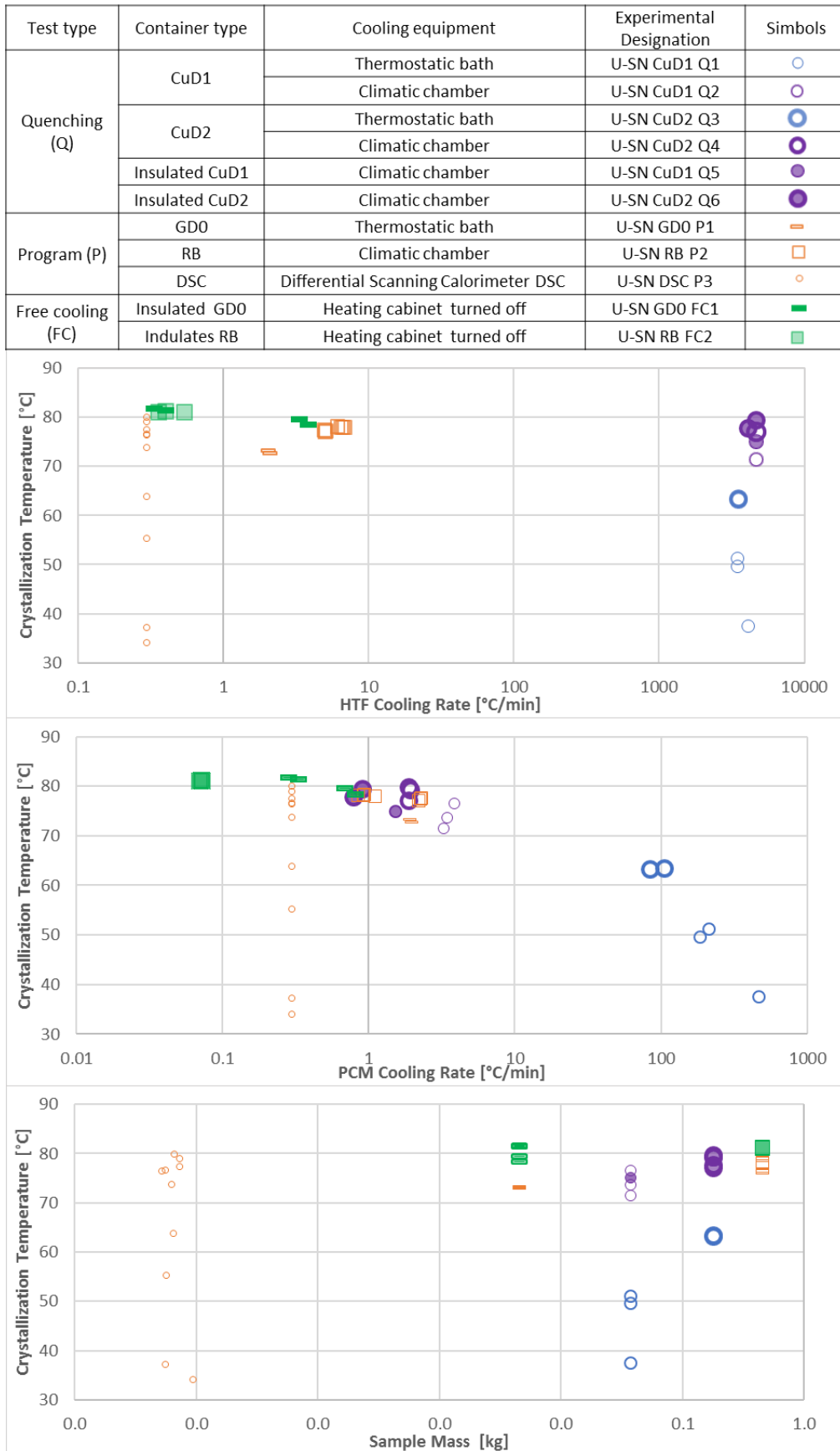
Figure 5. 5 Crystallization temperatures of U-SN eutectic depending on the HTF and PCM cooling rates, and mass
