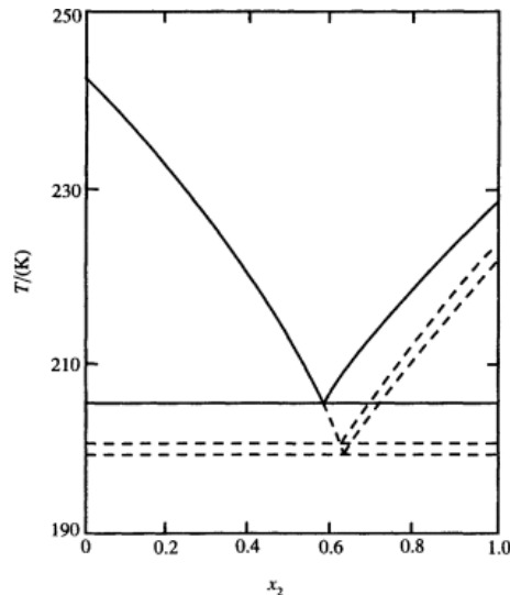
Figure 4. 3(Solid + liquid) phase equilibrium for \{x_1C_6H_5Br + x_21,3,5 C_6H_3(CH_3)_3\} . Continuous lines represent liquidus and solidus equilibrium temperatures, and the dashed lines represent metastable equilibrium between the liquid solution and unstable forms of 1,3,5-C6H3(CH3)3 [122]
