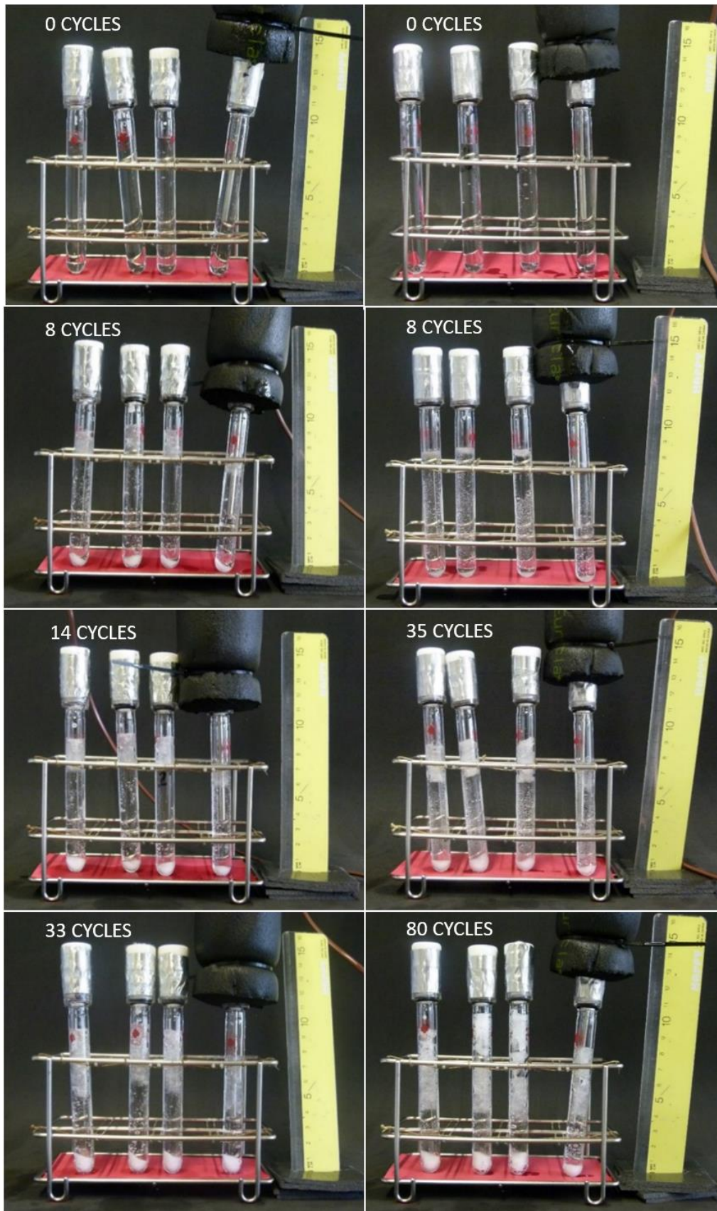
Figure 4. 8 Images of U-SN eutectic samples after selected number of thermal cycles at cooling rates of 0.3 °C/min (images on the left) and 2 °C/min (images on the right) where phase segregation is observed
