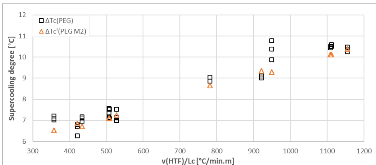
Figure 5. 18 Experimentally determined and modelled supercooling degree versus HTF cooling rate and characteristic length ratio values for PEG 10000
