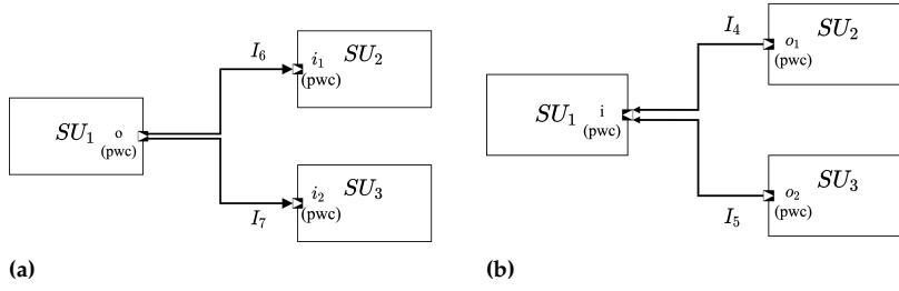
Figure 4.10: Two possible topological maps: 4.10a shows an allowed topological map; 4.10b shows a topology where multiple ports assign their value to a single port. The latter topological map is not allowed because a destination port must have only a source port.
