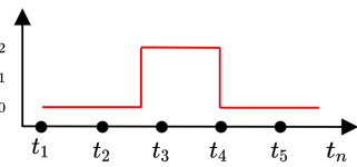
Figure 3.9: Piecewise-constant data.
