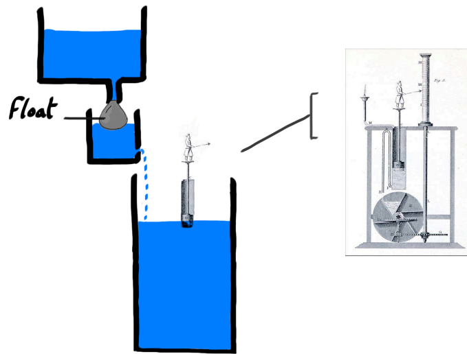
Figure 1.3: Ctesibius' solution for controlling the diminishing flow consisted in adding a third container between the two existing. Using a float regulator system, the water clock of Ctesibius required no outside intervention between the feedback and the controls of the mechanism.
