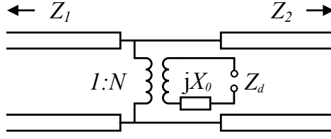
Figure 2.4 Equivalent network for the scan impedance of an infinite interfacial phased array of dipoles.
