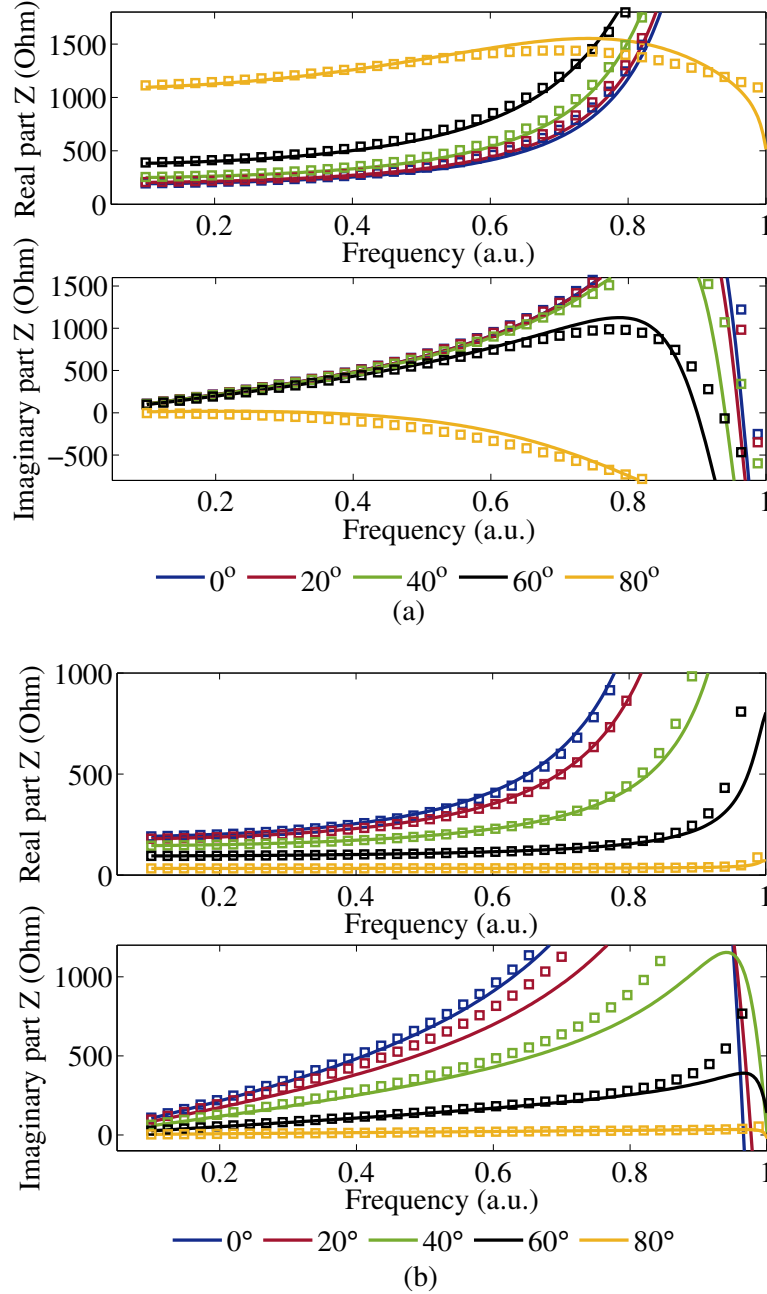
Figure 2.15 Real and imaginary parts of the scan impedance: simulated (solid lines), and calculated (squares) for a connected array of dipoles at different scan angles in (a) H-plane, and (b) E-plane.
