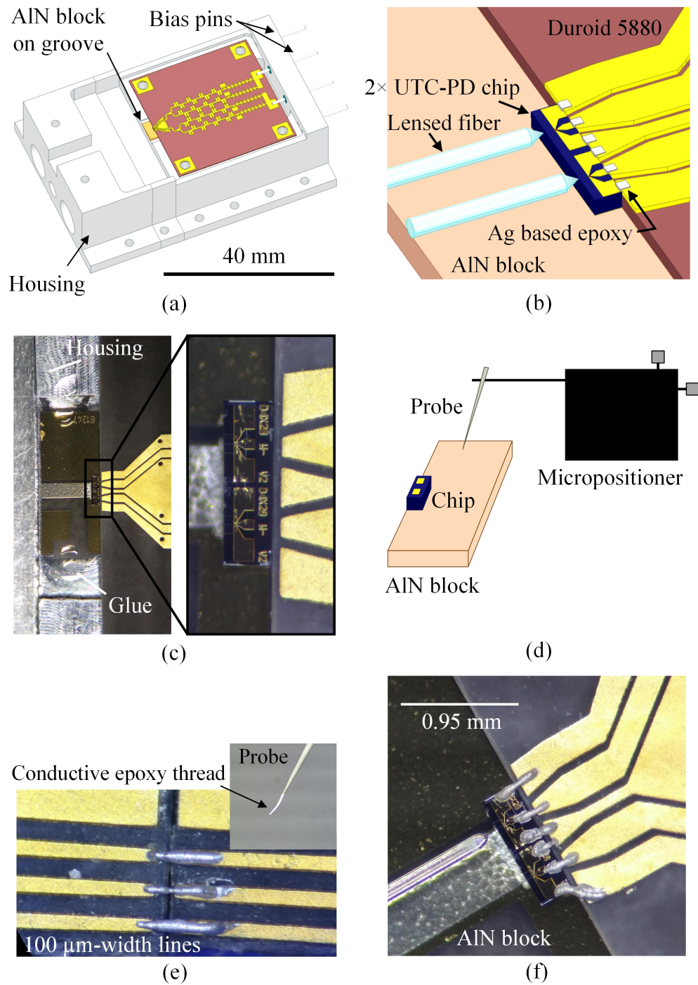
Figure 6.11 Images of the integration process: (a) designed housing, (b) G-CPW transition, (c) AlN block aligned to PCB and glued to the housing, (d) schematic of AlN block fixed in place by a micropositioner, (e) practice of thread bonding on 100 \mu\text{m} -wide dummy lines, inset: probe and epoxy thread ready to deposit. (f) detail of thread bonding and fiber used to excite the UTC-PD.
