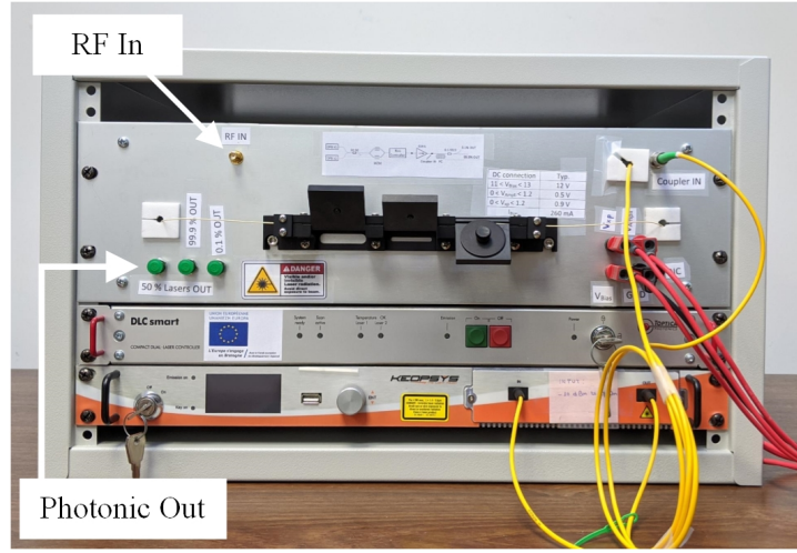
Figure E.2 Rack box used to arrange the components required for photonic generation and modulation of the optical tones (except for the mm-wave photonic Tx and OSA).
