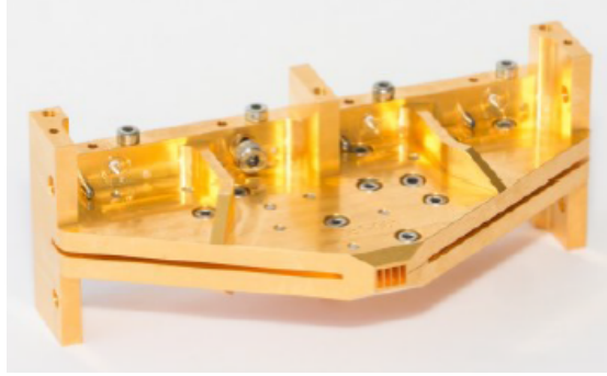
Figure 6.2 1 \times 4 horn array for a phased array at 300 GHz, from [211].
