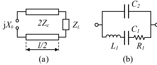
Figure 2.10 (a) Equivalent network representing the scan reactance. (b) Equivalent lossy lumped element circuit that represents the scan impedance.
