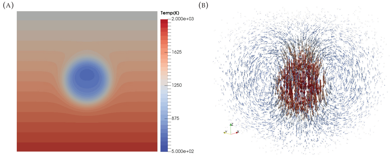
FIGURE 4.2: (a) Cross-sectional view in the yz — plane of the 3-D temperature field. The slice is taken at the center of the x — axis. (b) 3-D flow velocity due to the sinking anomaly. Largest flow magnitudes correspond to the cold anomaly.
