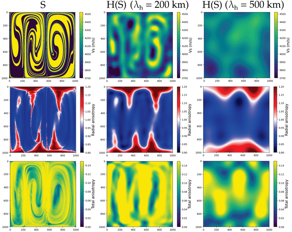
FIGURE 7.4: Some of the seismic properties of the reference medium \mathbf{S} before and after homogenization. The model dimensions are 1000 \text{ km} \times 1000 \text{ km} , with cell sizes of 5 \text{ km} \times 5 \text{ km} \times 5 \text{ km} . Here, each pixel contains an \mathbf{S} which consists of small-scale isotropic heterogeneities and an intrinsically anisotropic perturbation computed with D-Rex (Kaminski, Ribe, and Browaeys, 2004). The present-day marble cake patterns correspond to a mixing time for advection T_{\text{SPO}} \sim 75 \text{ My} , whereas the time scale for CPO evolution is T_{\text{CPO}} \sim 40 \text{ My} . We homogenized \mathbf{S} using the Fast-Fourier homogenization algorithm of Capdeville, Zhao, and Cupillard (2015). (From left to right) First row: V_s models derived from \mathbf{S} , \mathcal{H}(\mathbf{S}) at \lambda_h = 200 \text{ km} , and \mathcal{H}(\mathbf{S}) at \lambda_h = 500 \text{ km} . Second row: \xi_{\text{CPO}} , \xi^* at \lambda_h = 200 \text{ km} , and \xi^* at \lambda_h = 500 \text{ km} . Last row: Total anisotropy in terms of the norm fraction of \mathbf{S} , \mathcal{H}(\mathbf{S}) at \lambda_h = 200 \text{ km} , and \mathcal{H}(\mathbf{S}) at \lambda_h = 500 \text{ km} . Elastic homogenization can be viewed as the best possible model resolved by seismic tomography assuming perfect ray-path coverage.
