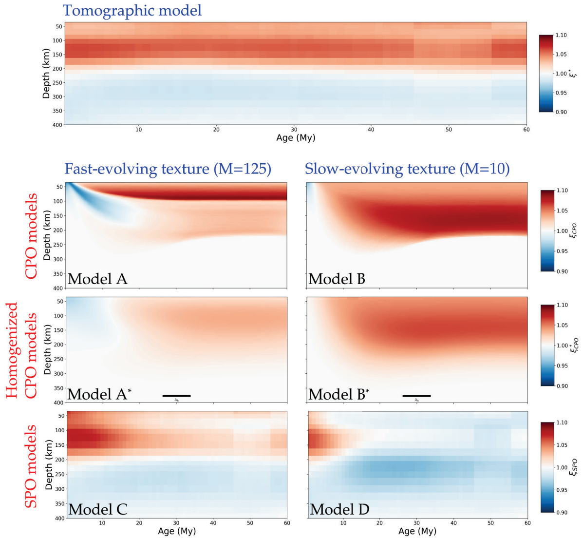
FIGURE 7.12: Radial anisotropy profiles across the upper-mantle underneath a mid-ocean ridge obtained from a tomographic model (top panel), reference CPO models corresponding to fast and slow-evolving textures (models A and B), homogenized versions of model A (model A*) and of model B (model B*). Upon homogenization, the strength of radial anisotropy is curtailed. CPO models constructed from reference parameter values therefore do not overestimate anisotropy, instead, seismic tomography underestimates anisotropy due to limited frequency band. Models C and D, respectively, are the extrinsic radial anisotropy profiles computed from \zeta^* of the tomographic model, and \zeta_{\text{CPO}}^* of model A* , and of model B* using the composite law. Positive lithospheric radial anisotropy in model C implies the existence of horizontally-laminated structures consistent with observations. This is absent in model D which is expected since model B* is designed to fit observations.
