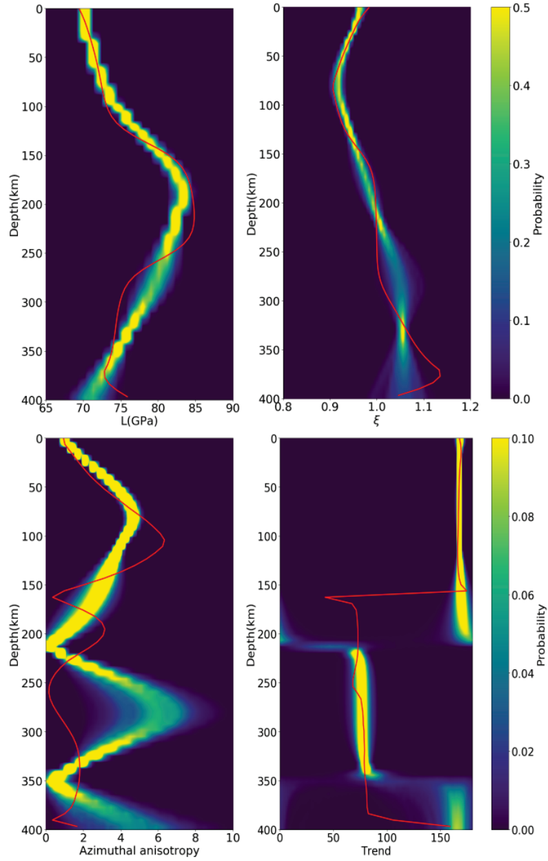
FIGURE 2.6: 1D marginal posterior distributions of L , \xi , peak-to-peak azimuthal anisotropy, and its fast azimuth \Psi at a specific geographical location, inferred from the Bayesian inversion of surface wave dispersion curves. The true structures are plotted in solid red.
