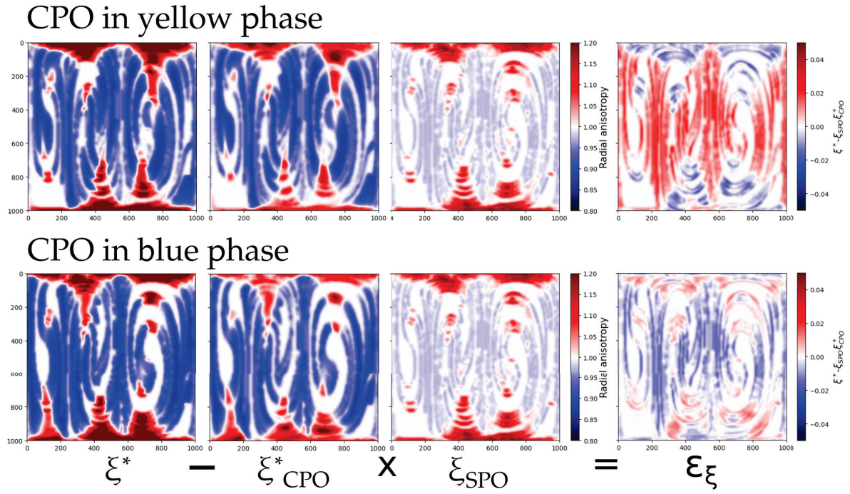
FIGURE 7.11: Quantification of the coupling between the shear modulus and intrinsic anisotropy in terms of the residual radial anisotropy \epsilon_{\xi} computed from \epsilon_{\xi} = \zeta^* - \zeta_{\text{CPO}}^* \zeta_{\text{SPO}} at each pixel in the 2-D maps of radial anisotropy under two scenarios: CPO is only computed in (1) the yellow phases (top panels), and (2) the blue phases (bottom panels). The reference 2-D maps \mathbf{S} , \mathcal{A}(\mathbf{S}) , and \mathcal{I}(\mathbf{S}) are homogenized at \lambda_h = 50 km to obtain \zeta^* , \zeta_{\text{CPO}}^* , and \zeta_{\text{SPO}} , respectively. Based on the \epsilon_{\xi} maps, shear modulus and intrinsic anisotropy are anti-correlated in (1), and positively correlated in (2). In both cases, the magnitudes of the cross terms are essentially equivalent, and only differ by their signs.
