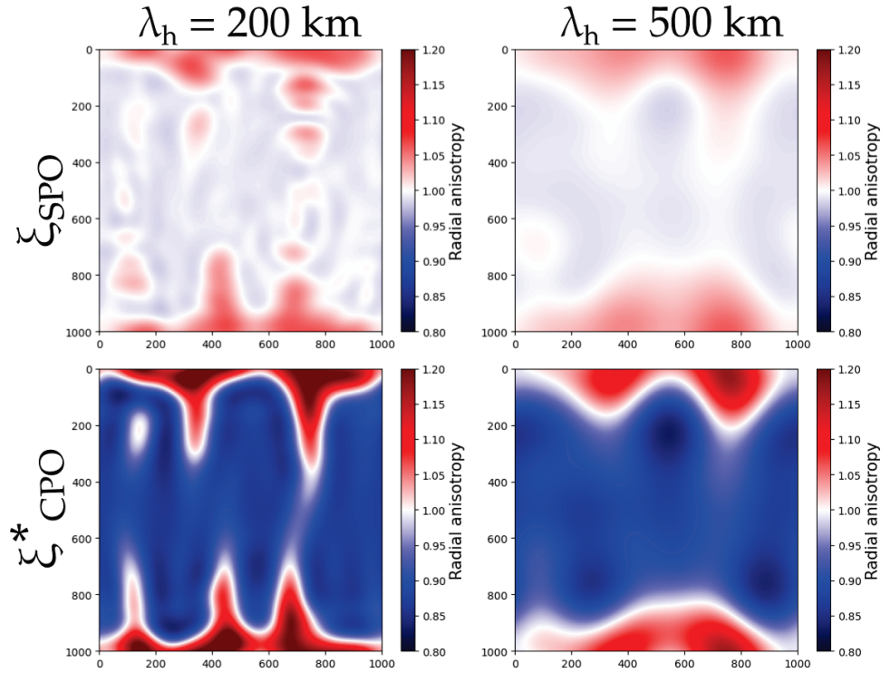
FIGURE 7.5: Extrinsic radial anisotropy \zeta_{SPO} ( i.e. , radial anisotropy of model \mathcal{H}(\mathcal{I}(\mathbf{S})) ) (top panels) at two different wavelengths of homogenization \lambda_h . Here, \zeta_{SPO} > 1 is now interpreted as vertical layering whereas < 1 as horizontal layering. The bottom panels are the effective intrinsic radial anisotropy \zeta_{CPO}^* ( i.e. , radial anisotropy of model \mathcal{H}(\mathcal{A}(\mathbf{S})) ).
