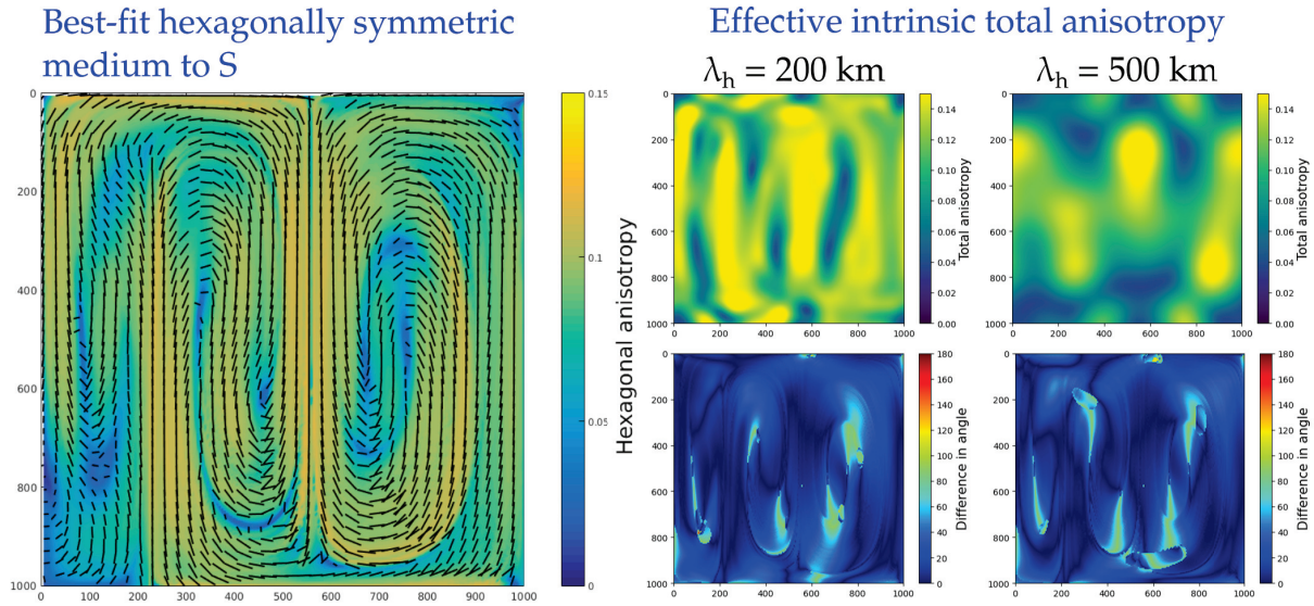
FIGURE 7.8: (Left panel) Amplitude and symmetry axis orientation (solid black lines) of the best-fit hexagonally symmetric medium to \mathbf{S} . We use the elastic decomposition method of Browaeys and Chevrot (2004) to arrive at such a medium. The symmetry axis maps well regions of high hexagonal anisotropy associated with strong shear deformation. It is often used as a proxy to identify the fast axis of olivine which appears to be also in agreement with the shear direction. (Top right panels) Effective intrinsic total anisotropy ( i.e. , total amount of anisotropy in \mathcal{H}(\mathcal{A}(\mathbf{S})) ) at two different wavelengths of homogenization. (Bottom right panels) Difference in the angle of the symmetry axis of a hexagonally-projected \mathbf{S} and \mathcal{H}(\mathcal{A}(\mathbf{S})) . Regions of high-misfit in the angle correlates well with low amplitudes of anisotropy.
