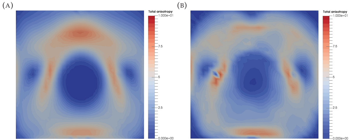
FIGURE 4.10: Cross-sectional view in the yz – plane of the percentage of total anisotropy( i.e. , norm of S_{ij} ) inferred from (a) true model, (b) mean model. The absence of anisotropy at the center corresponds to a region of minimal deformation for the cold and highly-viscous anomaly. The cross sections are taken at the center of the x – axis.
