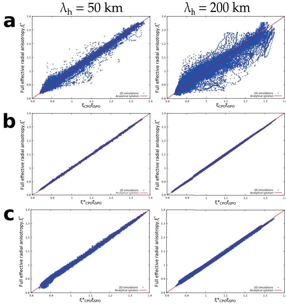
FIGURE 7.10: For each pixel i on our 2-D maps of \xi^* , \xi_{\text{CPO}} , \xi_{\text{CPO}}^* , and \xi_{\text{SPO}} Figure 7.10a: , we plot a cloud of points with coordinates: (a) [\xi_{\text{CPO}} \times \xi_{\text{SPO}}(i), \xi^*(i)] , (b) [\xi_{\text{CPO}}^* \times \xi_{\text{SPO}}(i), \xi^*(i)] overlaying the analytical solution equation (7.33) (solid red lines). Our numerical simulations suggest that CPO models should be homogenized first before comparing with tomographic models. Figure 7.10c displays the effect of the cross term by increasing isotropic heterogeneities to 15% and by prescribing CPO only in the yellow phases of the marble cake model in Figure 7.3.
