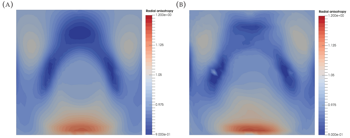
FIGURE 4.9: Cross-sectional view in the yz – plane of the radial anisotropy \zeta inferred from (a) true model, (b) mean model. Radial anisotropy is often used as a proxy to infer flow orientation. A \zeta > 1 (positive radial anisotropy) is often interpreted as horizontal flow. A \zeta < 1 (negative radial anisotropy) on the other hand, pertains to vertical flow. A \zeta = 1 indicates the absence of radial anisotropy. The cross sections are taken at the center of the x – axis.
