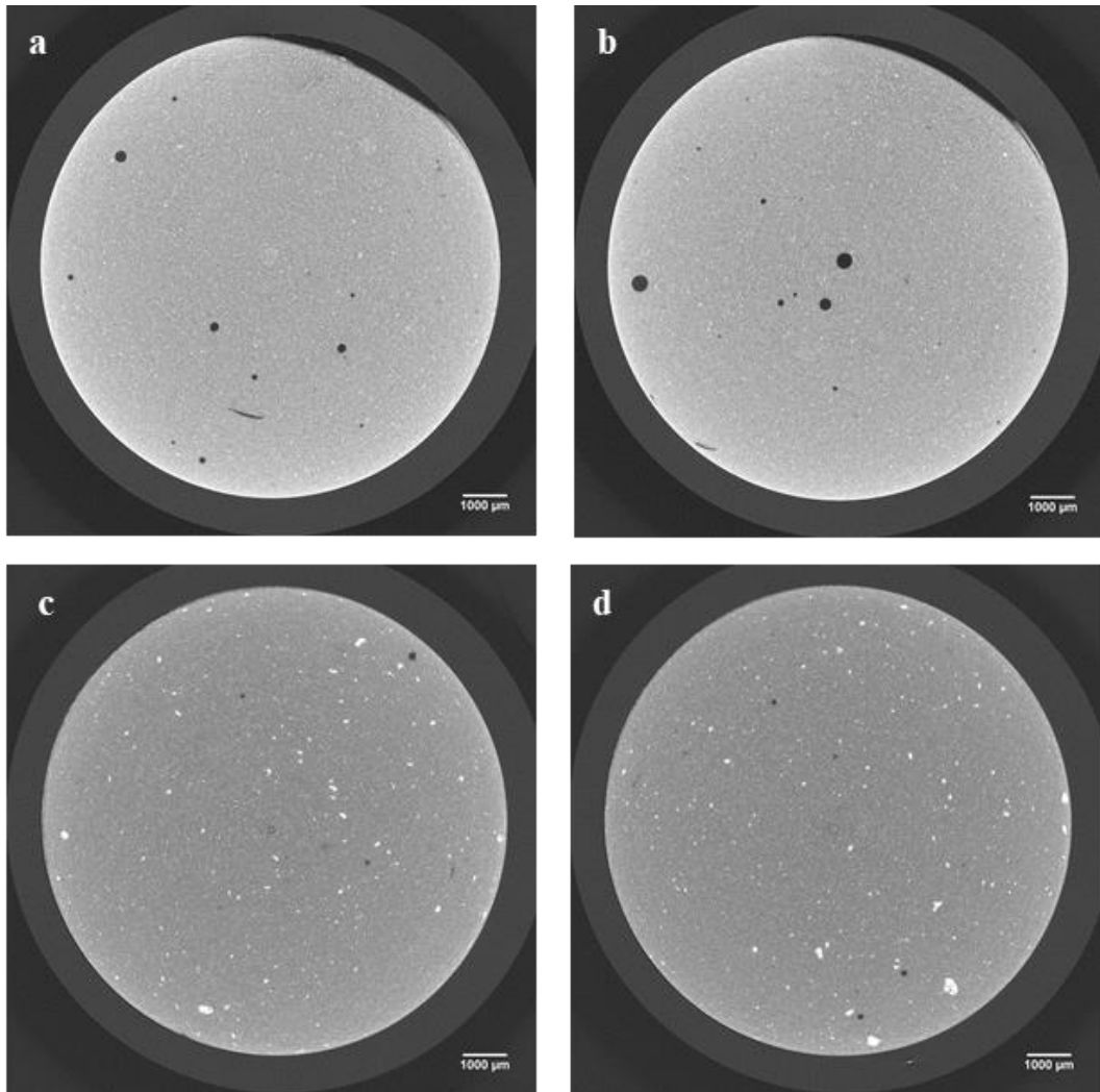
Figure 5.87: Tomography scans : Comparison between 0% (a,b) and 5% (c,d) GGBS replacement by 5% coarse clinker at the age of 120 days, with 8%Na 2 CO 3 and 0.1% 4Na*HEDP at W/B=0.40
