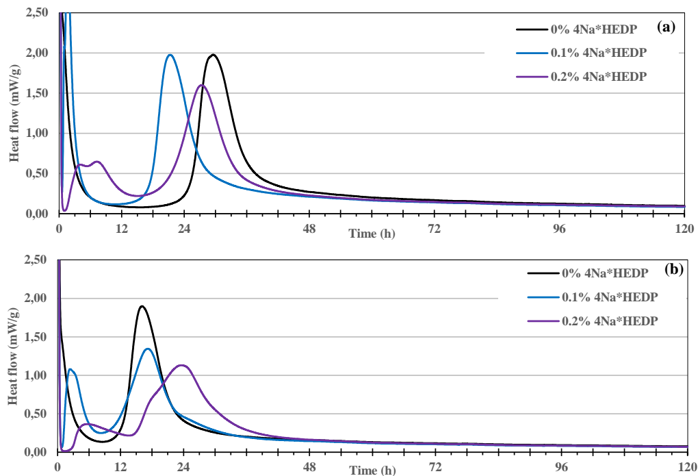
Figure 5.44: Influence of 4Na*HEDP on the hydration kinetics for GGBS 5600 cm 2 /g Blaine with 5% replacement by Clinker 1400 cm 2 /g at W/B=0.40 with 8% (a) or 6% (b) \text{Na}_2\text{CO}_3
