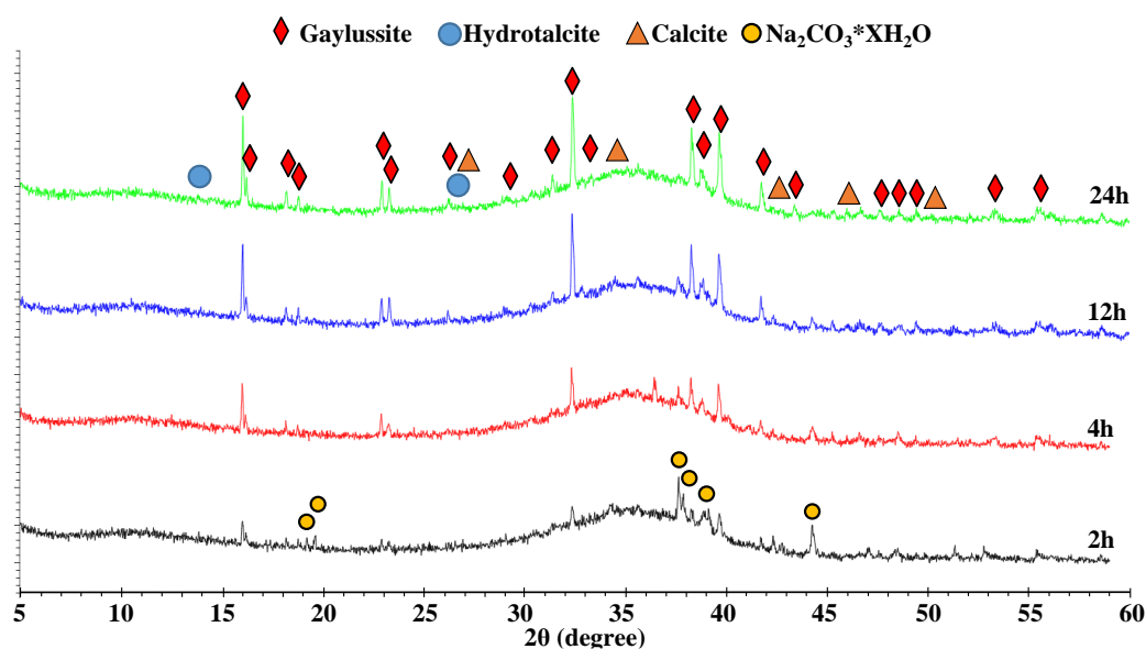
Figure 2.71: XRD patterns evolution of GGBS with 8% \text{Na}_2\text{CO}_3 at \text{W/B}=0.40 during the first 24h
