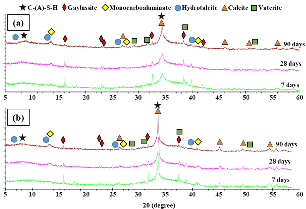
Figure 6.25: XRD patterns of GGBS hydration without (a) and with (b) 5% replacement by ultrafine limestone. Water/GGBS= 0.40 and 8% \text{Na}_2\text{CO}_3
