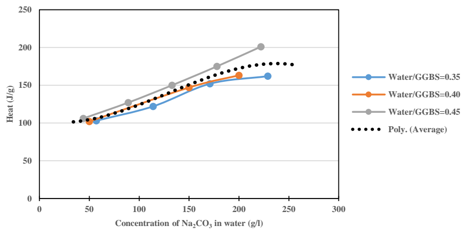
Figure 2.46: Heat released after 120h of hydration process of GGBS 5600 cm²/g as a function of initial sodium concentration in water.
