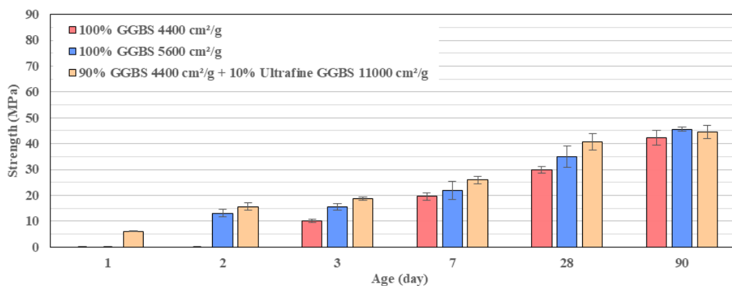
Figure 4.14: Comparison of strength evolution for different GGBS fineness. 4% \text{Na}_2\text{CO}_3 (100 g/l) and 0.05% 4Na*HEDP were used at W/B=0.40
