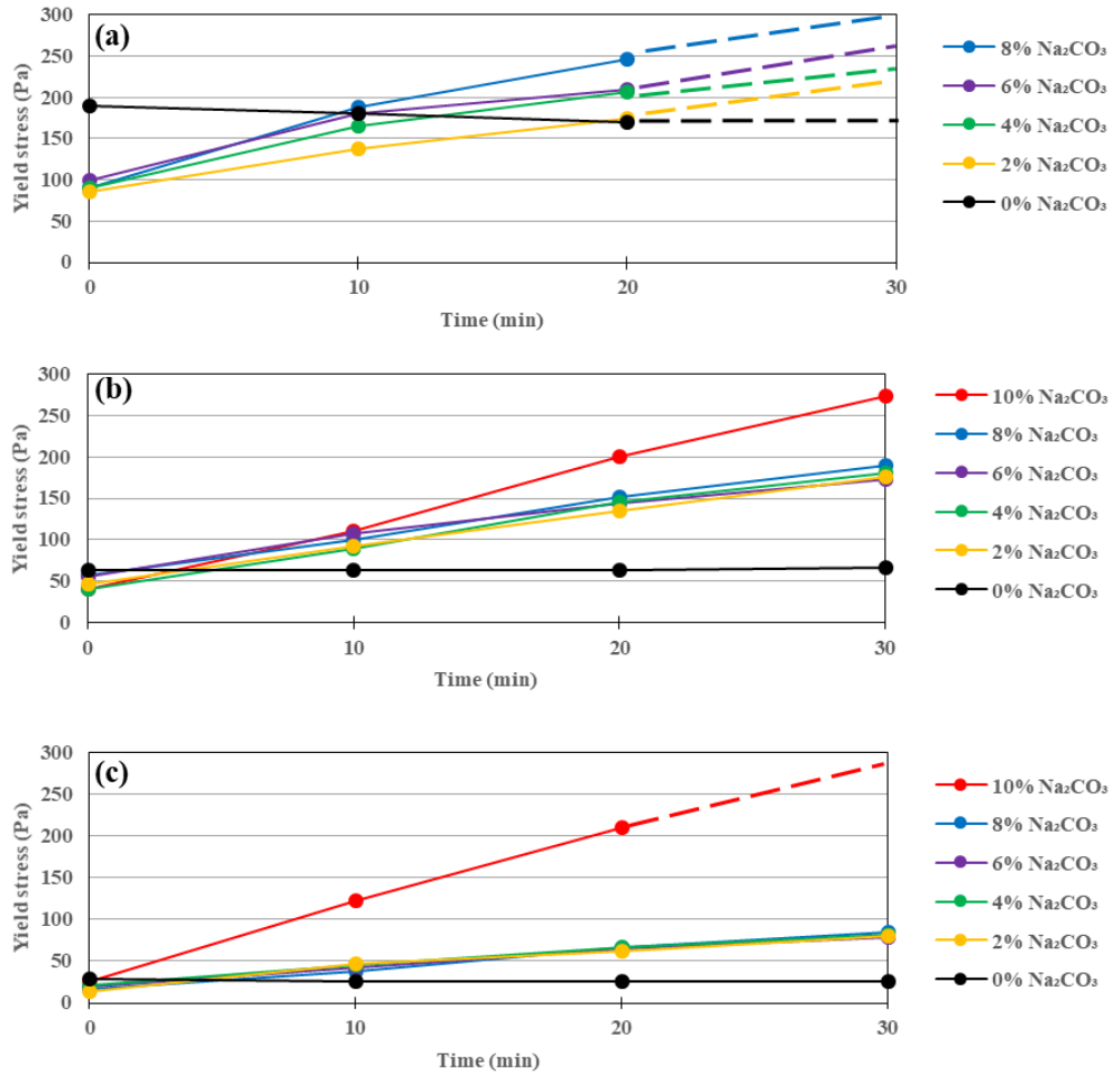
Figure 2.27: Yield stress evolution in time for Standard GGBS with different dosage of \text{Na}_2\text{CO}_3 and at different W/B ratio: 0.35 (a); 0.40 (b) and 0.45 (c)
