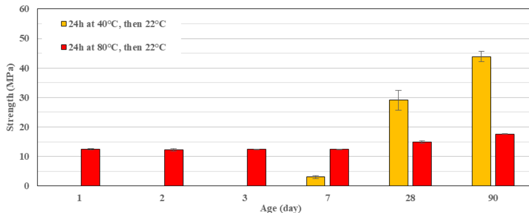
Figure 4.20: Influence of 24h heat treatment at different T^\circ . GGBS 4400 \text{ cm}^2/\text{g} with 2% \text{Na}_2\text{CO}_3 and 0.1% 4\text{Na}^*\text{HEDP} at \text{W/B}=0.40
