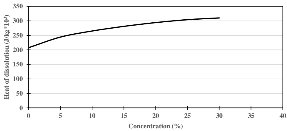
Figure 2.13: Effect of concentration on heat release over \text{Na}_2\text{CO}_3 dissolution at 25°C (GCIP, 2007)
