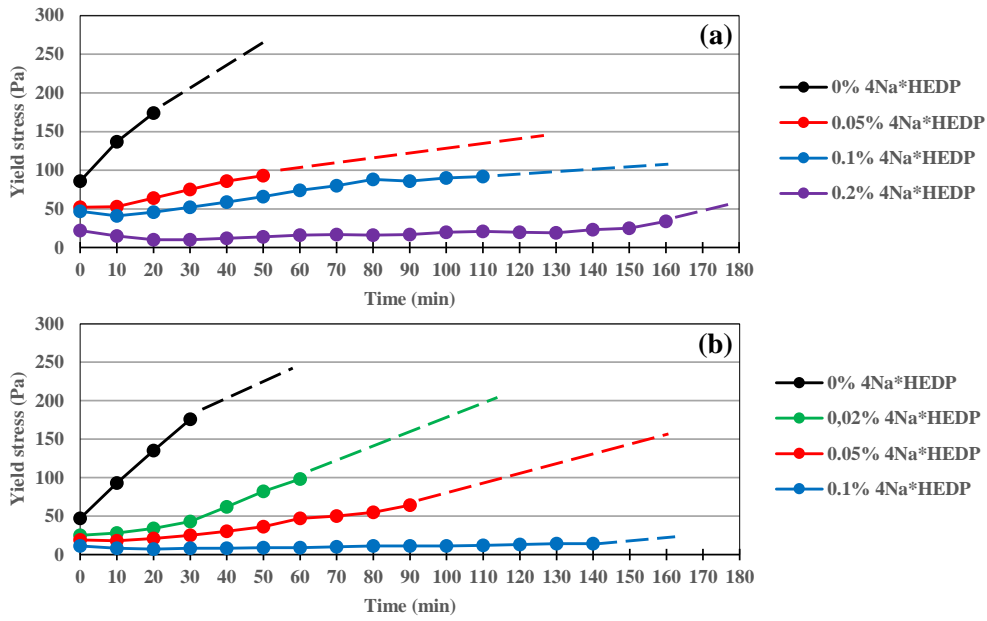
Figure 3.8: Yield stress evolution of GGBS activated with 2% \text{Na}_2\text{CO}_3 at W/B ratio 0.35 (a) and 0.40 (b) with addition of different dosages by GGBS weight of 4Na*HEDP
