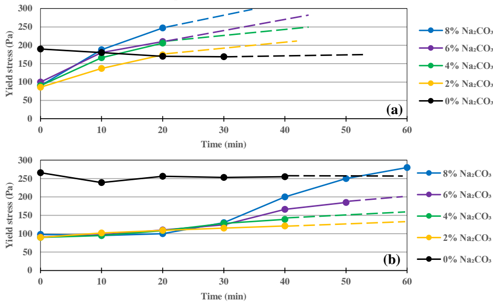
Figure 5.14: Yield stress evolution for different \text{Na}_2\text{CO}_3 amounts in the case of 100% GGBS (a) and 5% (b) replacement by Clinker 1400 \text{cm}^2/\text{g} at W/B=0.35
