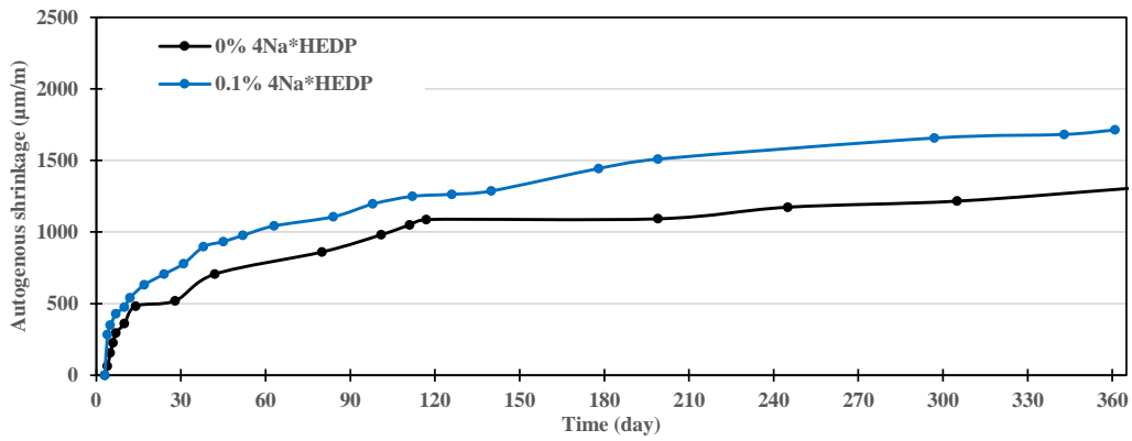
Figure 4.27: Influence of 4Na*HEDP on the autogenous shrinkage evolution of mortars based on GGBS activated with 8% \text{Na}_2\text{CO}_3 (200 g/l) at W/B=0.40
