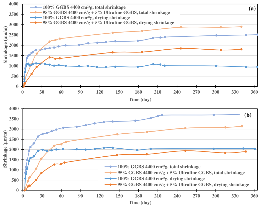
Figure 4.39: Influence of 5% GGBS replacement by Ultrafine GGBS on total and drying shrinkage stored at RH=50%. GGBS with 8% Na 2 CO 3 and 0.1% 4Na*HEDP. W/B=0.35 (a) and 0.40 (b)
