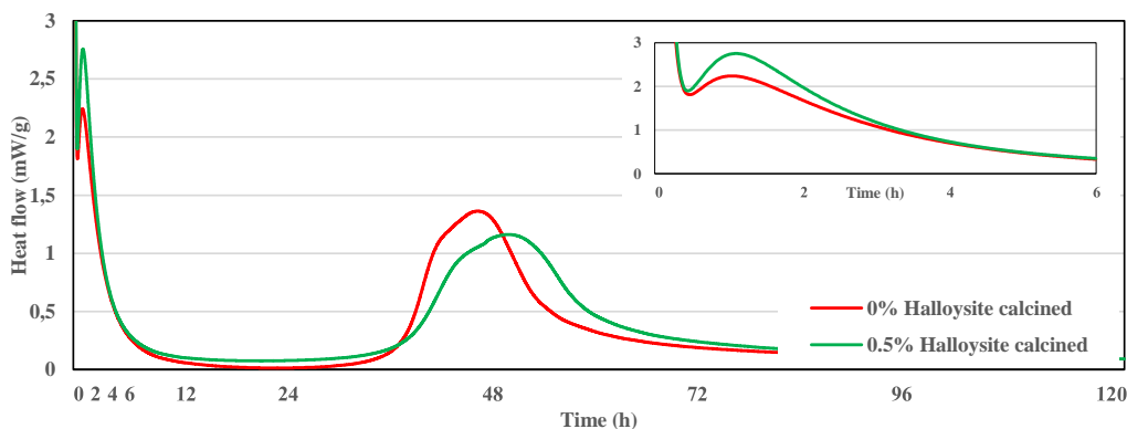
Figure 7.8: Hydration kinetics of 10% \text{Na}_2\text{CO}_3 activated GGBS with addition of calcined Halloysite ( W/B=0.40 )
