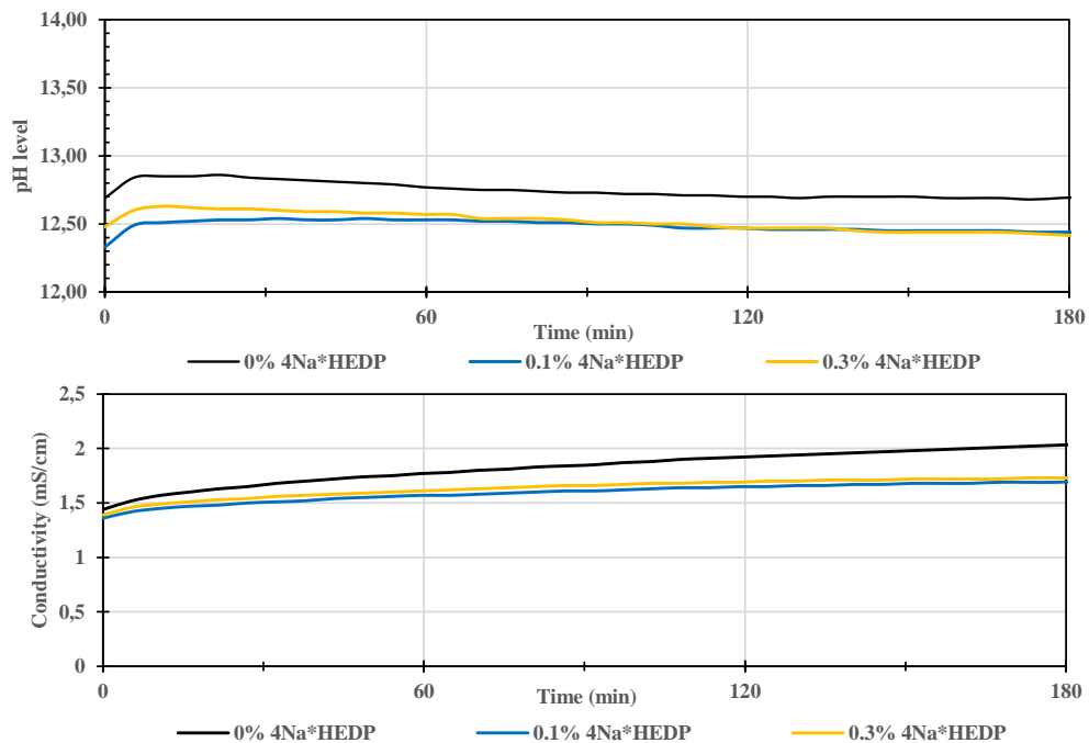
Figure 3.17: Evolution of pH level and conductivity of Standard GGBS with 8% \text{Na}_2\text{CO}_3 and different amount of 4Na*HEDP (W/B=100)
