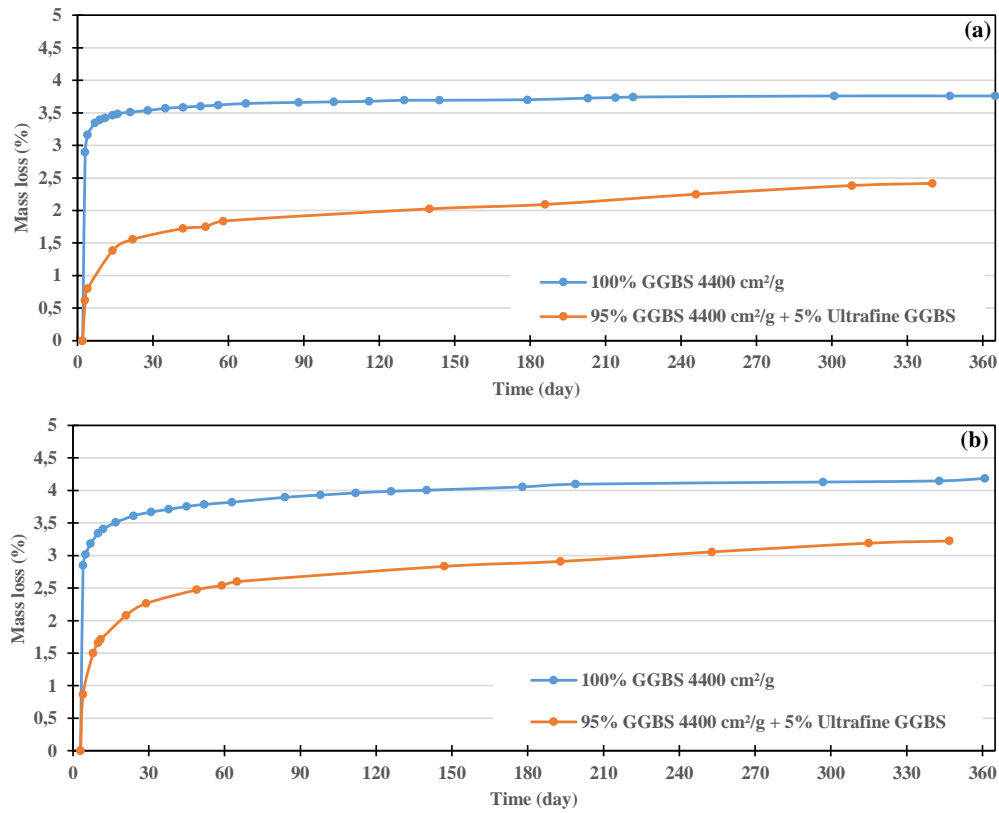
Figure 4.38: Influence of 5% GGBS replacement by Ultrafine GGBS on mass loss stored at RH=50%. GGBS with 8% Na 2 CO 3 and 0.1% 4Na*HEDP. W/B=0.35 (a) and 0.40 (b)
