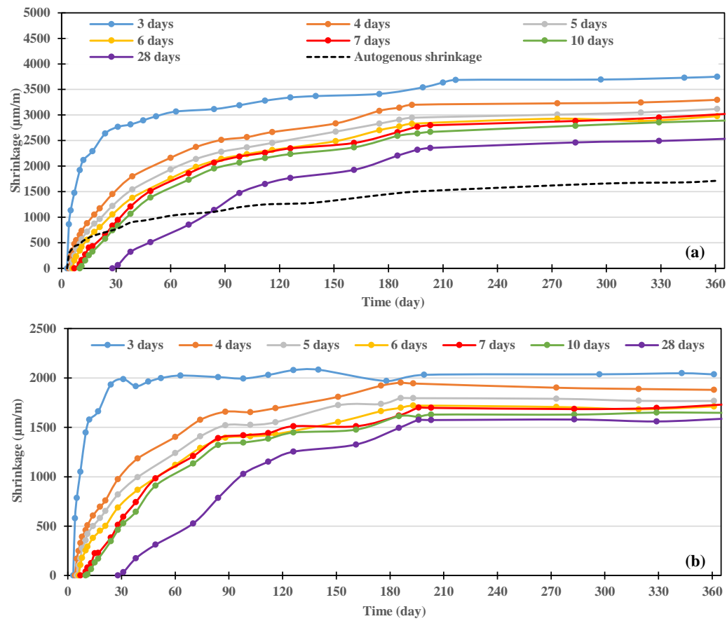
Figure 4.41: Influence of the duration of humid pre-curing on the afterwards dry curing ( \text{RH}=50\% ) on total (a) and net drying shrinkage (b) in the case of GGBS activated with 8% \text{Na}_2\text{CO}_3 in the presence of 0.1% 4\text{Na}^*\text{HEDP} at W/B=0.40
