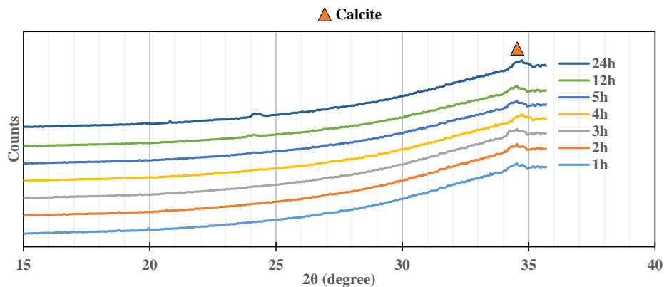
Figure 2.69: Synchrotron in-situ X-ray patterns evolution of GGBS activated with 50g/l \text{Na}_2\text{CO}_3
