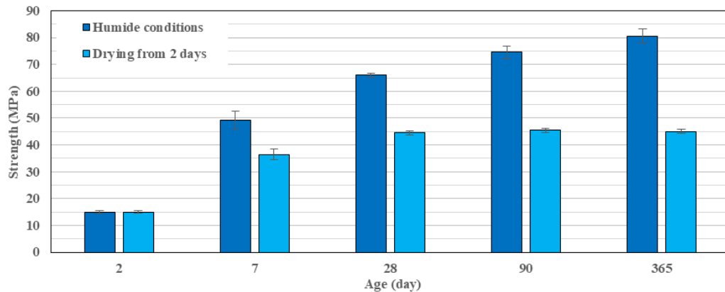
Figure 4.24: Strength development under dry conditions ( RH=50\% ) following 2 days curing in humid conditions in case of GGBS 4400 \text{ cm}^2/\text{g} with 8\% \text{ Na}_2\text{CO}_3 and 0.1\% 4\text{Na}^*\text{HEDP} at W/B=0.35
