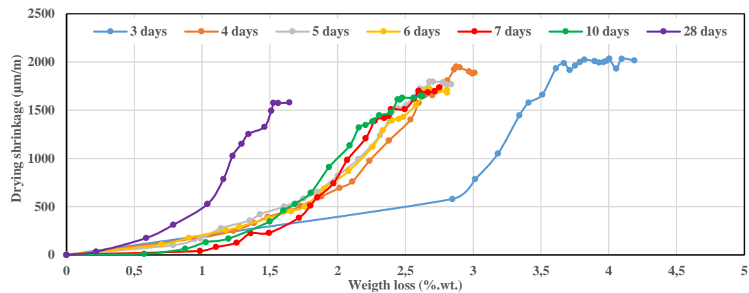
Figure 4.42: Net drying shrinkage as a function of weight loss for GGBS activated with 8% \text{Na}_2\text{CO}_3 in the presence of 0.1% 4\text{Na}^*\text{HEDP} at W/B=0.40 , for different durations of humid pre-curing preceding curing under dry conditions ( 50\%\text{RH} )
