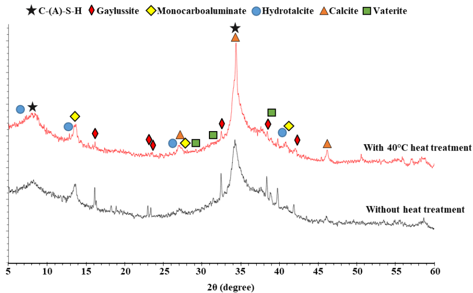
Figure 4.21: Influence of 10 days heat treatment at 40°C of 28 days old sample of GGBS with 8% Na 2 CO 3 and 0.1% 4Na*HEDP at W/B=0.40.
