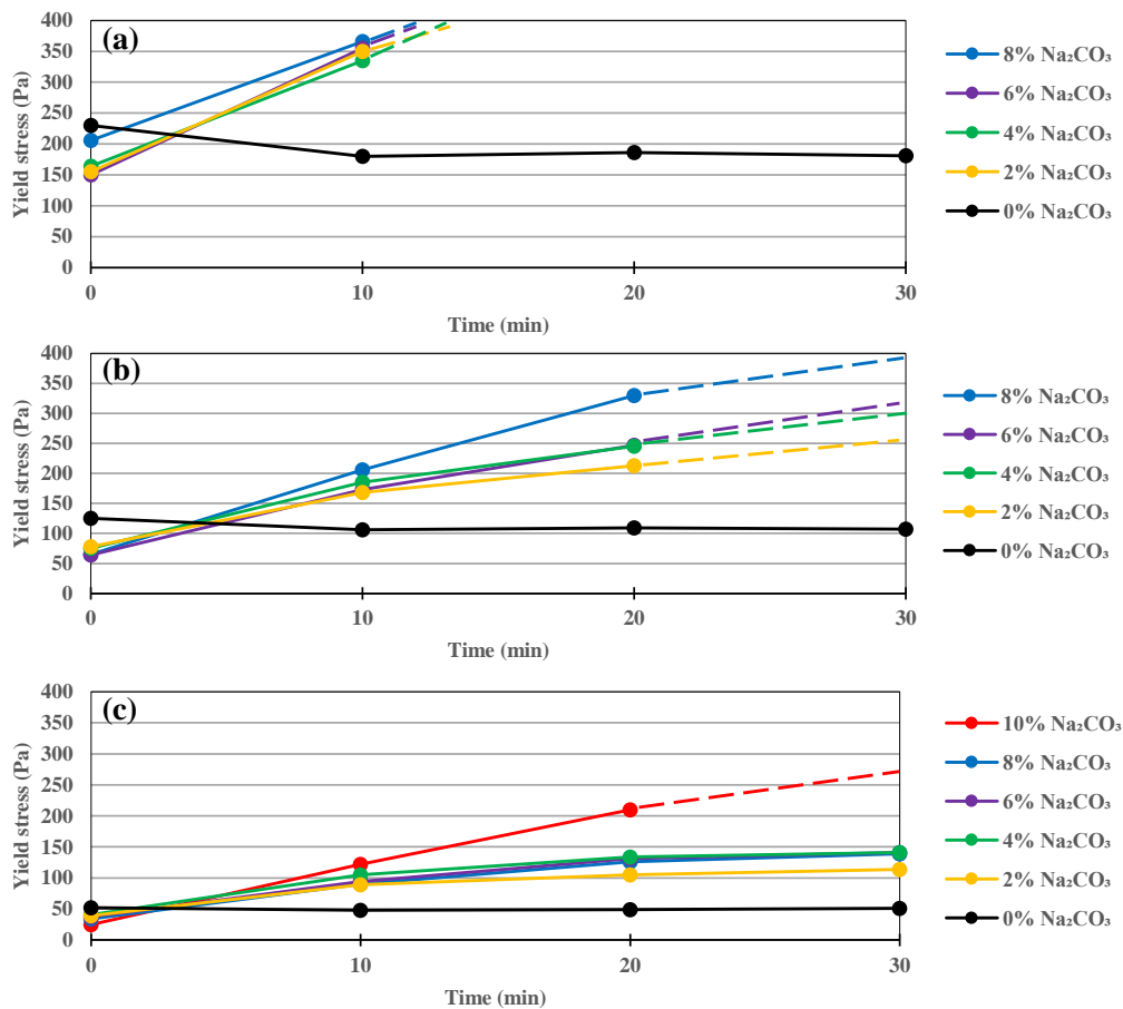
Figure 2.31: Yield stress evolution of GGBS 5600 cm²/g with different dosages of Na₂CO₃ and at W/B ratio of: 0.35 (a), 0.40 (b) and 0.45 (c)
