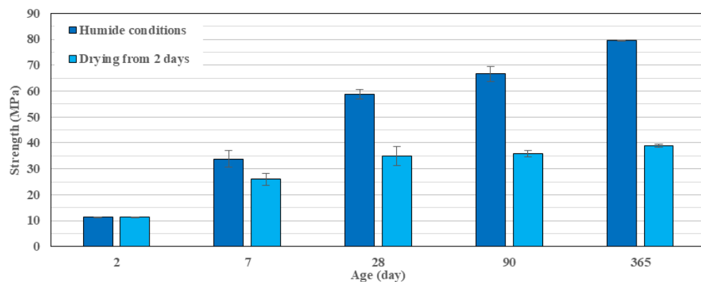
Figure 4.25: Strength development under dry conditions ( RH=50\% ) following 2 days curing in humid conditions in case of GGBS 4400 \text{ cm}^2/\text{g} with 6\% \text{ Na}_2\text{CO}_3 and 0.1\% 4\text{Na}^*\text{HEDP} at W/B=0.35
