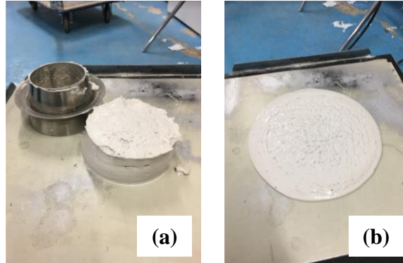
Figure 2.29: Mini-cone slump test: GGBS paste with 8% \text{Na}_2\text{CO}_3 at \text{W/B}=0.40 before (a) and after (b) vibration at the age of 50 minutes.
