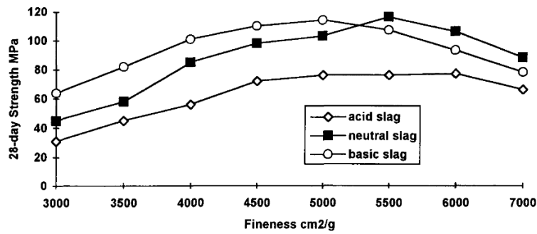
Figure 1.14: Fineness vs. 28-day strength for different types of slag (Waterglass activator, \text{Na}_2\text{O}=5.5\% ; M_s=1 ; sand/slag=2; slag fineness variation= \pm 300 \text{ cm}^2/\text{g} ) (Wang et al., 1994)
