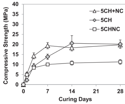
Figure 1.7: Compressive strength evolution of slag activated by 6.25% \text{Ca}(\text{OH})_2 (5CH), 6.25% \text{Ca}(\text{OH})_2 + 3\%\text{Na}_2\text{CO}_3 (5CH+NC) or 3% \text{Ca}(\text{OH})_2 + 3.25\%\text{Na}_2\text{CO}_3 (5CHNC) weighted by slag at \text{W/B}=0.5 (Jeong et al., 2016)
