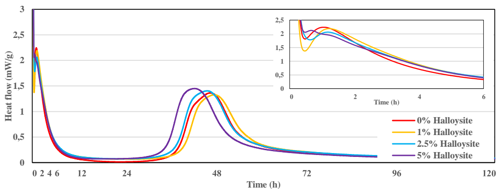
Figure 7.7: Hydration kinetics of GGBS activated with 10% \text{Na}_2\text{CO}_3 at W/B=0.40 with various amounts of Halloysite
