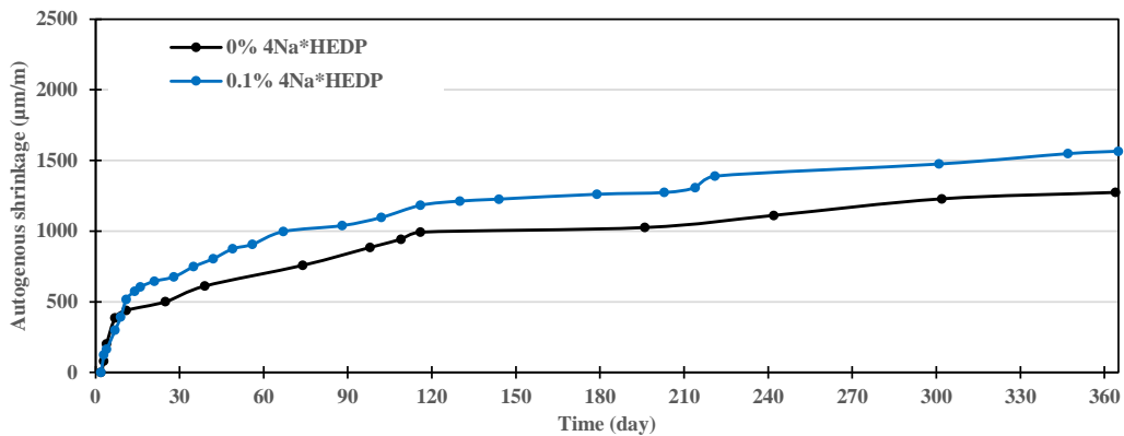
Figure 4.28: Influence of 4Na*HEDP on the autogenous shrinkage evolution of mortars based on GGBS activated with 8% \text{Na}_2\text{CO}_3 with (230 g/l) at W/B=0.35
