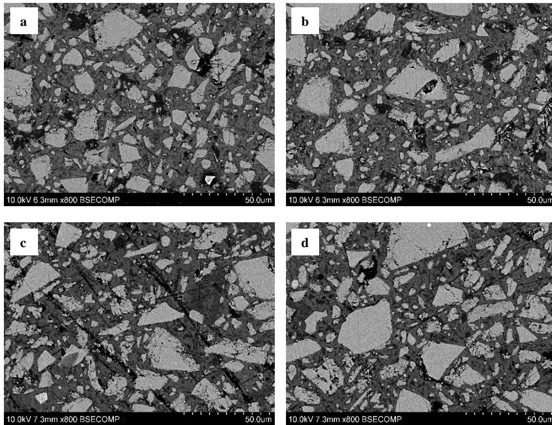
Figure 5.88: SEM observations of polished surface. Comparison between 0% (a,b) and 5% (c,d) GGBS replacement by coarse clinker at 28 days. 8%Na 2 CO 3 and 0.1% 4Na*HEDP at W/B=0.40
