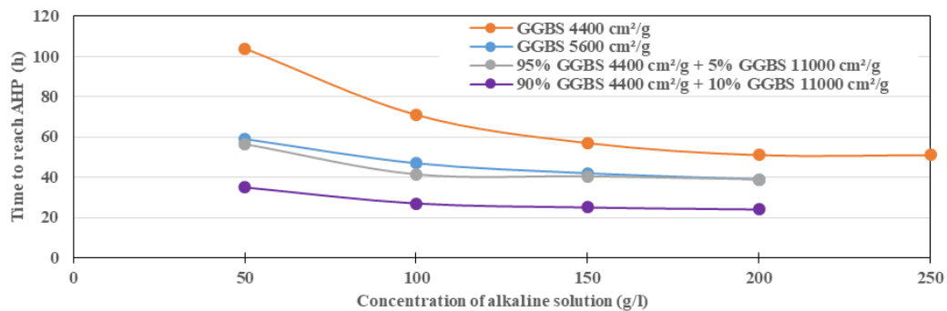
Figure 2.53: Time to rich the main hydration peak for different GGBS fineness at constant Water/GGBS ratio of 0.40 as a function of sodium carbonate concentration
