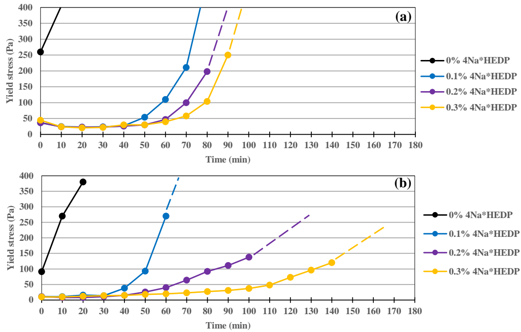
Figure 3.12: Influence of 4Na*HEDP on yield stress evolution of paste: 95% GGBS + 5% Ultrafine GGBS with 8% \text{Na}_2\text{CO}_3 at W/B ratio of 0.35 (a) and 0.40 (b)
