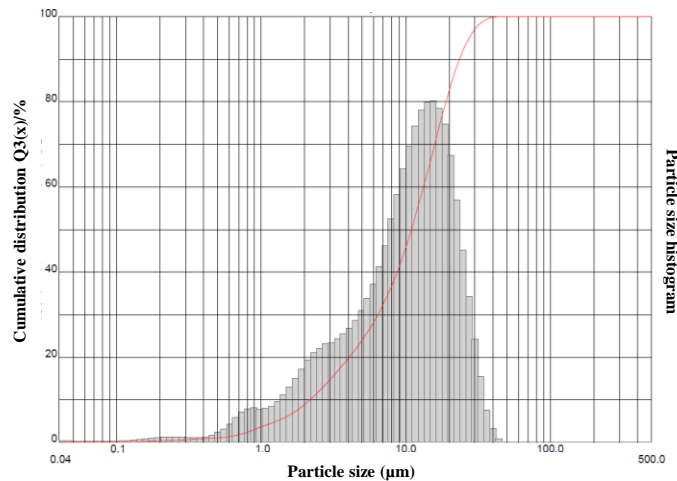
Figure 2.2: Particle size distribution of Standard GGBS
