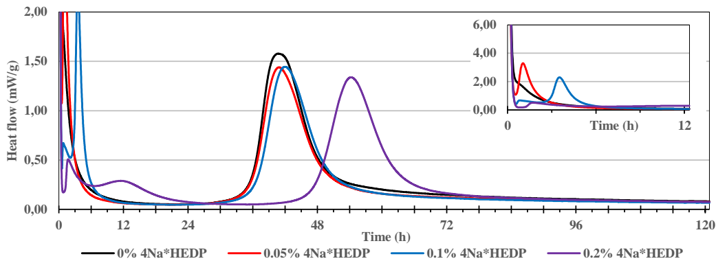
Figure 3.25: Influence of 4Na*HEDP on the hydration kinetics of GGBS 5600 cm²/g activated with 6% Na₂CO₃ at W/B=0.40
