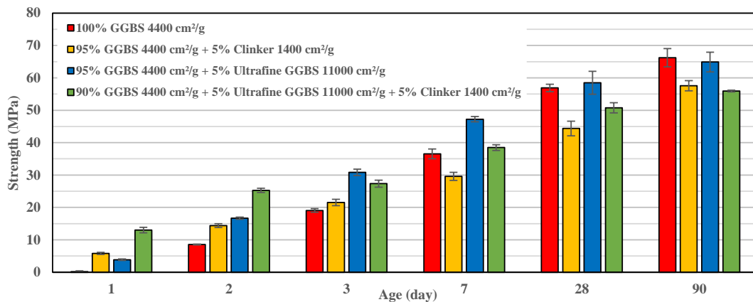
Figure 5.59: Influence of the combination of Ultrafine GGBS and coarse Clinker 1400 cm²/g substitution on the strength development at W/B=0.40, 8% Na 2 CO 3 (200g/l) and 0.1% 4Na*HEDP
