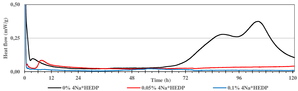
Figure 3.23: Released heat upon hydration of GGBS activated with 2% \text{Na}_2\text{CO}_3 in the presence of 4Na*HEDP at W/B=0.40
