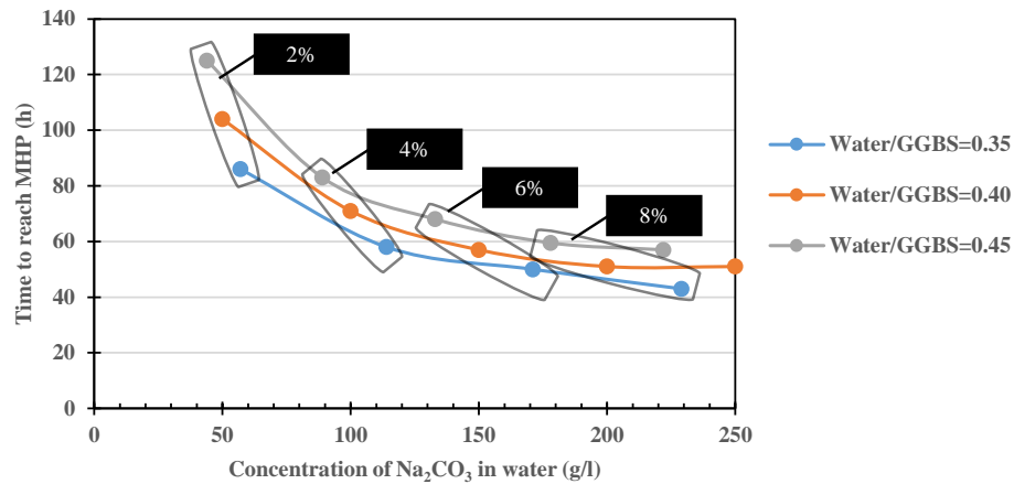
Figure 2.39: Time to reach the main hydration peak (MHP) as a function of \text{Na}_2\text{CO}_3 aqueous concentration. The black squares indicate the percentage of the activator relative to GGBS mass
