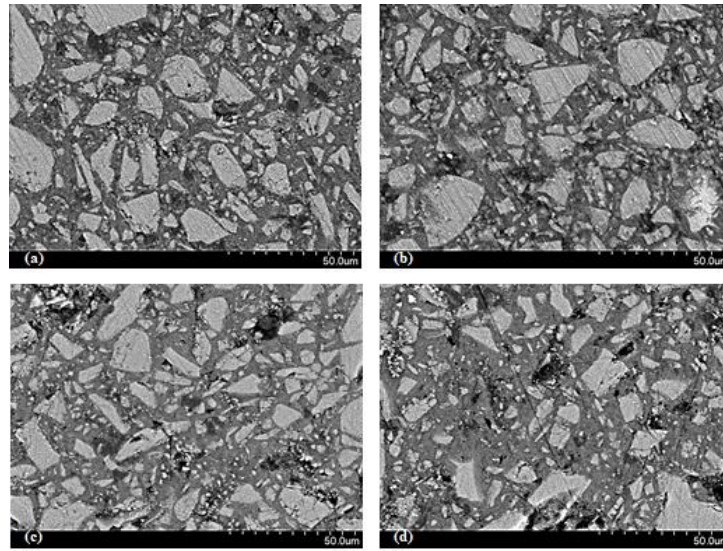
Figure 3.34: Influence of 4Na*HEDP on the microstructure (through SEM imaging) of GGBS activated with 8% \text{Na}_2\text{CO}_3 without (a-b) and with 0.3% (c-d) 4Na*HEDP, at the age of 28 days at W/B=0.35
