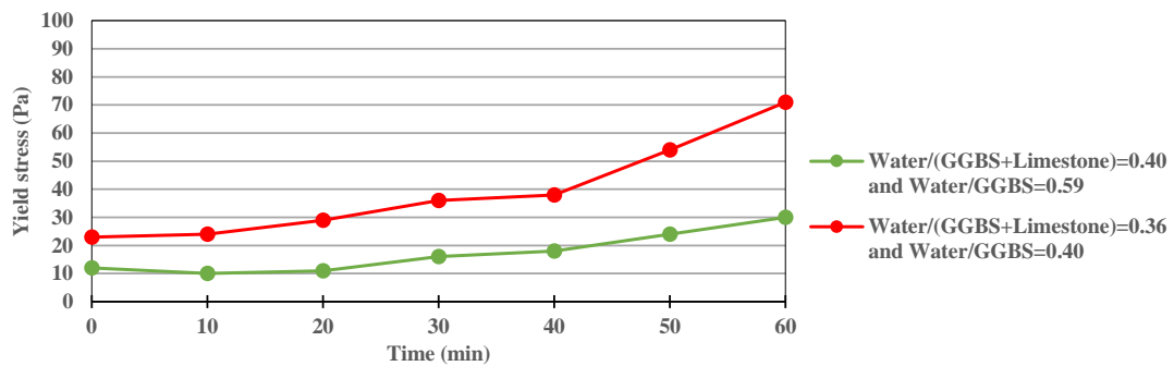
Figure 6.17: Influence of 10% GGBS replacement by ultrafine limestone at \text{Water}/(\text{GGBS}+\text{Limestone})=0.40 or 0.36 and 8\%\text{Na}_2\text{CO}_3 to GGBS or to GGBS+Limestone to keep concentration of 200g/l with 0.1% 4Na*HEDP
