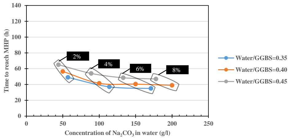
Figure 2.49: Time to reach the main hydration peak (MHP) for GGBS with 5% replacement by Ultrafine GGBS by mass as a function of \text{Na}_2\text{CO}_3 concentration in water.
