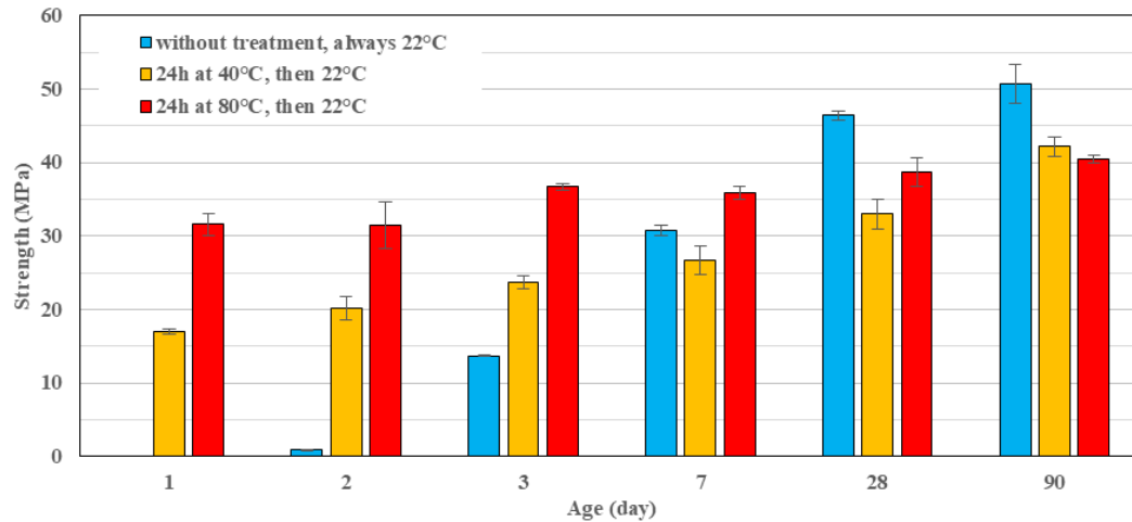
Figure 4.19: Influence of 24h heat treatment at different T^\circ . GGBS 4400 \text{ cm}^2/\text{g} with 6% \text{Na}_2\text{CO}_3 (150 g/l) and 0.1% 4\text{Na}^*\text{HEDP} at \text{W/B}=0.40
