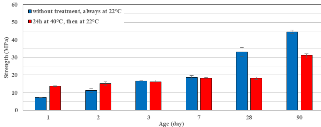
Figure 5.64: Influence of heat treatment at 40^\circ\text{C} over 24h for mortars based on GGBS with 5% replacement by coarse Clinker 1400\text{ cm}^2/\text{g} at \text{W/B}=0.40 , 6% \text{Na}_2\text{CO}_3 (150g/l) and 0.1% 4Na*HEDP
