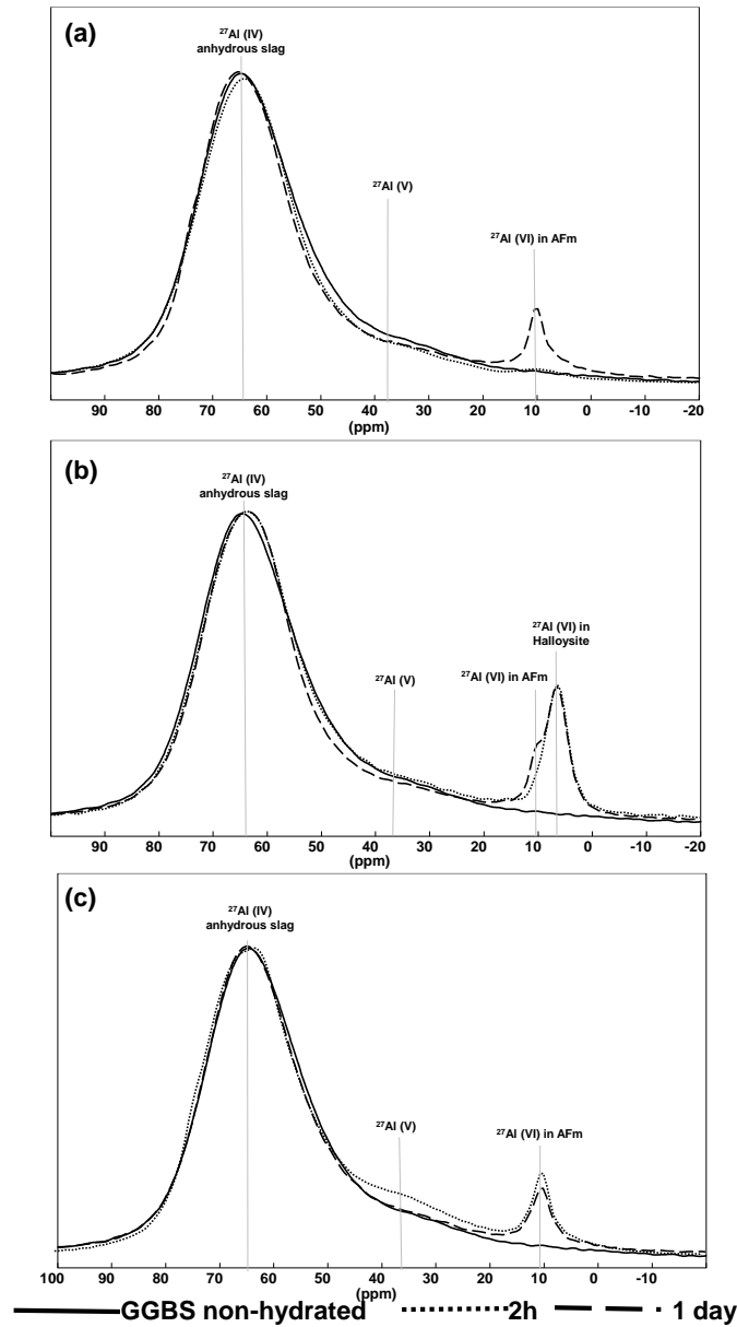
Figure 7.16: ^{27}\text{Al} MAS NMR spectra at 2 hours and 1 day for pure GGBS (a) or with addition of 2.5% Halloysite (b) and 1% \text{NaAlO}_2 (c) at \text{W/B}=0.40 and 10% \text{Na}_2\text{CO}_3
