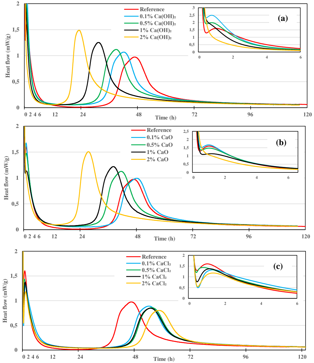
Figure 5.7: Comparison of hydration kinetics in case of partial GGBS replacement by various calcium sources: \text{Ca(OH)}_2 (a), \text{CaO} (b) and \text{CaCl}_2 (c). W/B=0.40 with 10% \text{Na}_2\text{CO}_3 (250 g/l)
