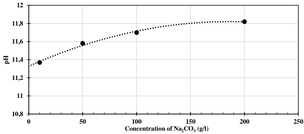
Figure 2.12: pH level of solution as a function of anhydrous \text{Na}_2\text{CO}_3 concentration in water at 20°C
