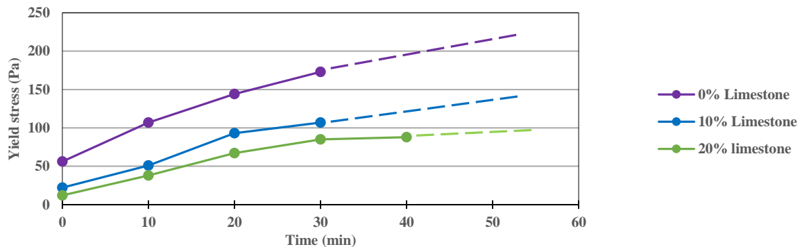
Figure 6.6: Influence of partial GGBS replacement by fine limestone on yield stress evolution at \text{Water}/(\text{GGBS} + \text{Limestone}) = 0.40 and 8\% \text{ Na}_2\text{CO}_3 to dry components ( 200 \text{ g/l} ).
