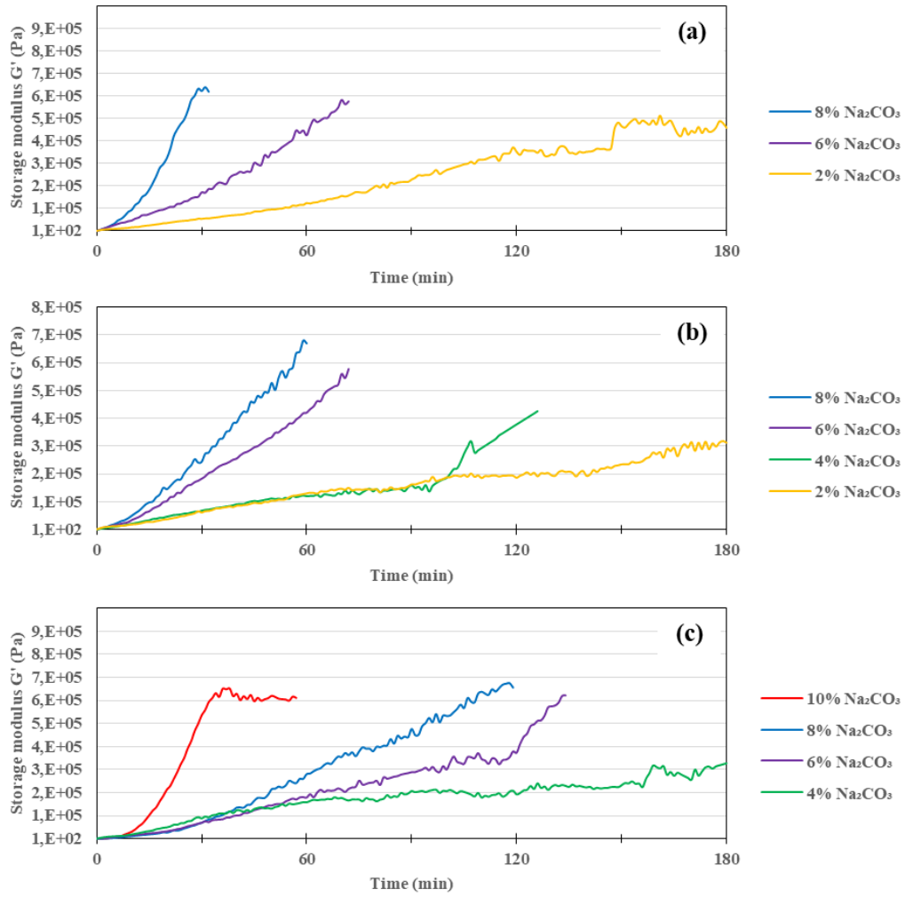
Figure 2.32: Storage modulus evolution of Fine GGBS with different amount Na_2CO_3 and W/B ratio of: 0.35 (a), 0.40 (b) and 0.45 (c)
