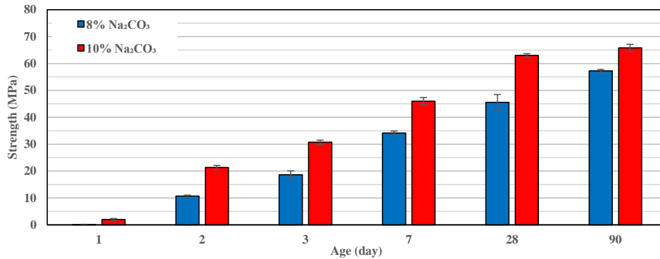
Figure 2.60: Influence of \text{Na}_2\text{CO}_3 amount on compressive strength development of mortars based on 100% GGBS 4400 \text{cm}^2/\text{g} at \text{W/B}=0.40
