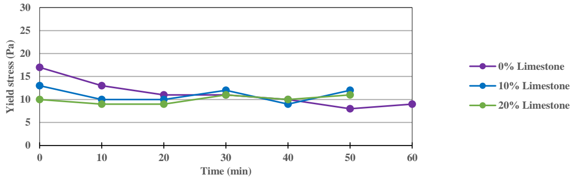
Figure 6.7: Influence of partial GGBS replacement by fine limestone on yield stress evolution at \text{Water}/(\text{GGBS}+\text{Limestone})=0.40 , 8% \text{Na}_2\text{CO}_3 (200 g/l) and 0.1% 4\text{Na}^*\text{HEDP} to dry components
