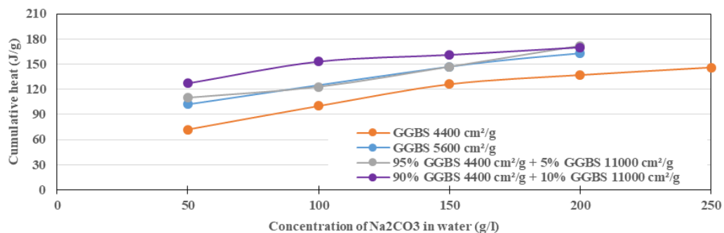
Figure 2.54: Cumulative heat released after 120h of hydration as a function of aqueous sodium carbonate concentration for different GGBS fineness at the same Water/GGBS ratio of 0.40
