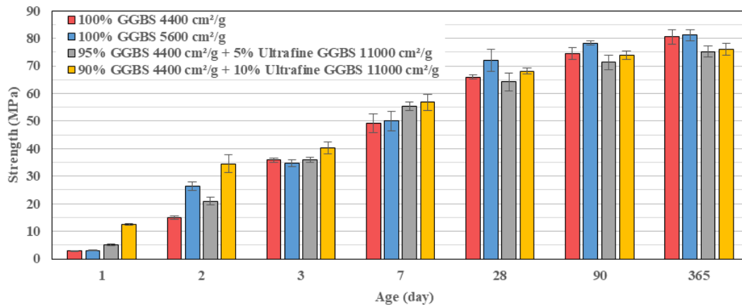
Figure 4.13: Comparison of strength evolution for different GGBS fineness. 8% \text{Na}_2\text{CO}_3 (200 g/l) and 0.1% 4\text{Na}^*\text{HEDP} were used at \text{W/B}=0.35
