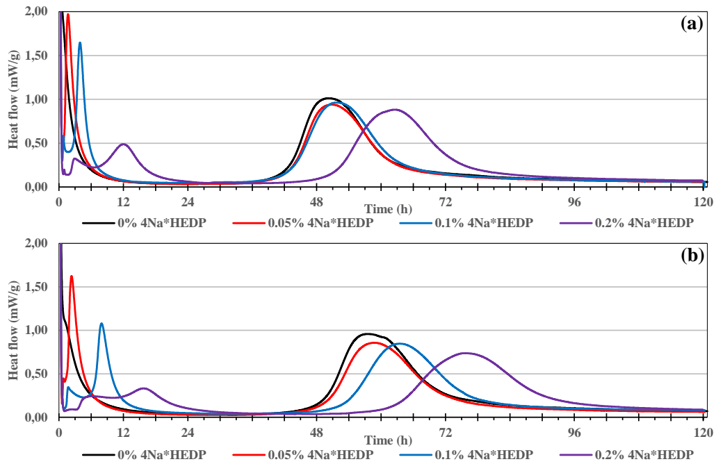
Figure 3.22: Hydration kinetics of GGBS with 6% \text{Na}_2\text{CO}_3 and with different dosage of 4Na*HEDP at Water/GGBS ratio of 0.35 (a) and 0.40 (b)
