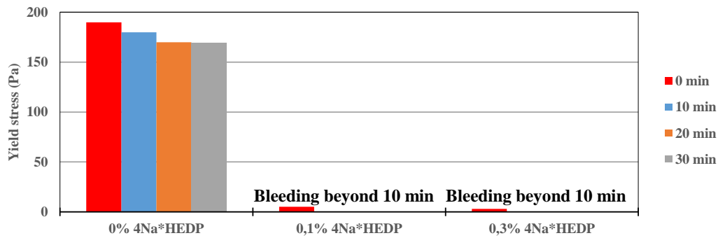
Figure 3.9: Influence of 4Na*HEDP on yield stress of GGBS with 0% \text{Na}_2\text{CO}_3 at W/B=0.35
