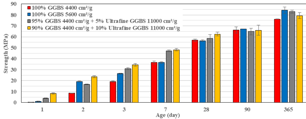
Figure 4.12: Comparison of strength evolution for different GGBS fineness. 8% \text{Na}_2\text{CO}_3 and 0.1% 4\text{Na}^*\text{HEDP} were used at \text{W/B}=0.40
