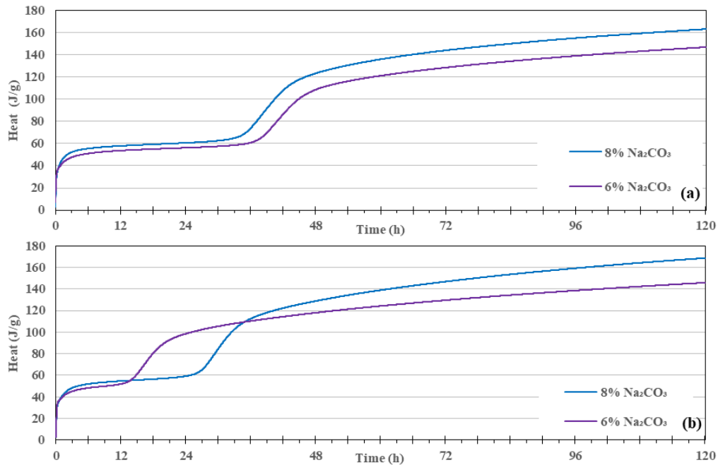
Figure 5.43: Heat released from hydration of GGBS 5600 cm 2 /g Blaine without (a) and with 5% (b) replacement by clinker 1400 cm 2 /g at W/B=0.40
