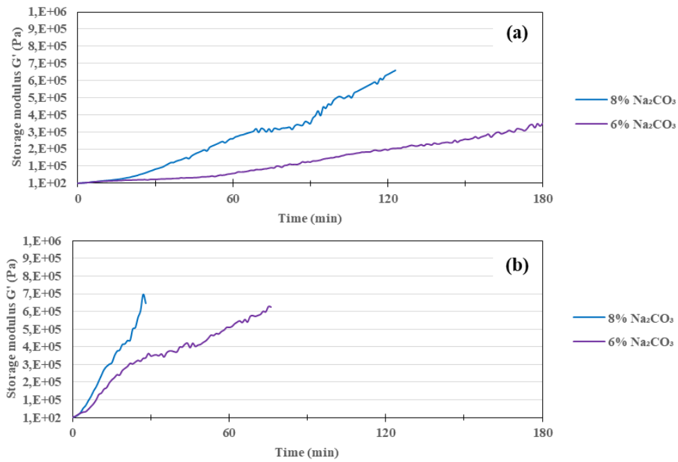
Figure 2.35: Comparison of storage modulus evolution in case of 100% GGBS (a) and with 10% replacement by Ultrafine GGBS (b) with different amounts of \text{Na}_2\text{CO}_3 and \text{W/B}=0.45
