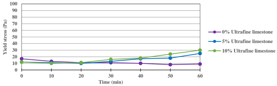
Figure 6.16: Influence of partial GGBS replacement by ultrafine limestone on yield stress evolution at \text{Water}/(\text{GGBS}+\text{Limestone})=0.40 and 8\%\text{Na}_2\text{CO}_3 (200g/l) in the presence of 0.1% 4Na*HEDP
