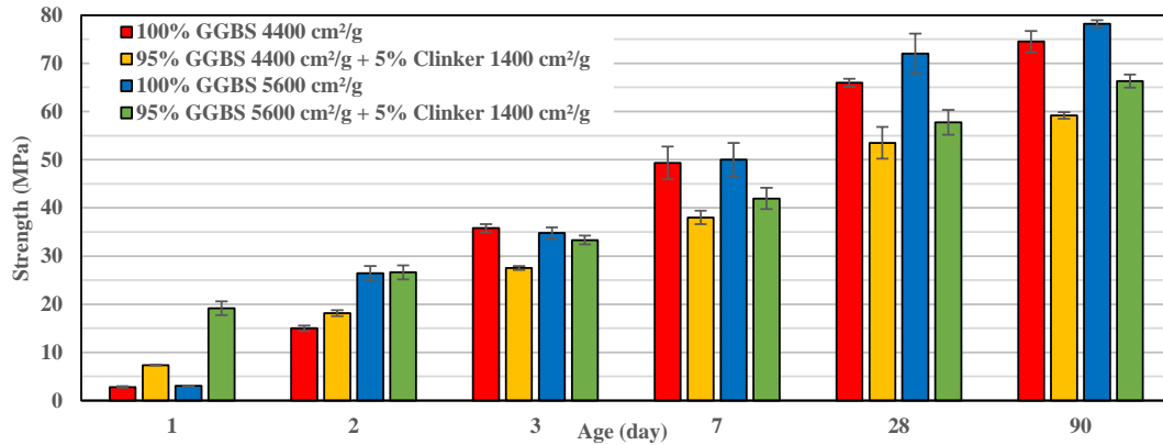
Figure 5.58: Comparison of 5% GGBS replacement by clinker 1400 cm²/g in case of two different GGBS fineness (4400 and 5600 cm²/g) at W/B=0.35, 8% Na 2 CO 3 (230g/l) and 0.1% 4Na*HEDP
