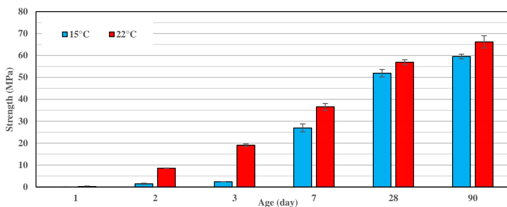
Figure 4.15: Influence of storage temperature 22°C versus 15°C on strength evolution of GGBS 4400 cm²/g with 8% \text{Na}_2\text{CO}_3 and 0.1% 4Na*HEDP at W/B=0.40
