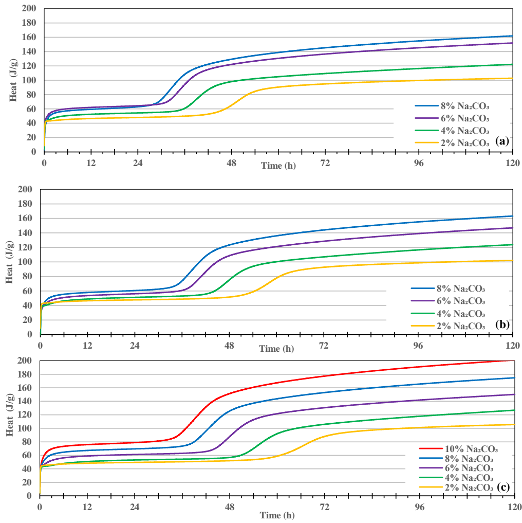
Figure 2.45: Heat released after hydration of GGBS 5600 cm²/g with different quantity of Na₂CO₃ at Water/GGBS ratio: 0.35 (a); 0.40 (b) and 0.45 (c).
