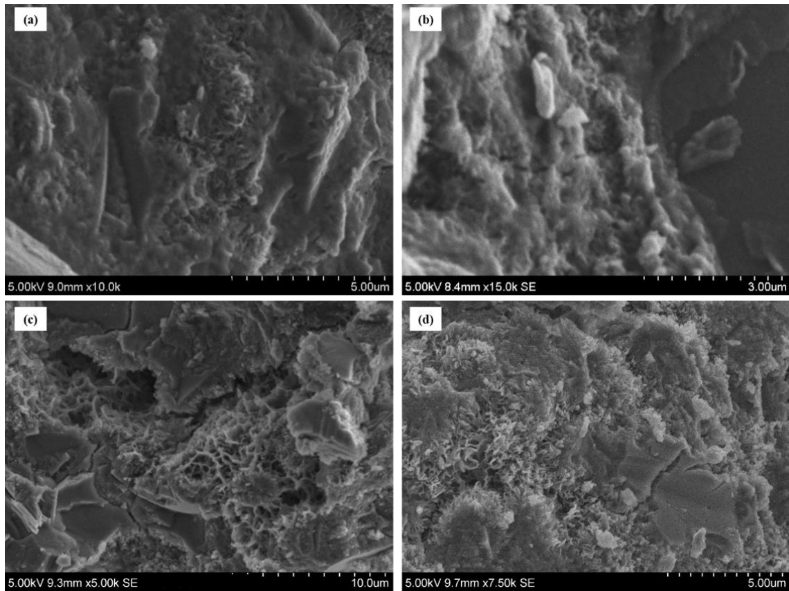
Figure 5.89: SEM observations of fault surface. Comparison between 0% (a,b) and 5% (c,d) GGBS replacement by coarse clinker at the age of 28 days. 8%Na 2 CO 3 and 0.1% 4Na*HEDP at W/B=0.40
