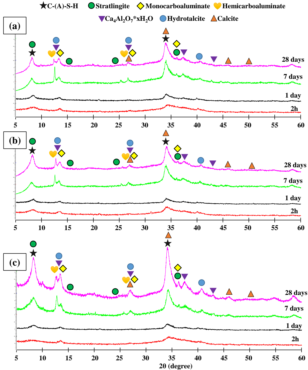
Figure 7.15: XRD patterns of pure GGBS (a) or with 2.5% Halloysite (b) and 1% \text{NaAlO}_2 (c) addition at W/B=0.45 and 8% \text{NaOH}
