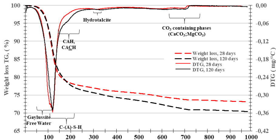
Figure 3.33: Evolution of TG-DTG curves at long term for GGBS activated with 8% \text{Na}_2\text{CO}_3 at \text{W/B}=0.40 with 0.1% 4Na*HEDP. Comparison between 28 and 120 days
