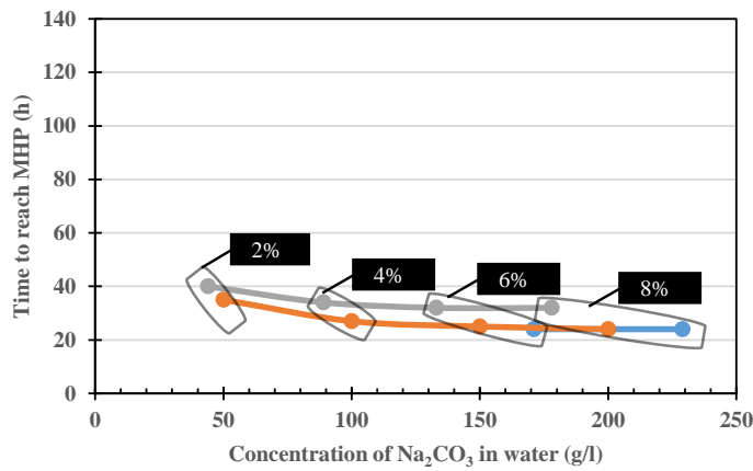
Figure 2.50: Time to reach the main hydration peak (MHP) for GGBS with 10% replacement by Ultrafine GGBS by mass as a function of \text{Na}_2\text{CO}_3 concentration
