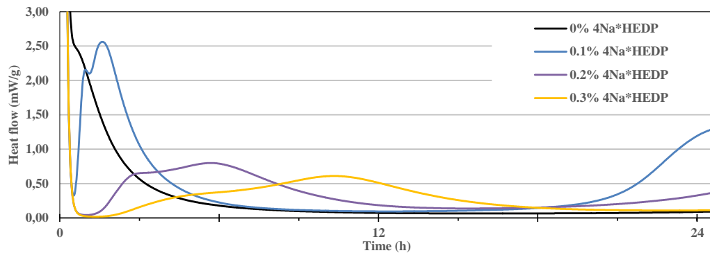
Figure 5.33: Influence of 4Na*HEDP dosage on hydration kinetics for the first 24h in case of 5% GGBS replacement by clinker 1400 cm 2 /g at W/B=0.40 and 8% Na 2 CO 3
