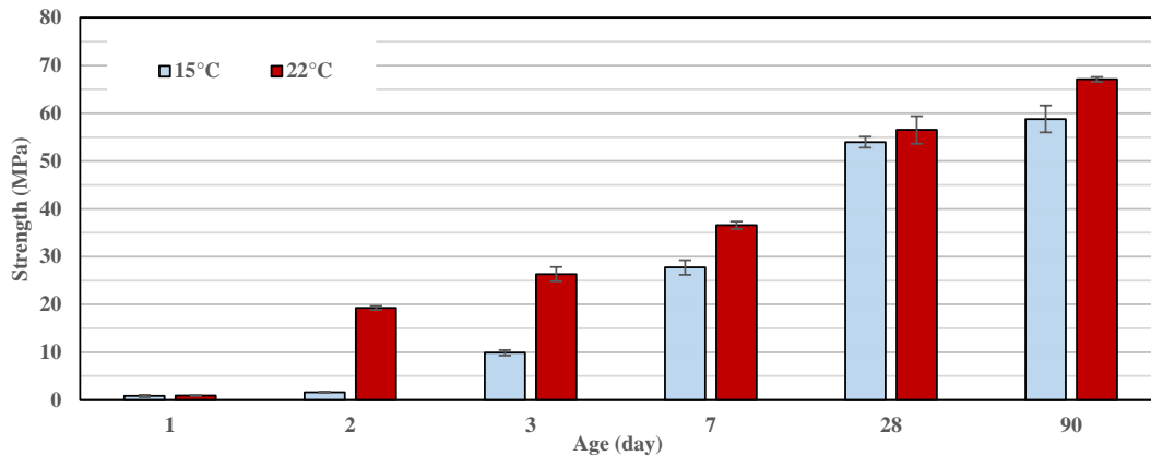
Figure 4.16: Influence of storage temperature 22°C versus 15°C on strength evolution of GGBS 5600 \text{cm}^2/\text{g} with 8% \text{Na}_2\text{CO}_3 and 0.1% 4Na*HEDP at W/B=0.40
