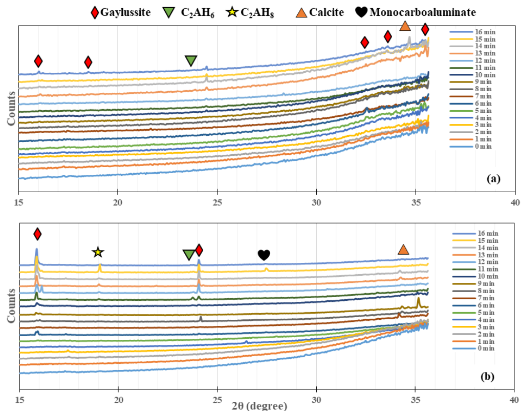
Figure 5.81: Synchrotron in-situ XRD patterns over the very first minutes of hydration for GGBS with 5% replacement by clinker 1400 (a) or 6000 (b) cm 2 /g. Solution: 200 g/l Na 2 CO 3 with 0.1% 4Na*HEDP
