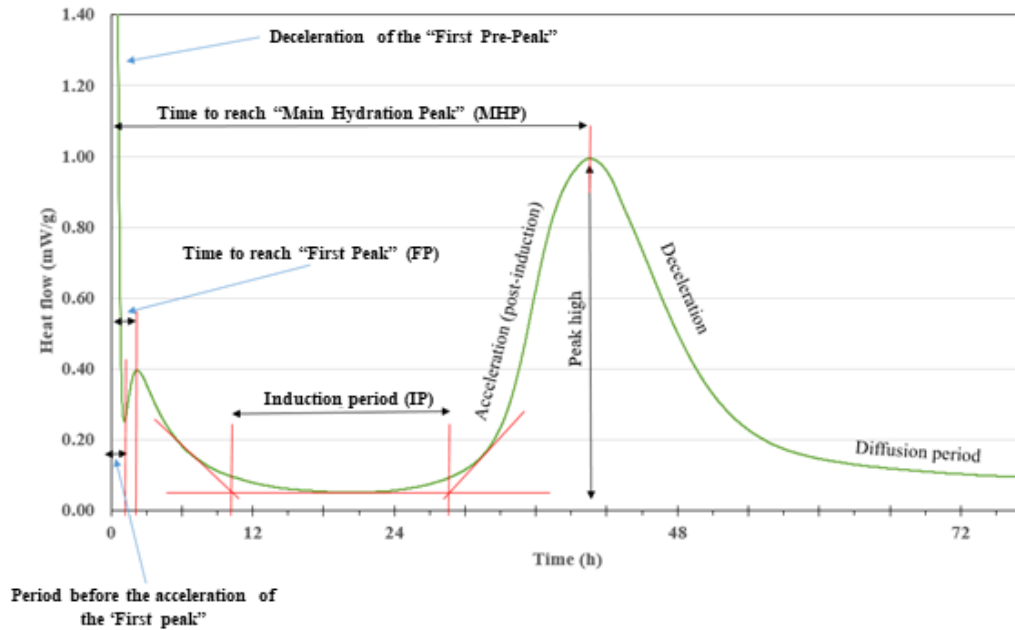
Figure 2.37: Schematic representation of heat evolution during \text{Na}_2\text{CO}_3 activated GGBS hydration with indication of zone of interest
