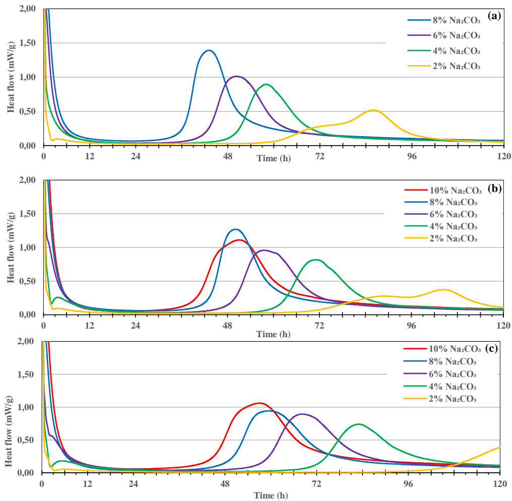
Figure 2.38: Heat evolution of GGBS with different Na 2 CO 3 dosages at W/B ratio of: 0.35 (a), 0.40 (b) and 0.45 (c)
