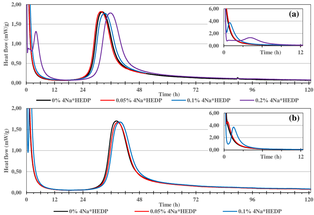
Figure 3.24: Influence of 4Na*HEDP on the hydration kinetics of GGBS 5600 cm²/g activated with 8% Na₂CO₃ at W/B ratio of 0.35 (a) and 0.40 (b)
