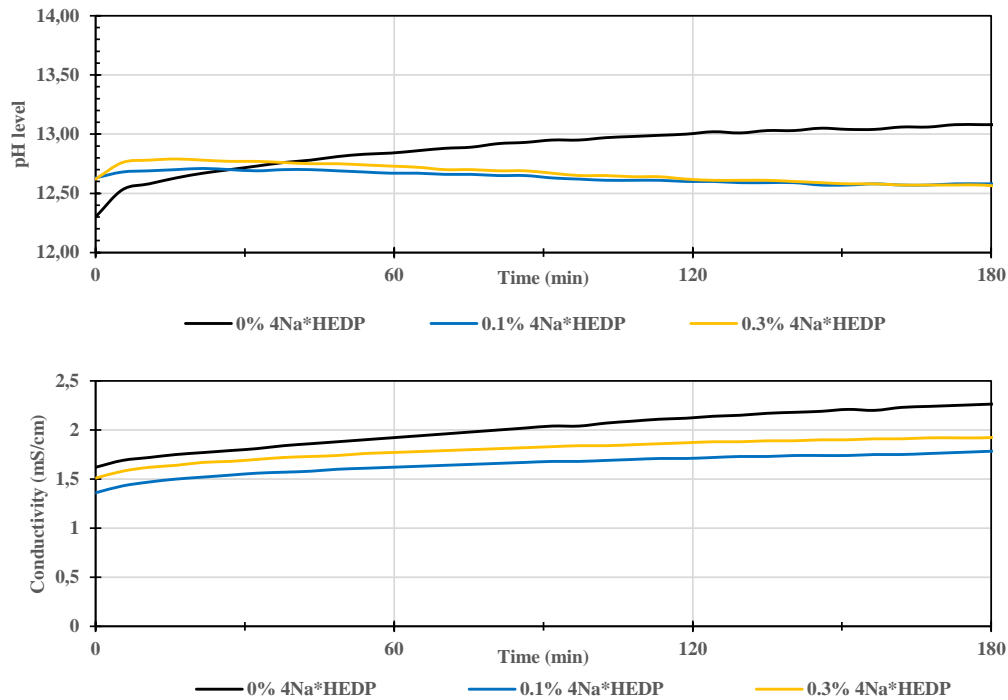
Figure 3.19: Evolution of pH level and conductivity of GGBS 5600 cm 2 /g with 8% Na 2 CO 3 and different amount of 4Na*HEDP (W/B=100)
