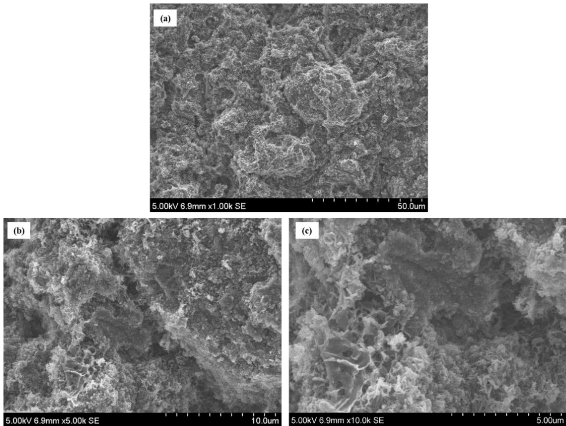
Figure 5.90: SEM observations of fault surface. GGBS with 5% replacement by coarse clinker at the age of 28 days. 2%Na 2 CO 3 and 0.1% 4Na*HEDP at W/B=0.40
