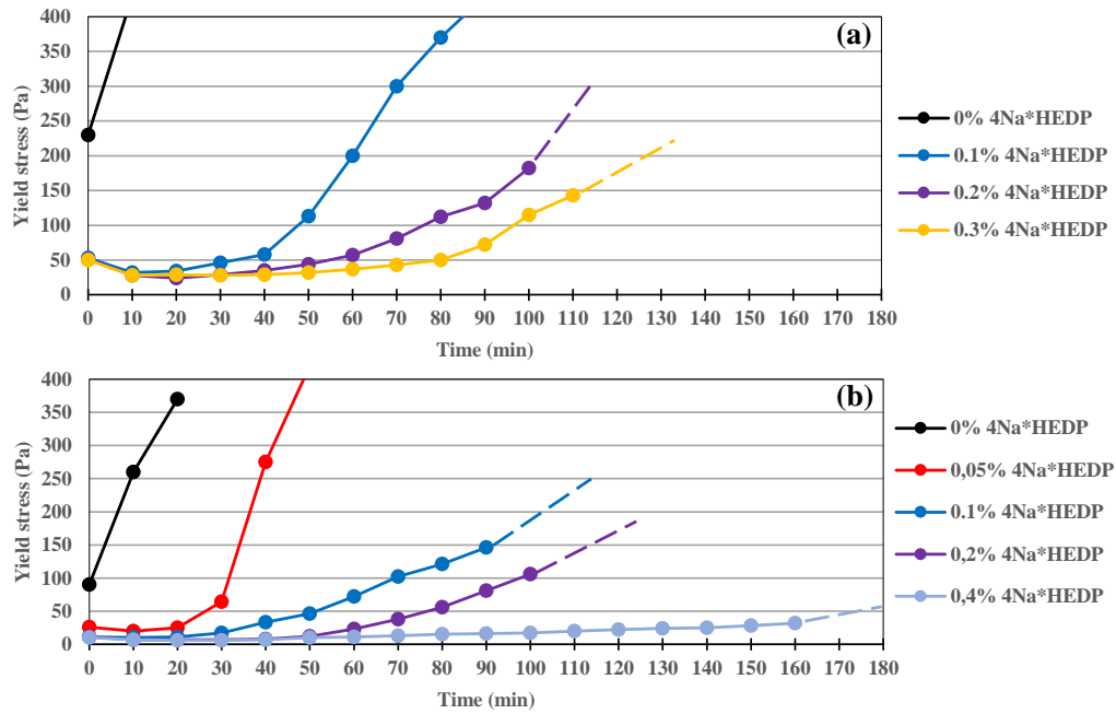
Figure 3.13: Influence of 4Na*HEDP on yield stress evolution of paste: 95% GGBS + 5% Ultrafine GGBS with 6% \text{Na}_2\text{CO}_3 at W/B ratio of 0.35 (a) and 0.40 (b)
