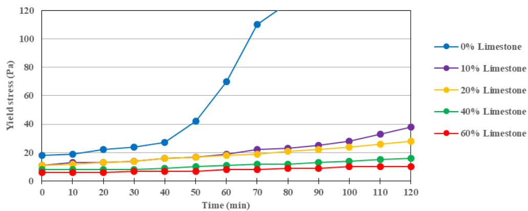
Figure 6.8: Influence of partial replacement of 95%GGBS+5%Clinker mix by fine limestone on yield stress evolution at \text{W/B}=0.40 , 0.1% 4\text{Na}^*\text{HEDP} and 6% \text{Na}_2\text{CO}_3 (150g/l) to total dry mix
