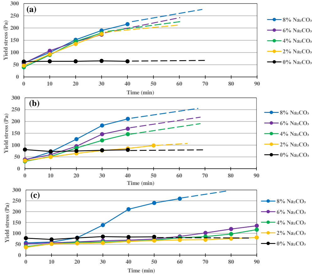
Figure 5.13: Yield stress evolution for different \text{Na}_2\text{CO}_3 amounts in the case of 100% GGBS (a), with 1% (b) and 5% (c) replacement by Clinker 1400 \text{cm}^2/\text{g} at W/B=0.40
