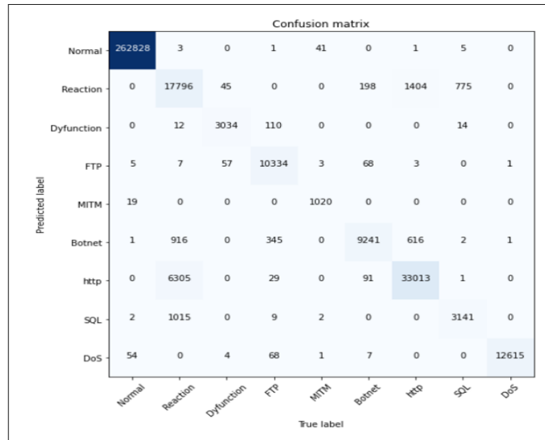
Figure 3.12 – Confusion matrix
