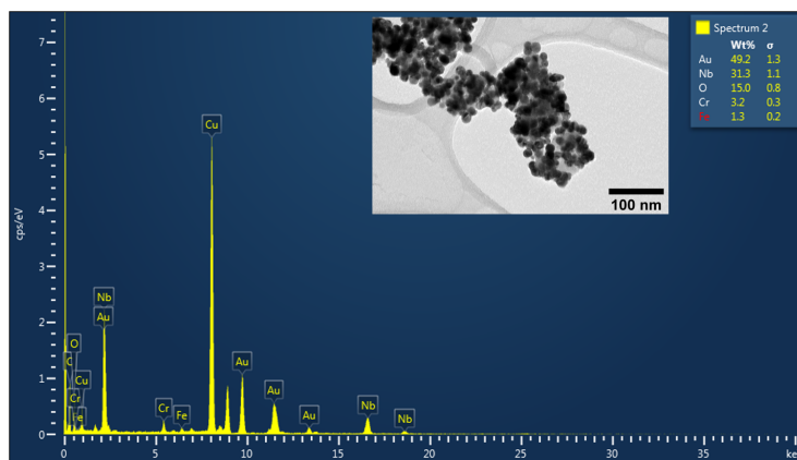
Figure 2.5: EDS spectrum of the elements identified by the characteristic X-rays emitted (using the Siegbahn notation) upon a focused spot electron beam on the sample shown in the TEM image included. Spectrum shows the peaks for Nb at 16.6 and 18.6 keV, Au at 9.7 and 11.4 keV. The spectrum also shows peaks for O, Cu, Cr and Fe, which are from the TEM grid.
