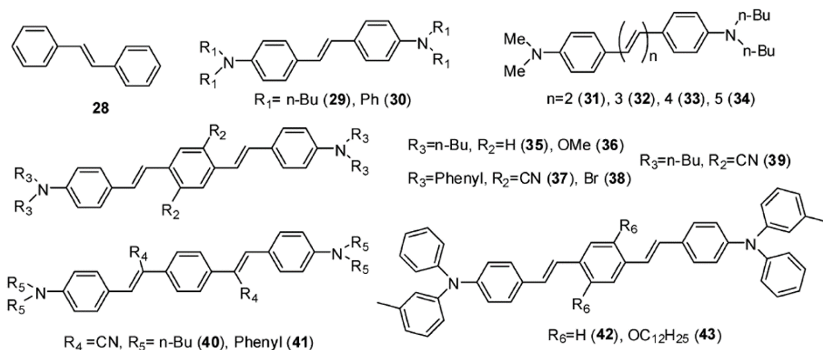
Figure 1.12: Examples of TPEF active organic molecules. 60
