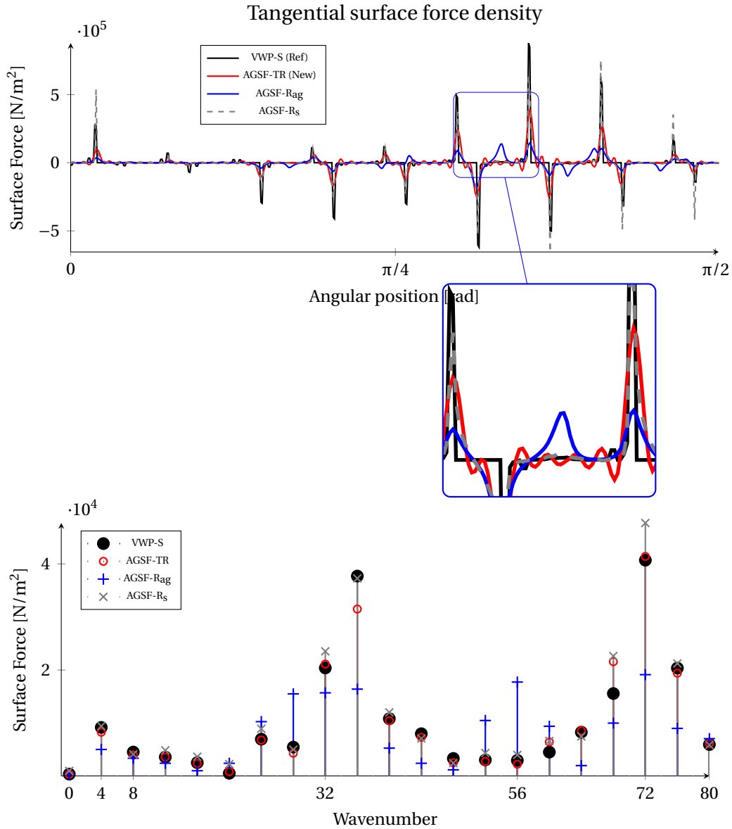
Figure 2.15 – Comparison of several methods for tangential surface force density using air-gap MST and VWP for SCIM topology.
