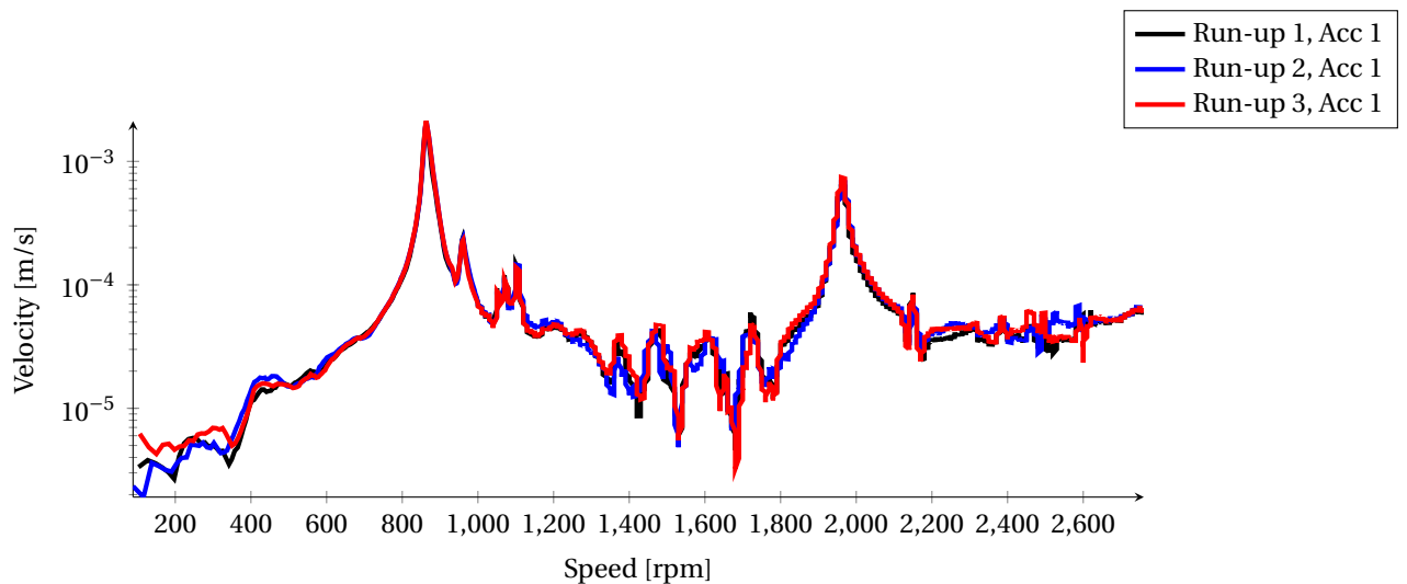
Figure B.8 – One accelerometer measurement for 3 different run-up at 10f_s .
