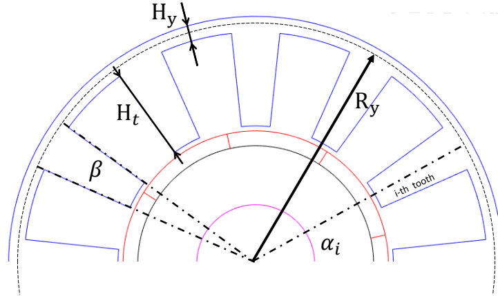
Figure 1.23 – Geometrical notations.
