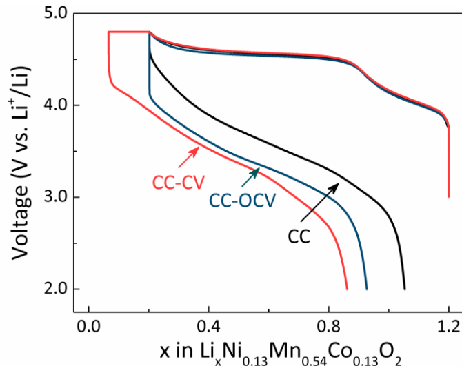
Figure III. 13 The first charge-discharge voltage curves of \text{Li}_{1.2}\text{Ni}_x\text{Ni}_{0.13}\text{Mn}_{0.54}\text{Co}_{0.13}\text{O}_2 cycled with different protocols. One cell was charged to 4.8 V and then directly discharged to 2.0 V, denoted as CC (black line), whereas an intermediate OCV step for 120 h (blue line, denoted as CC - OCV) or CV hold for 8 h (red line, denoted as CC - CV) was respectively imposed to the other two cells. All the cells were cycled at C/3.
