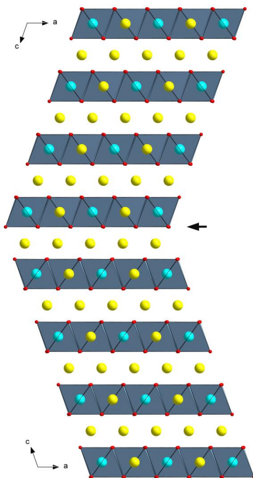
Figure III. 7 Tentative model of twins in the O3 R\bar{3}m structure. Two twinned domains viewed along [010] possess mirror-related orientation of the c -axis. At the twin plane the “cubic” ccp close packing of the O atoms is interrupted by a single “hexagonal” h layer (marked with an arrow). The M cations, Li cations and O atoms are shown as cyan, yellow and red spheres, respectively. The MO_6 octahedra are shaded.
