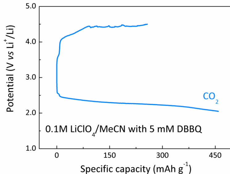
Figure A. 4. 9 Galvanostatic discharge-charge curve in 0.1 M \text{LiClO}_4/\text{MeCN} with the addition of 5 mM DBBQ under \text{CO}_2 in a two-compartment “oraha” cell with a ceramic membrane to prevent the crossover of quinones.
