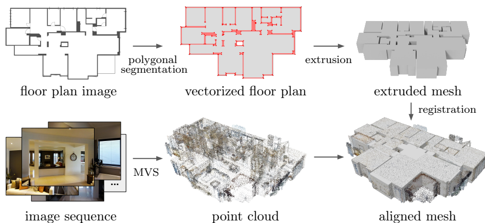
Figure 5.1: Overview of our pipeline. The floor plan image is first converted to a vectorized form, where the interior region is indicated in gray. The 2.5D model is generated by extruding polygons corresponding to the interior region given an estimated height. Finally, the model is registered to the point cloud, computed from the image sequence, to output an aligned model.
