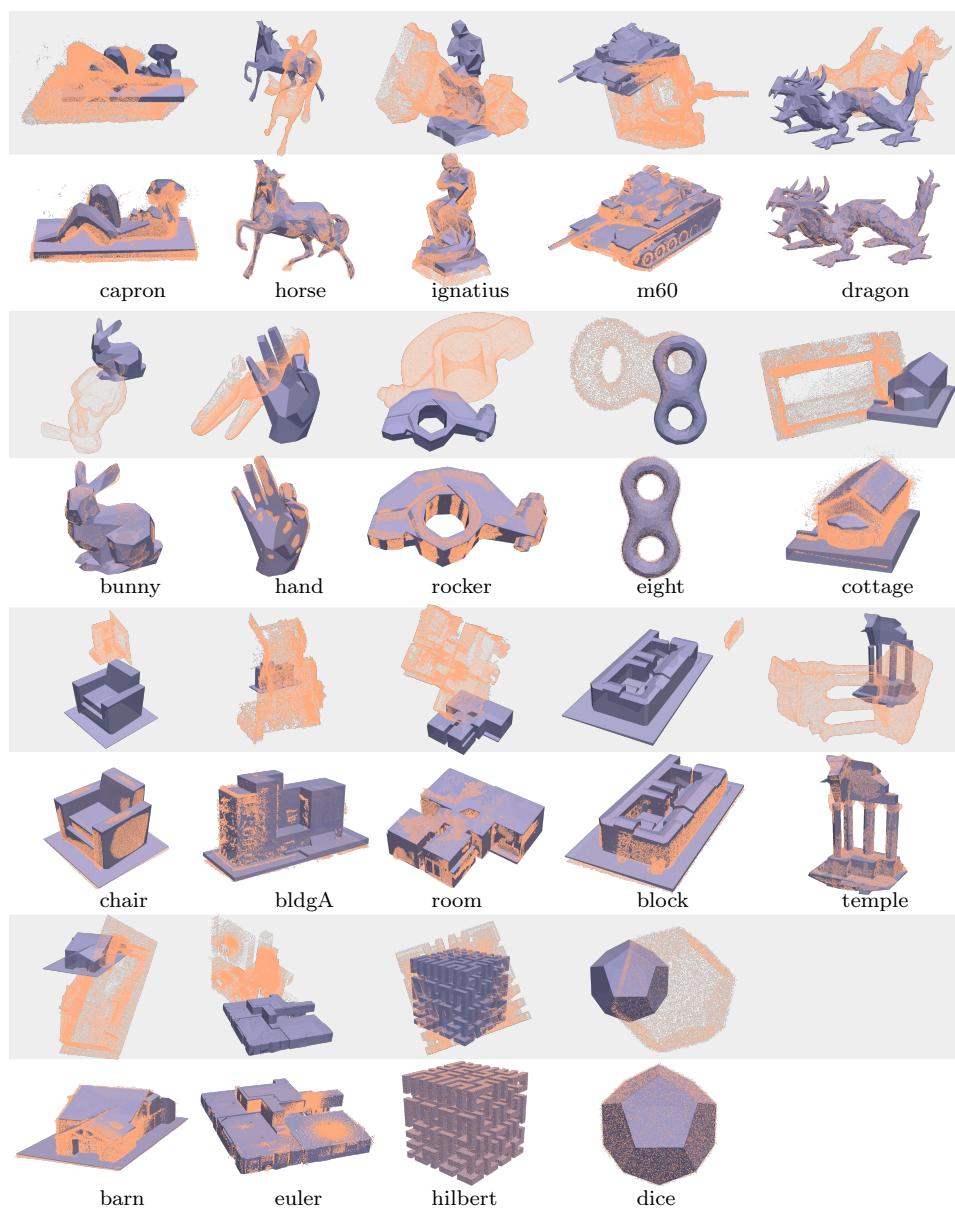
Figure 4.4: Visualization of our results on 19 examples from the dataset, with random perturbations in rotation between 90^\circ and 180^\circ , in translation between 0 and 100% of the diameter, and in scaling between 0.25 and 2. Regular objects are shown after free-form objects. For each example, the input point cloud and mesh are shown on the top (gray region), with the alignment output at the bottom.
