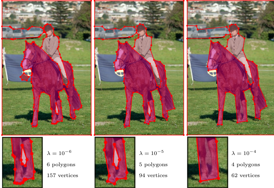
Figure 3.2: Trade-off between fidelity to data and complexity to output polygons. Increasing \lambda gives more compact, yet less accurate, output polygons. Objects of interest: horses, persons and cars.
