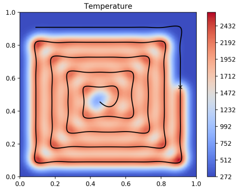
Figure 2.10: Exterior spiral path at time t=0.87 .
