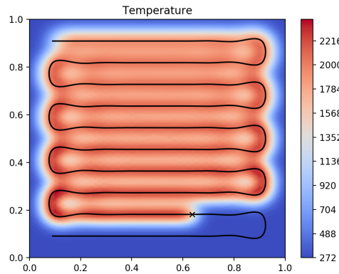
Figure 2.8: Basic path at time t = 0.87 .
