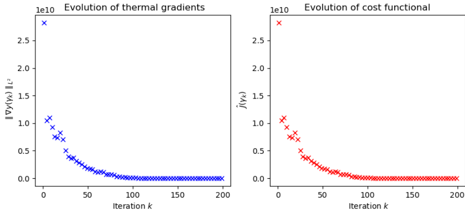
Figure 2.14: Evolution of thermal gradients and cost functional
