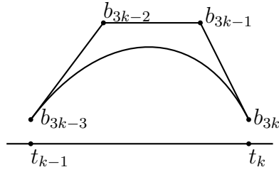
Figure 2.15: Bézier curve on [t_{k-1}, t_k]
