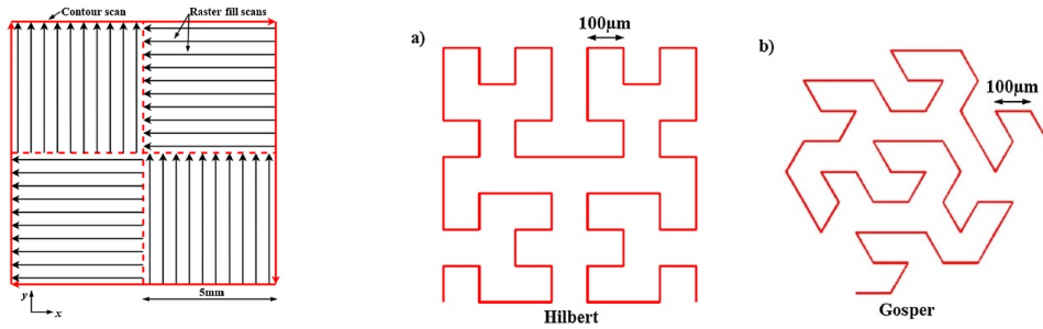
Figure 2.5: Illustration of island scan control sample and scan strategies generated using (a) Hilbert and (b) Peano-Gosper mathematical space filling curves as studied in [11].
