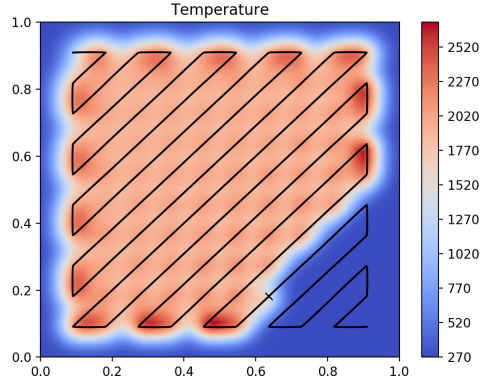
Figure 2.11: Zigzag path at time t = 0.87 .
