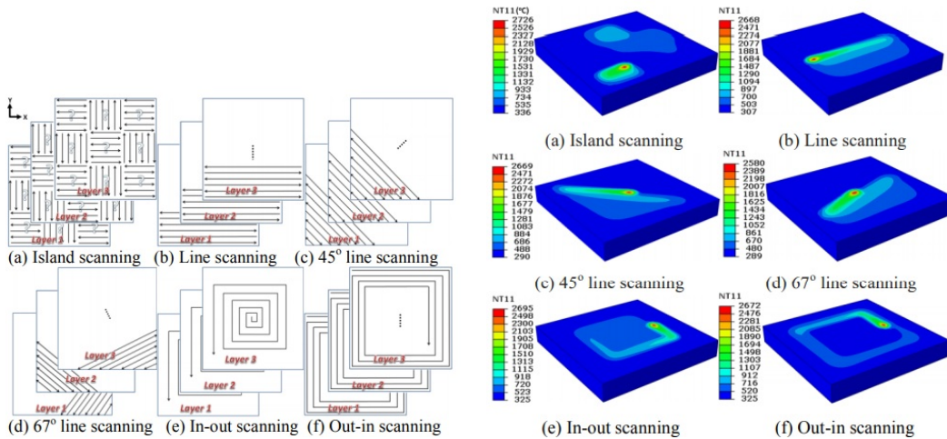
Figure 2.3: The different laser paths studied in [12].
