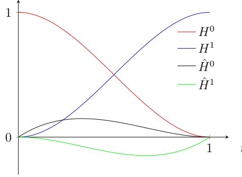
Figure 2.7: Hermite basis functions.
