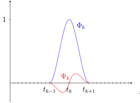
Figure 2.12: Hermite element finite basis functions.
