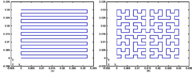
Figure 2.4: S scanning pattern and fractal scanning pattern based upon Hilbert curve studied in [37].
