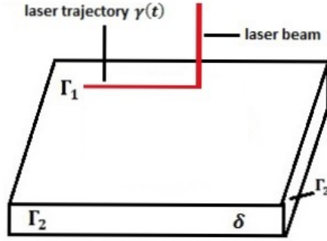
Figure 2.1: One layer \Omega of thickness \delta with boundary \Gamma = \overline{\Gamma_1} \cup \overline{\Gamma_2} \cup \overline{\Gamma_3} .
