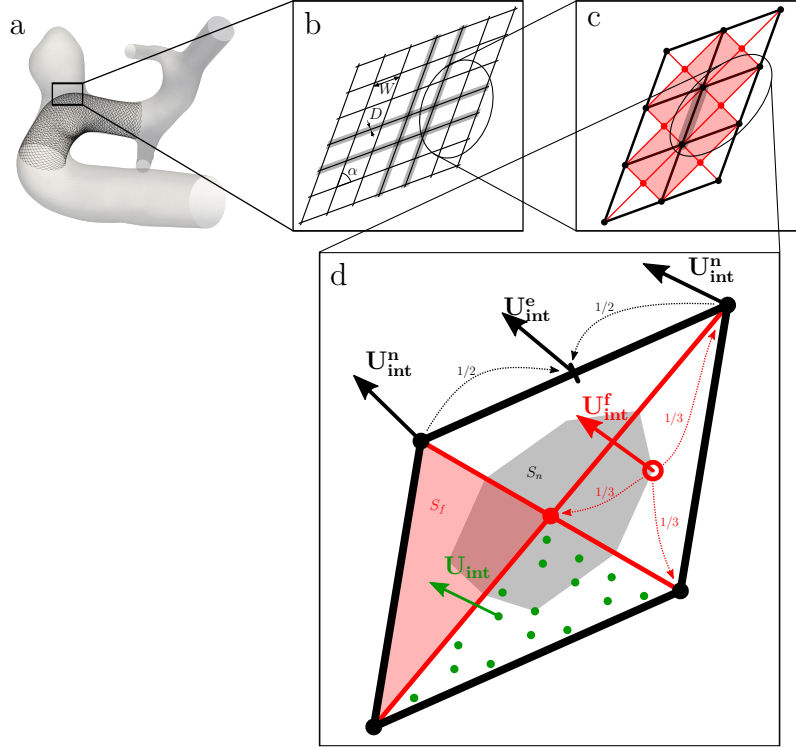
Figure 3.1: Device data structure. a : Aneurysm with deployed endovascular flow-diverter. b : Wires neutral fibre representation output from mechanical deployment. Only a few cylinders envelopes of diameter D have been coloured in grey for illustration purposes. c : Triangles are constructed using original wire-wire intersection points (in black) and the inserted barycentric points (in red). Cells in transparent red are involved in the velocity interpolation for the edge highlighted in grey. Only real cylinders locations (black edges) are used to apply volume forces on the fluid to mimic wires impact on the flow. d : Points used to interpolate velocities for one triangle cell are represented in green. Cell-to-points and points-to-edge redistributions are also indicated by dotted arrows with the corresponding coefficients.
