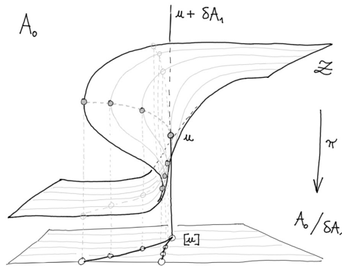
Figure 6.1: A cuspidal singularity of the projection \mathcal{Z}(X) \rightarrow A_0(X)/\delta A_1(X) . Vertical lines represent classes of homologous potentials, some of which intersect the stationary surface more than once.
