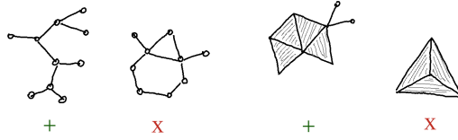
Figure 6.2: retractable hypergraphs (+) and other ones (x).
