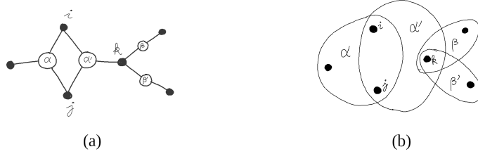
Figure 1: (a) factor graph and (b) hypergraph representations of X \subseteq \mathcal{P}(\Omega) .
