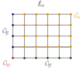
Figure 2.2: Spectral decomposition \hat{E}_\alpha = \bigsqcup_{\beta \subseteq \alpha} \hat{G}_\beta .
