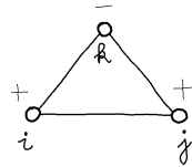
Figure 6.3: A triangle of binary variables.
