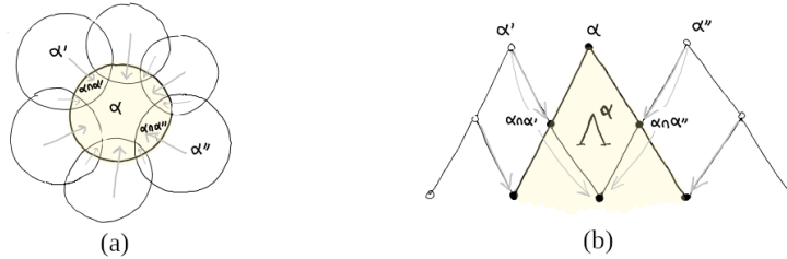
Figure 2.1: X \subseteq \mathcal{P}(\Omega) illustrated as (a) a Venn diagram and (b) a semi-lattice. The colored region represents \Lambda^\alpha = \{\beta' \subseteq \alpha\} while arrows represent some of the flux contributions to the Gauss formula \sum_{\beta' \in \Lambda^\alpha} \delta\varphi_{\beta'} = \sum_{\alpha' \beta' \in d\Lambda^\alpha} \varphi_{\alpha' \beta'} .
