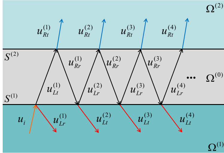
Figure 4.4: A simple double interface model. The incident wave u_i passes through the two interfaces \mathcal{S}^{(1)} and \mathcal{S}^{(2)} from bottom to top, u_{Lr}^{(1)} and u_{Lt}^{(n)} ( n \geq 2 ) generated through the interface \mathcal{S}^{(1)} constitute the reflected wave u_r , and u_{Rt}^{(n)} ( n \geq 1 ) through the interface \mathcal{S}^{(2)} constitute the transmitted wave u_t .
