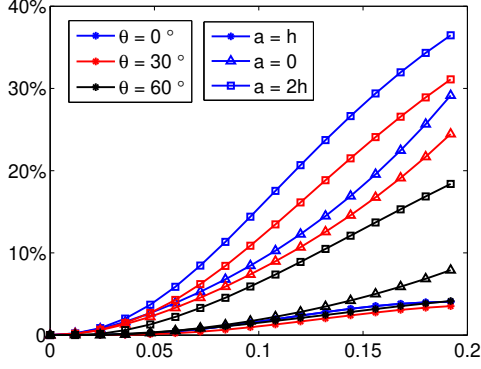
(a) Reflection coefficient errors \mathcal{R}_{Err}
