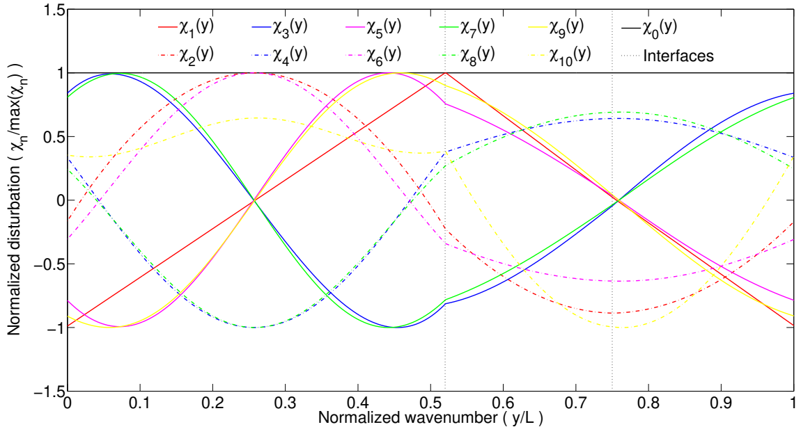
Figure 3.2: 1D polynomial approximation function \mathcal{X}_n (up to order 10).
