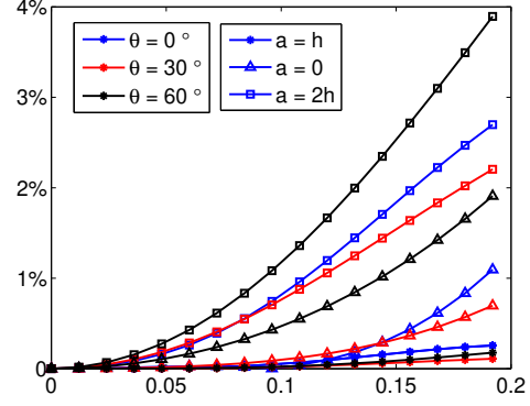
(b) Transmission coefficient errors \mathcal{T}_{Err}
