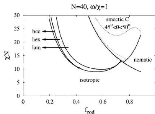
Figure 9. Phase diagram with N = 40 , and \mu/\chi = 1 . 52
