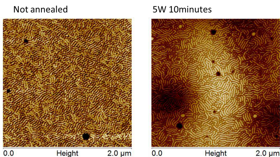
Figure S8. AFM images of MBM films made on silicon substrate from drop casted dichloromethane solution (5 g/L, film thickness 1500 nm ). The left image shows the film without any annealing and the right one presents the film annealed at 5W during 10 minutes. We first tried an annealing for 1 minute at 5W but the structuration didn't change. Then we increased the irradiation time to 5 and even 10 minutes but we couldn't obtain perpendicular cylinders. These continuous films were produced to compare with porous honeycomb films.
