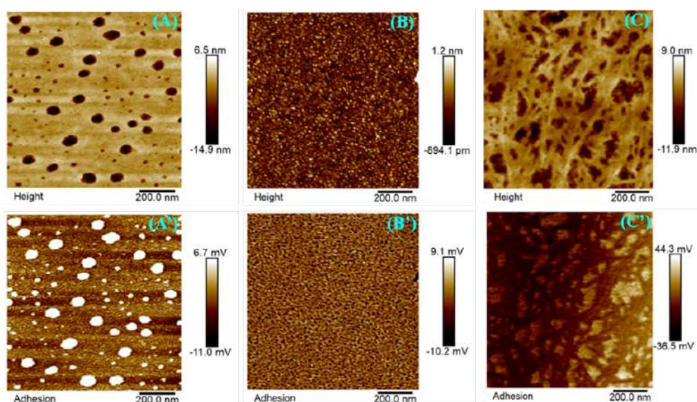
Figure 5. PeakForce QNM-Mode AFM images of diblock copolymer films were prepared by dip coating method with the withdraw speed was 10 μm/sec at room temperature. Films realized from a solution of P3HT 5K - b -PMMA 10K at (A) 1 g.L -1 , (B) 3 g.L -1 and (C) 5 g.L -1 in chloroform at ambient temperature.
