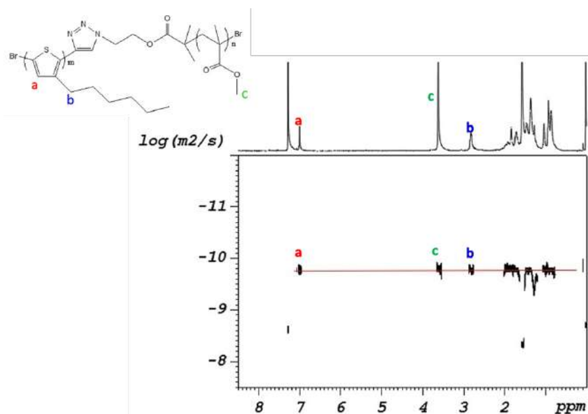
Figure S3. 1 H DOSY NMR spectrum of P3HT 16KK -b-PMMA 10K .
