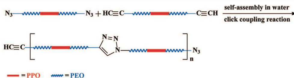
Scheme 9. Synthesis of (PEO- b -PPO- b -PEO) n multiblock copolymer by multiple coupling procedure using a combination of self-assembly and click chemistry in water. 117
