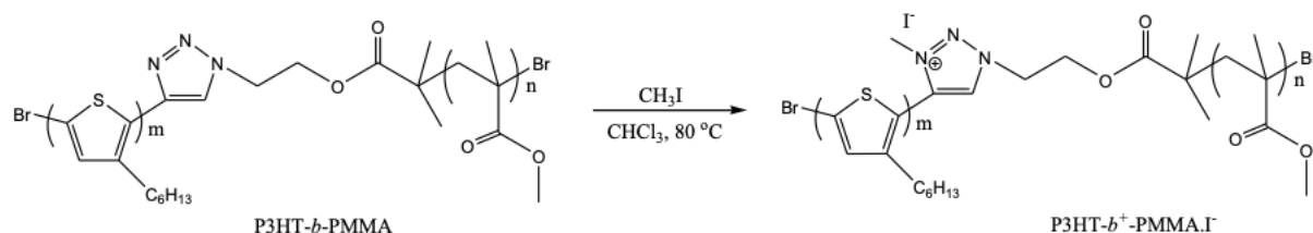
Scheme 4. Charge added of P3HT- b -PMMA by methylation reaction.
