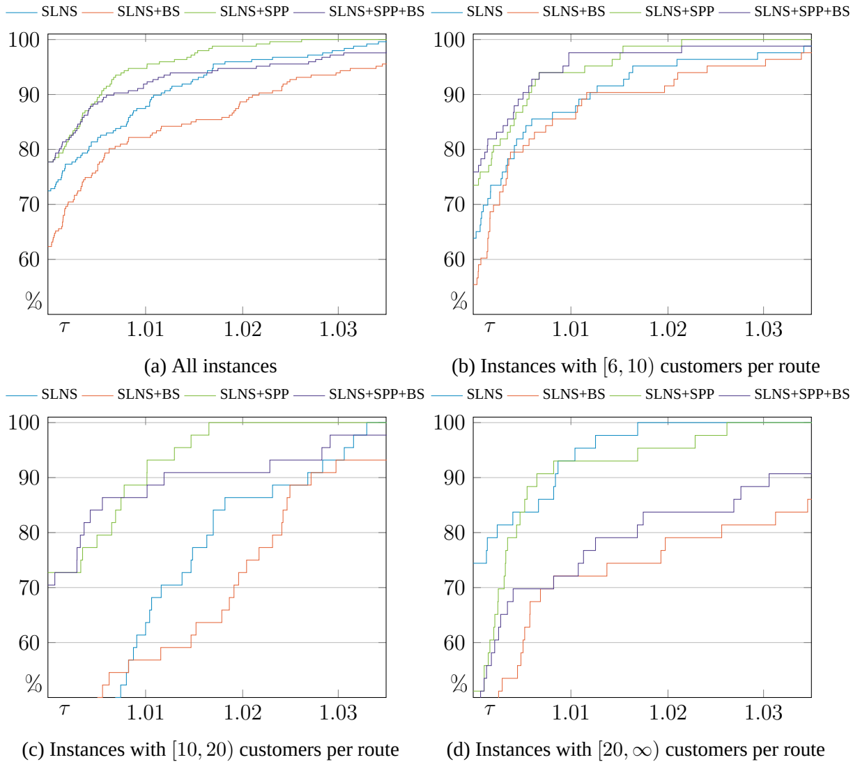
Figure 2.3 – Performance profile of the four variants, grouped by average route length
