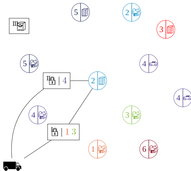
Figure 1.8 – Example of a partial solution
