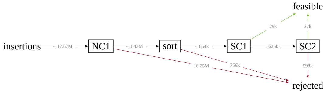
Figure 3.9 – Example of the usage of the feasibility tests
