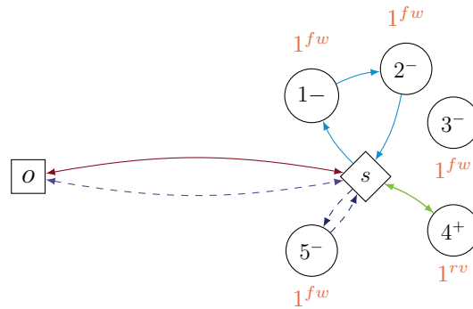
Figure 3.3 – Example for the insertion of customer 3^- in and incomplete solution
