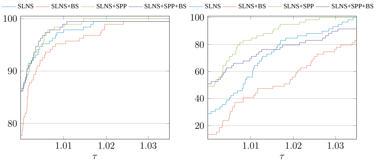
(a) All GVRPTW except VRPDO instances
