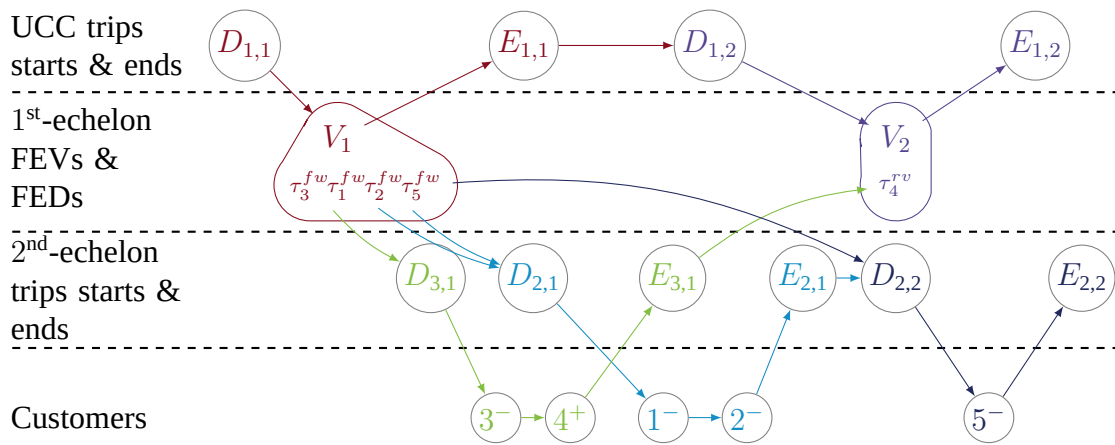
Figure 3.7 – Precedence graph of the solution of Figure 3.6 with the time schedule of Table 3.6.
