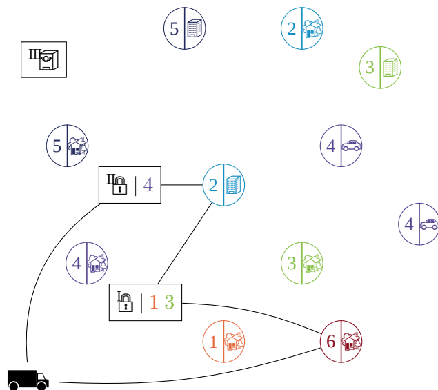
Figure 1.9 – Insertion of the brown (6) customer without lockers
