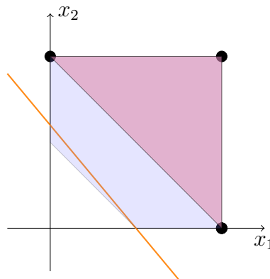
Figure 3: The set \{(x_1, x_2) \in \{0, 1\}^2 : 2x_1 + 2x_2 \geq 1\} can be relaxed using linear programming. This region K^0 includes fractional basic feasible solutions such as (1/2, 0) and (0, 1/2) . By adding new variables simulating the possible products between the variables and introducing new constraints, one obtains a larger program, but is easy to solve. Furthermore, the projection K^1 over the original space it is strictly contained in K^0 . This approach was introduced by Sherali & Adams [95]. By combining the first, third and fifth constraint at the right one can show that 2x_1 + 5x_2/3 \geq 1 holds, which cuts the point (0, 1/2) .
