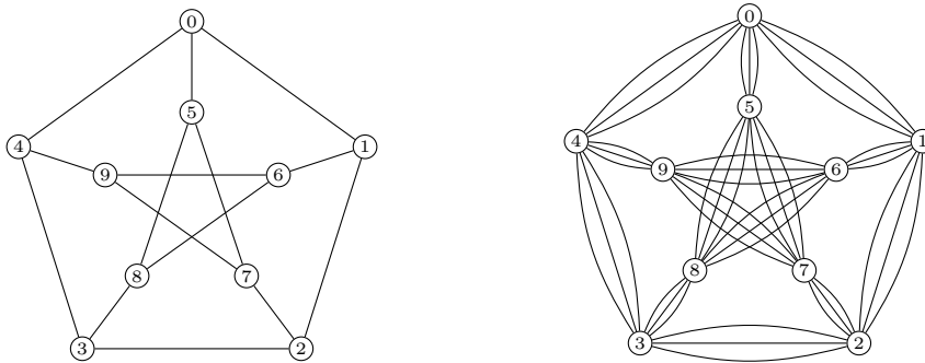
Figure 2.1: On the left, the Petersen graph G_1 . On the right, the multigraph G_3 obtained from considering 3 copies of each edge in the Petersen graph.
