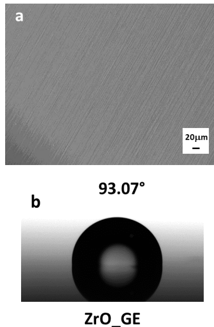
Fig. III.3 - 22 a) SEM Image and b) water contact angle of ZrO 2 _GE
