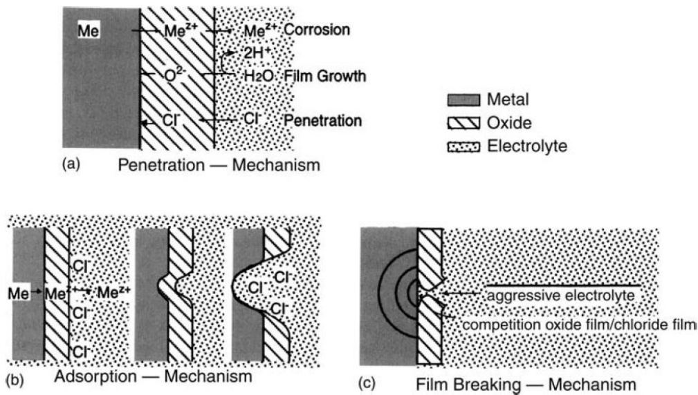
Fig. 1.2 - 5 Mechanism of break down of passive film by the presence of \text{Cl}^- and introduced pitting corrosion 31
