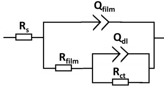
Fig. IV.2 - 5 Electrochemical Equivalent Circuit of 316L bare substrate immersed in NaCl
