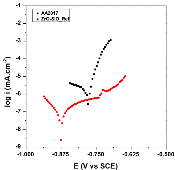
Fig. IV.3 - 4 Potentiodynamic Polarization curves of AA2017 substrate and ZrO-SiO_Ref after 24 hours of immersion in NaCl 30g/L
