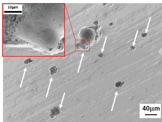
Fig. IV.3 - 6 Surface morphology of ZrO-SiO_Ref after 1 weeks of immersion (White arrows indicating the delamination, red rectangle indicating zoomed region of corroded site)
