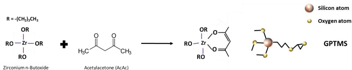
Fig. II.3 - 2 Scheme of the AcAc blocking active sites on Zirconium n-Butoxide and the precursors of ZrO-SiO
