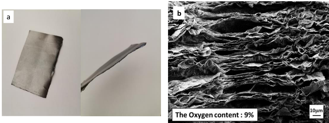
Fig. III.2 - 2 a) The photo of Graphite foil before electrochemical expanding b) and after
