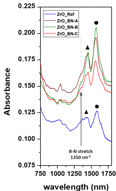
Fig. III.3 - 7 The FTIR/ATR spectroscopy of ZrO deposited coatings with or without three BNNS fillers
