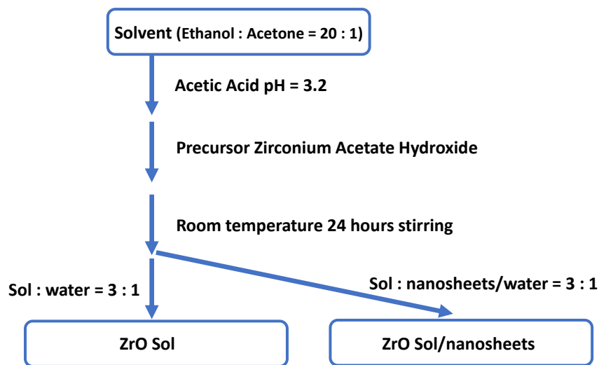
Fig. II.3 - 1 Scheme of preparation procedure for ZrO Sol
