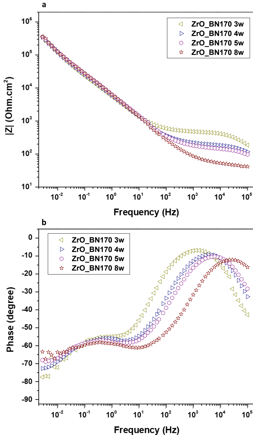
Fig. IV.2 - 32 Bode curves of ZrO 2 /BN170 at 3, 4, 5 and 8 weeks of immersion a) Impedance curves and b) Phase curves
