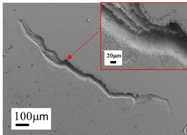
Fig. IV.2 - 3 SEM image of the morphology of 316L bare substrate after the polarization
