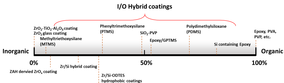
Fig. I.4 - 3 Classification of hybrid coatings with the x-axes showing the ratio of organic compound in the coatings
