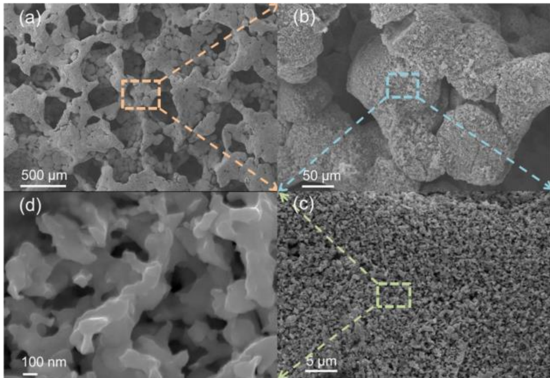
Fig. I.2 - 6 SEM images of porous structure synthesized by dealloying-redealing method done by Zhu et al with different magnifications a) 40 b) 300 c) 3000 d) 30,000 16
