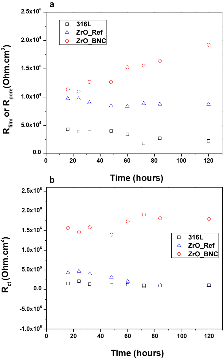
Fig. IV.2 - 22 The evolution of EIS fitting parameter value over 120 hours of the three samples a) R_{\text{film}} or R_{\text{pore}} , b) R_{\text{ct}}
