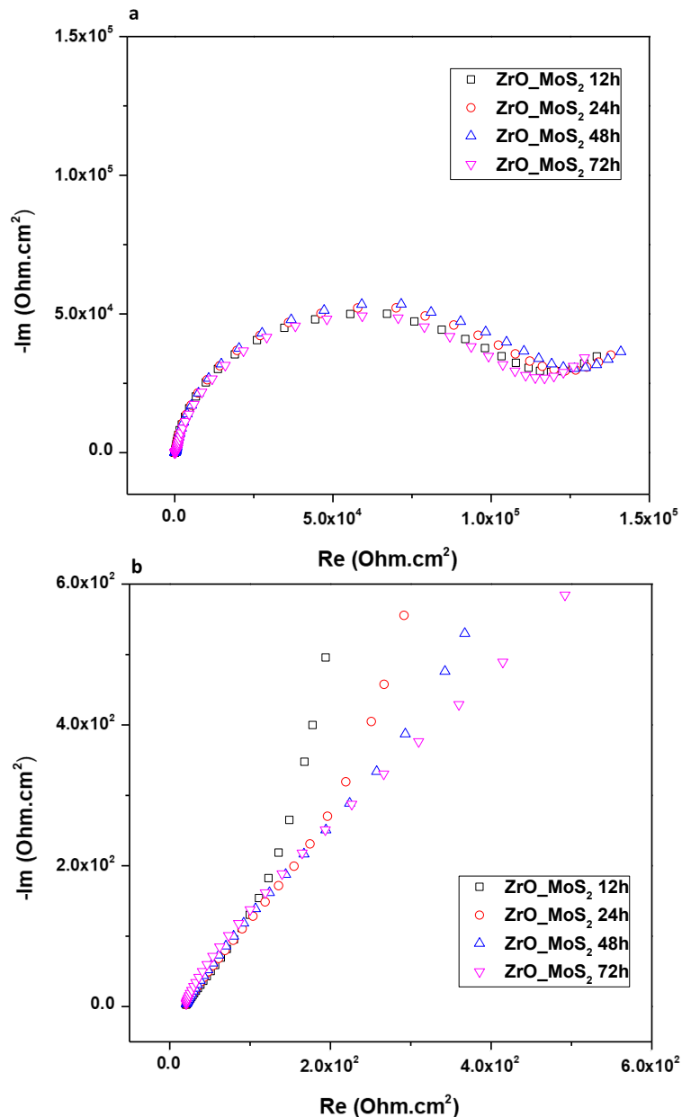
Fig. IV.5 - 9 a) Nyquist curve and b) zoomed region at high frequency of EIS tests of ZrO_MoS 2
