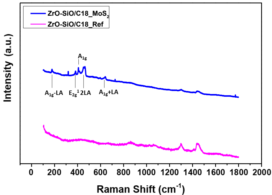
Fig. III.3 - 30 Raman shift of all ZrO 2 -SiO 2 /C18_Ref and ZrO 2 -SiO 2 /C18_MoS 2 deposited carbon steel samples
