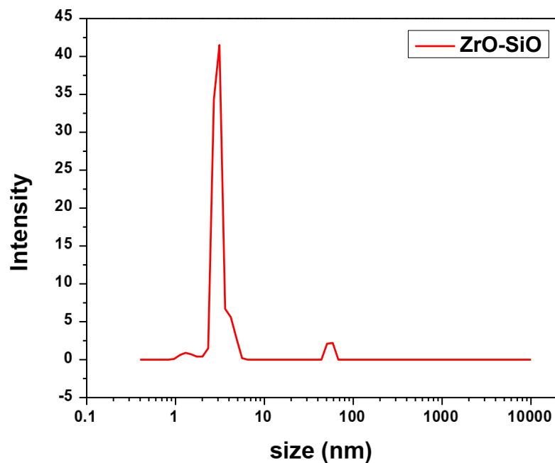
Fig. III.3 - 11 DLS of ZrO-SiO Sol-Gel solution after synthesis
