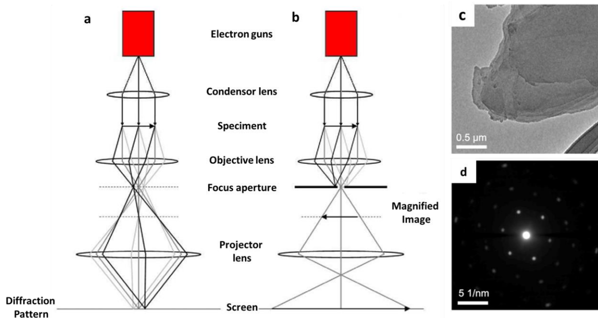
Fig. A - 8 Scheme of TEM a) Diffraction Pattern Mode and b) Magnification Image Mode ; 5 the Image of c) Magnified image and d) Diffraction Pattern 6
