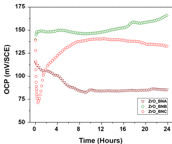
Fig. IV.2 - 16 OCP of three different BNNS charged ZrO coated samples in 24 hours of immersion in NaCl 30g/L solution
