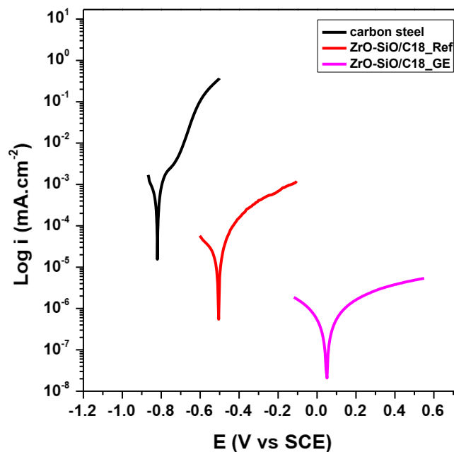
Fig. IV.5 - 10 Polarization curve of ZrO-SiO/C18_GE superposed with reference samples after 24 hours immersed in NaCl 30g/L
