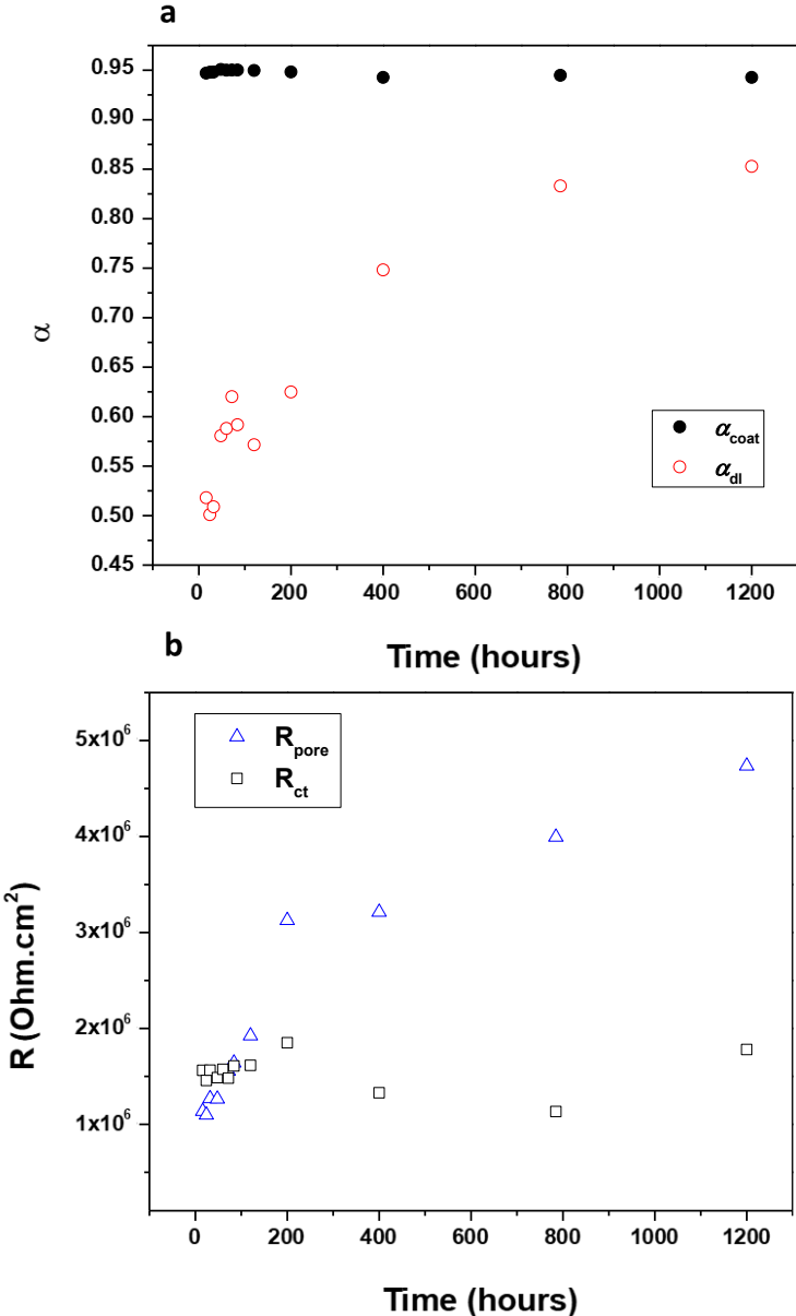
Fig. IV.2 - 23 The evolution of ZAH_BNC of a) \alpha_{coat} and \alpha_{dl} values and b) R_{pore} and R_{ct} values over 1200h
