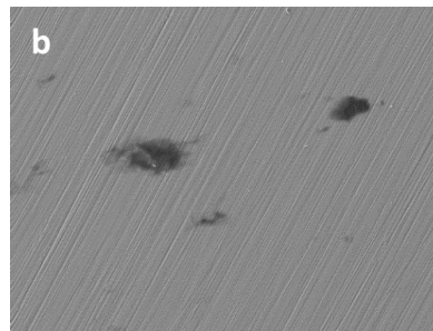
Fig. IV.5 - 4 a) Nyquist curve of ZrO_GE and b) SEM image of surface morphology of ZrO_GE after 5 weeks of immersion
