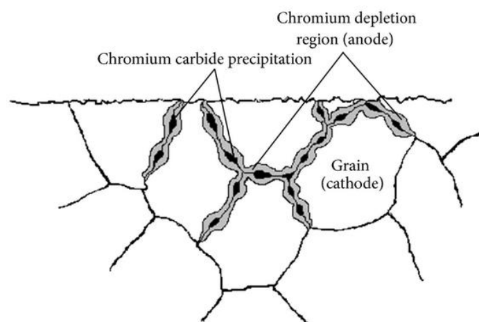
Fig. I.2 - 7 Mechanism of intergranular corrosion 18
