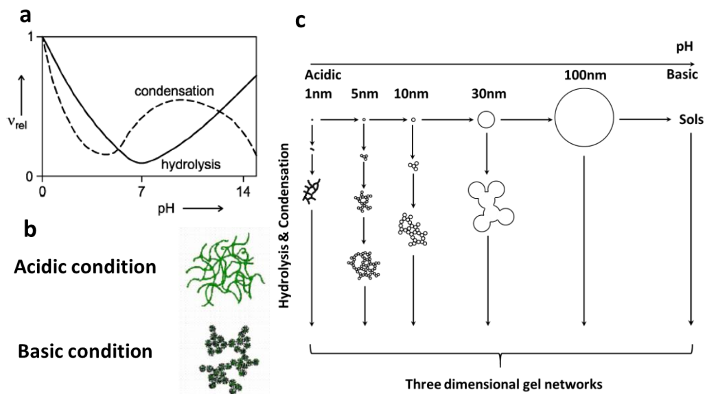
Fig. I.3 - 4 Influence of pH to the microstructure a) the figure of the reaction speed of hydrolysis and condensation influenced by pH b) particles size influence by pH c) the shape of the final product influenced by pH (reform from the work of Pandey et al.) 83,101 102
