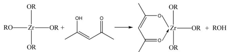
Fig. 1.3 - 5 Mechanism of chelating agent blocking precursor active sites for Zr-based precursor and diketone 103
