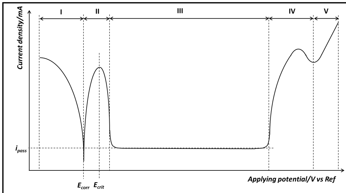
Fig. I.2 - 3 Typical Electrochemical Dynamic Polarization curve of a passive material 11
