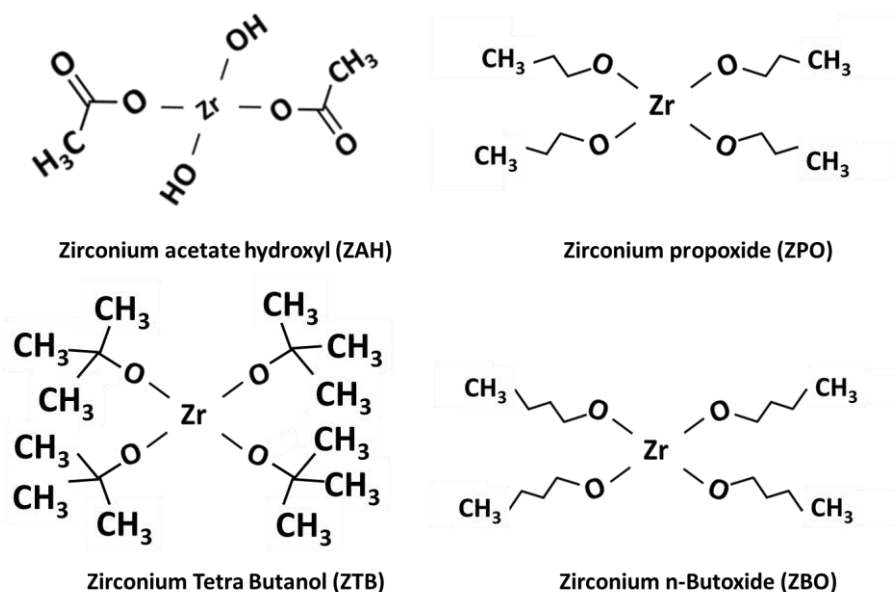
Fig. 1.3 - 3 Four different Zirconium based precursors
