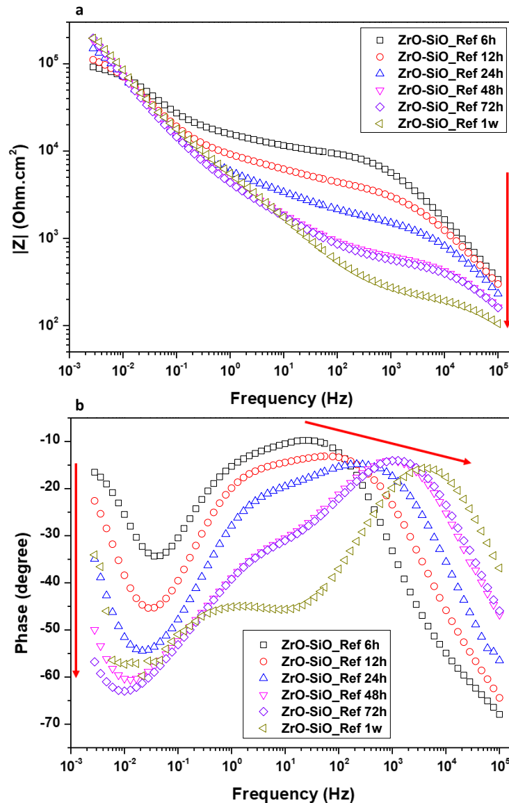
Fig. IV.3 - 5 Bode a) Impedance curves and b) Phase curves of ZrO-SiO 2 _Ref in 1 weeks of immersion in NaCl 30g/L solution
