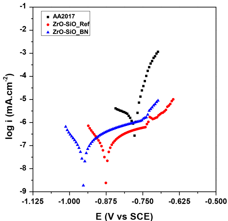
Fig. IV.3 - 7 Potentiodynamic polarization curve for ZrO-SiO_BN superposed with AA2017 substrate and ZrO-SiO_Ref
