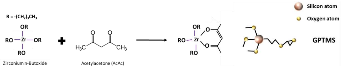
Fig. II.3 - 2 Scheme of the AcAc blocking active sites on Zirconium n-Butoxide and the precursors of ZrO-SiO
