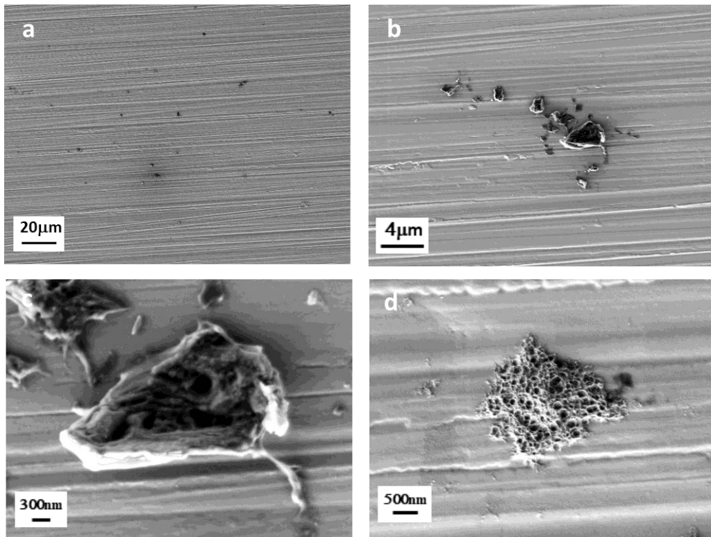
Fig. IV.5 - 8 SEM images of surface morphology of ZrO 2 -MoS 2 after 24 hours of immersion in NaCl solutions
