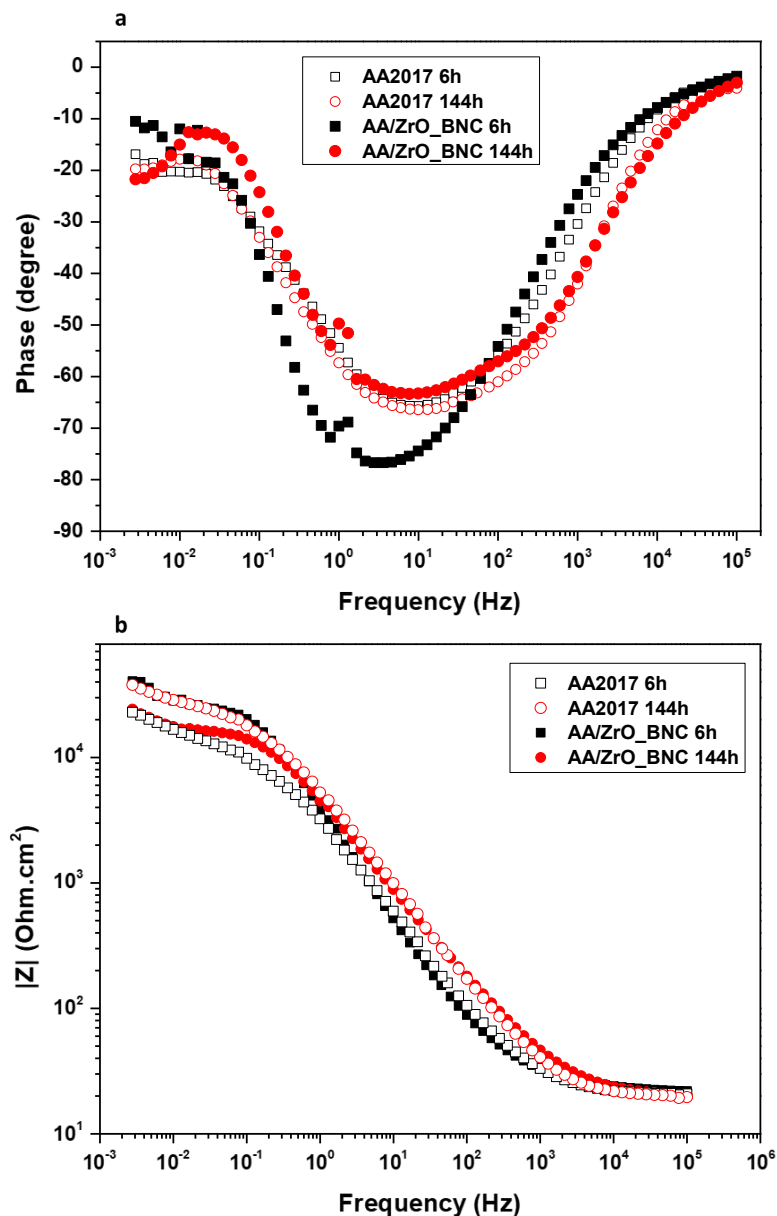
Fig. IV.3 - 3 Bode a) Phase and b) Impedance curves of comparison between AA2017 substrate and AA/ZrO 2 -BNC at 6 hours of immersion and 144 hours of immersion in NaCl 30g/L solution
