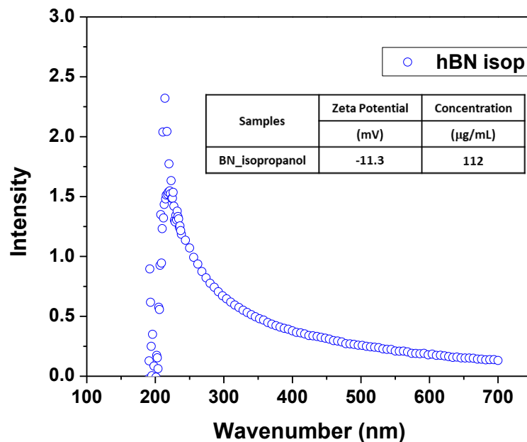
Fig. III.3 - 13 UV-Visible spectroscopy of BN-C exfoliated in isopropanol with inset table showing the parameters of the solution
